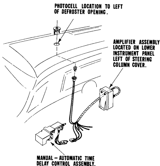
Figure 9G-1 - Twilight Sentinel Components - Typical Installation - Past Models
