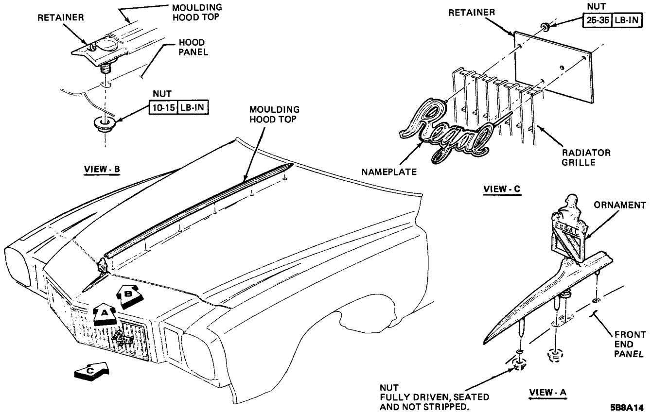
Figure 8A-14 A Series Hood Moldings
