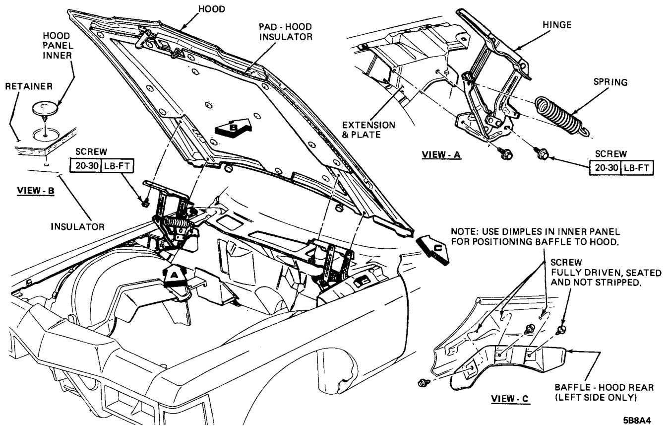
Figure 8A-4 E Series Hood
