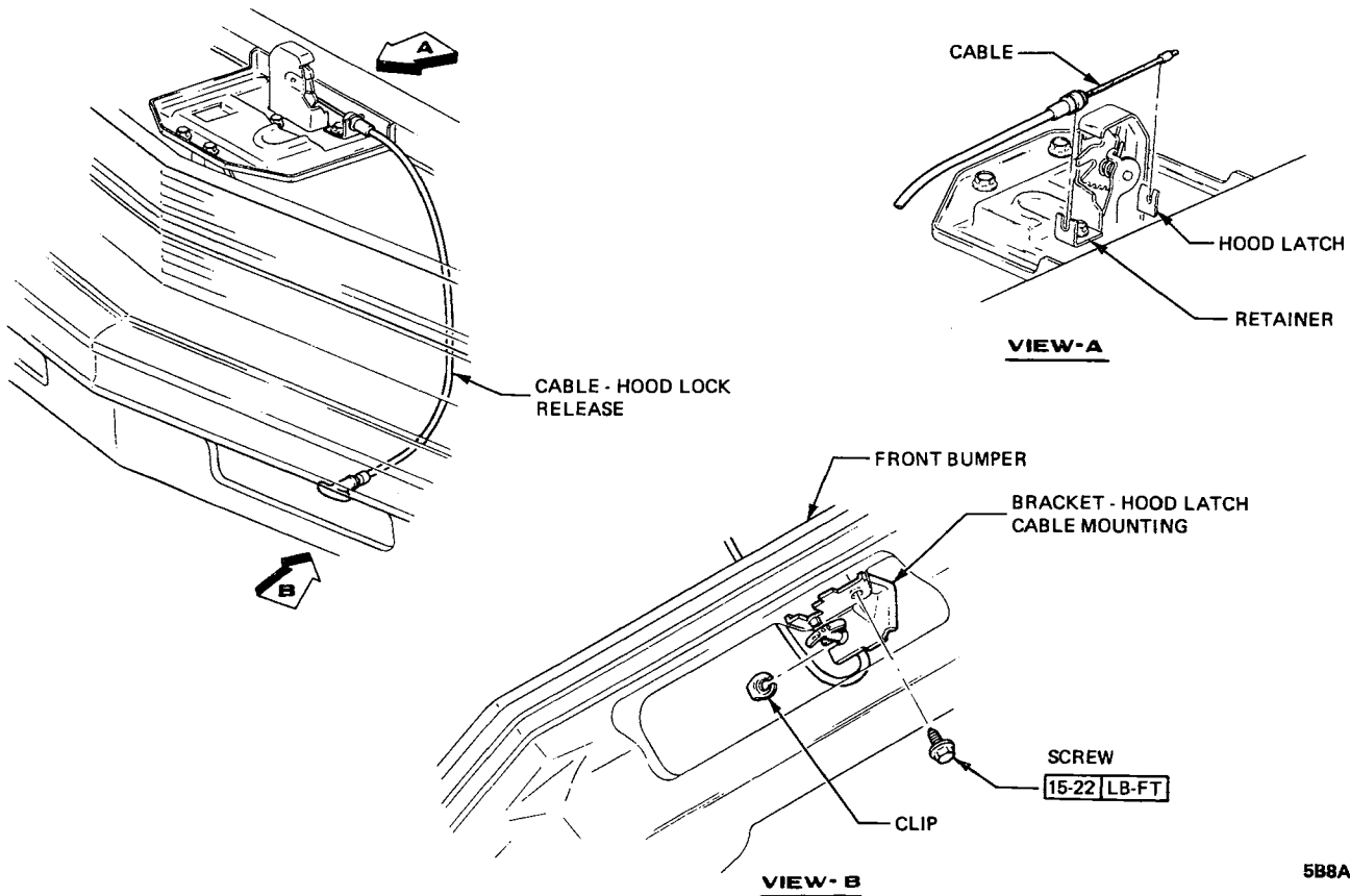
Figure 8A-7 X Series Hood Release Cable
