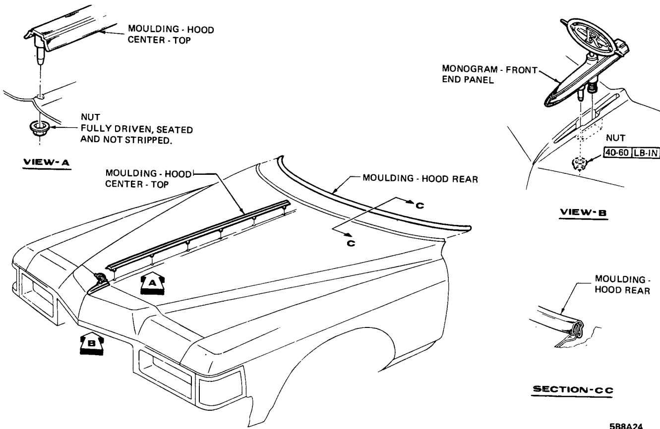
Figure 8A-24 E Series Hood Moldings
