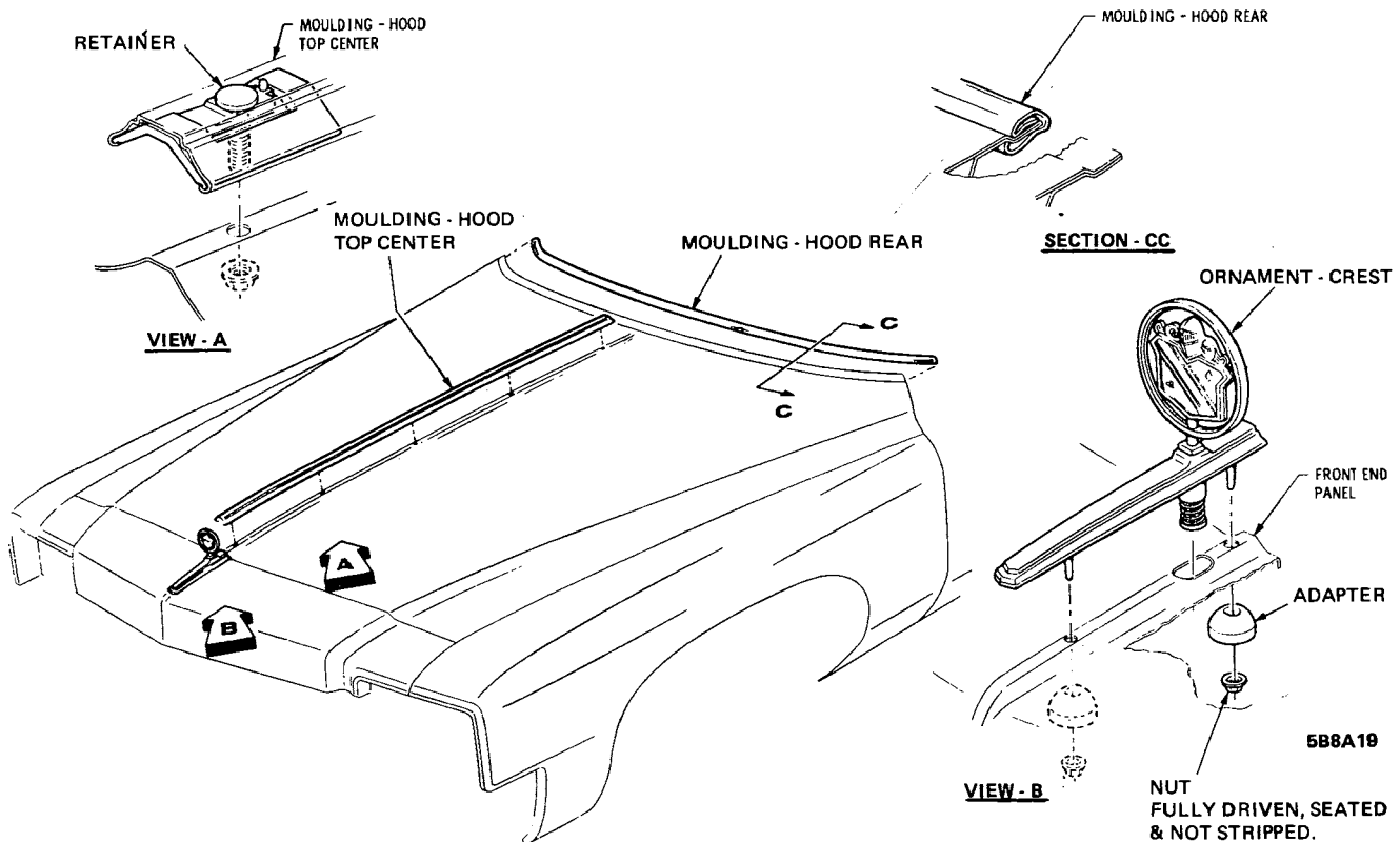
Figure 8A-19 B-C Series Hood Moldings
