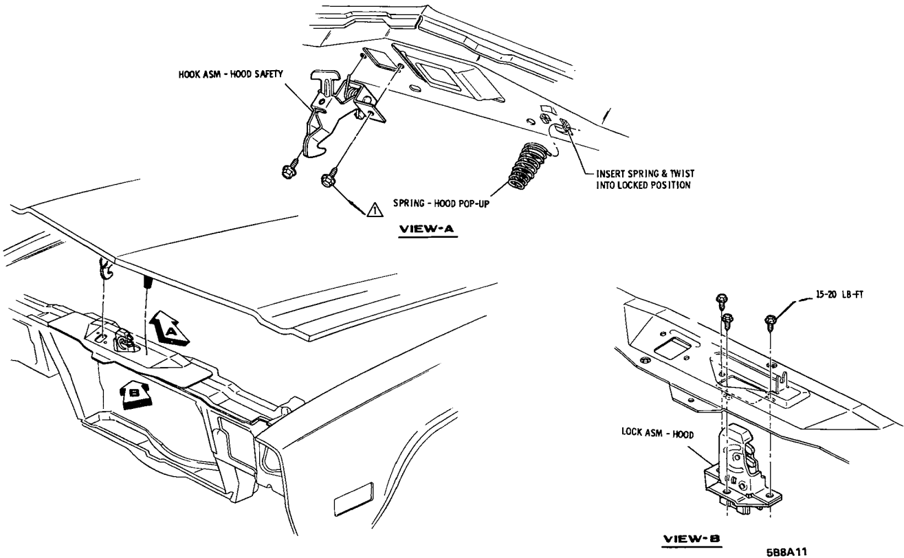
Figure 8A-11 A Series Hood Latch
