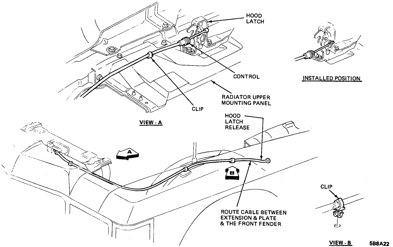
Figure 8A-22 E Series Hood Release Cable
