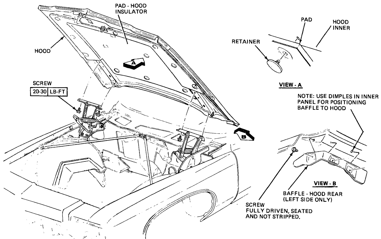
Figure 8A-2 A Series Hood
