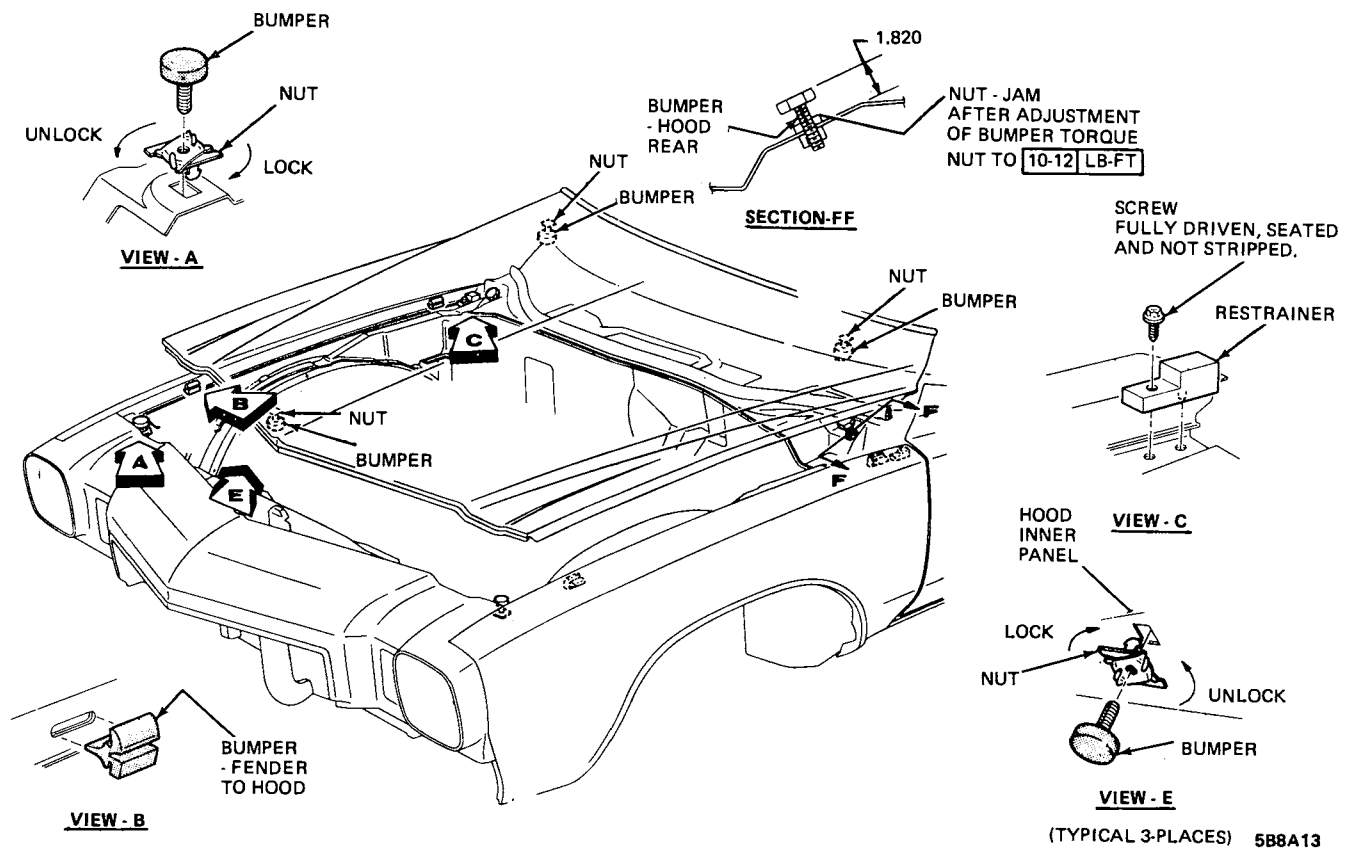
Figure 8A-13 A Series Hood Bumpers
