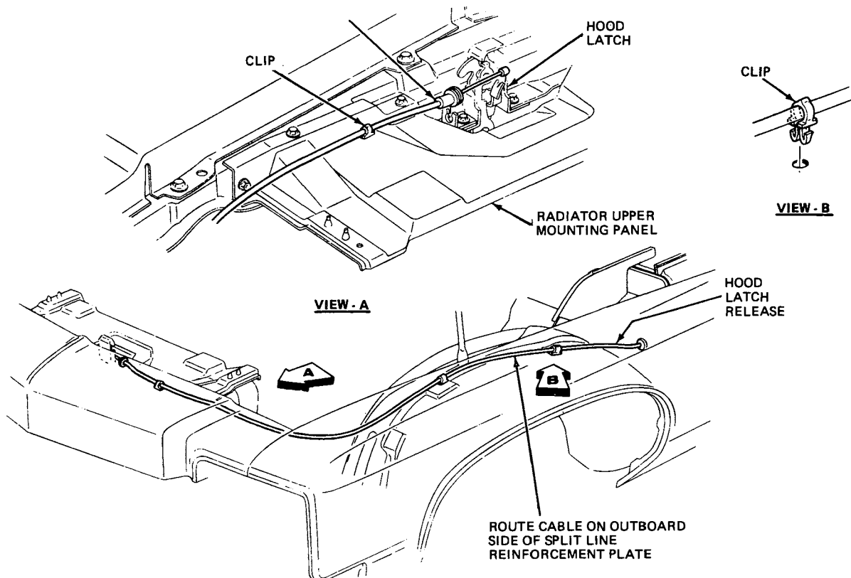
Figure 8A-17 B-C Series Hood Release Cable
