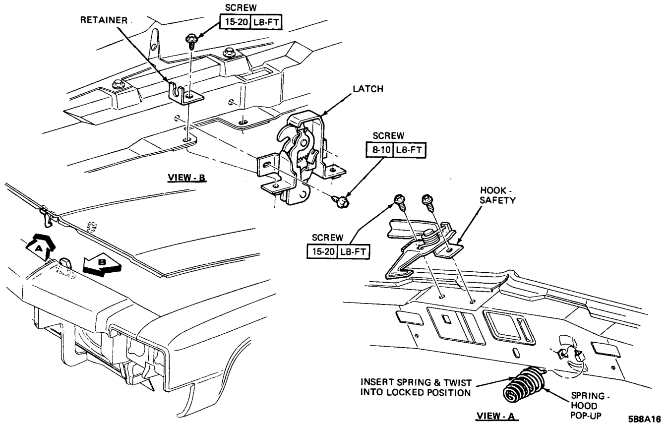
Figure 8A-16 B-C Series Hood Latch
