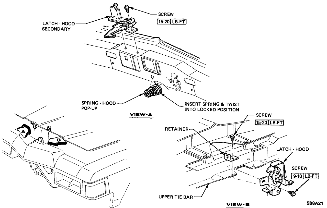
Figure 8A-21 E Series Hood Latch
