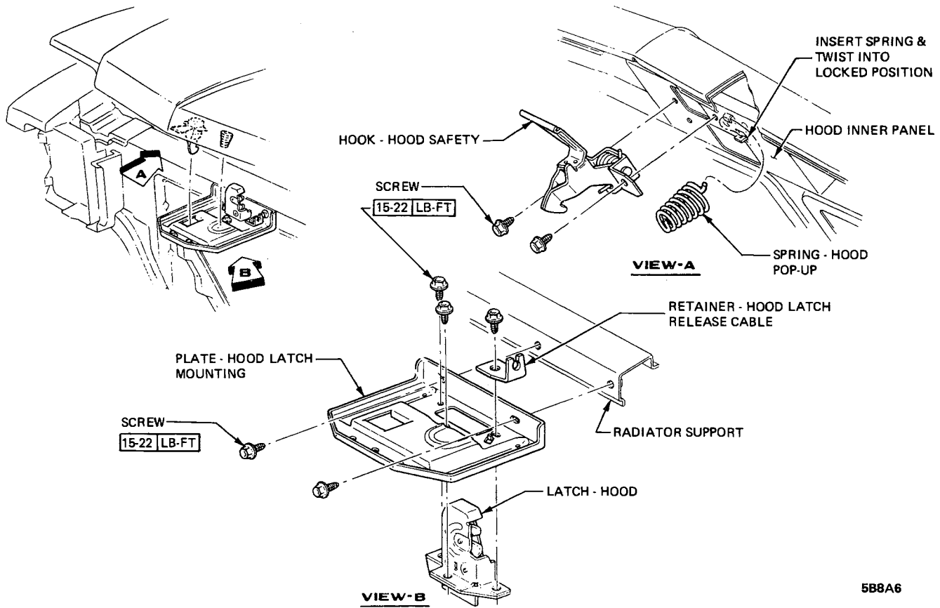
Figure 8A-6 X Series Hood Latch
