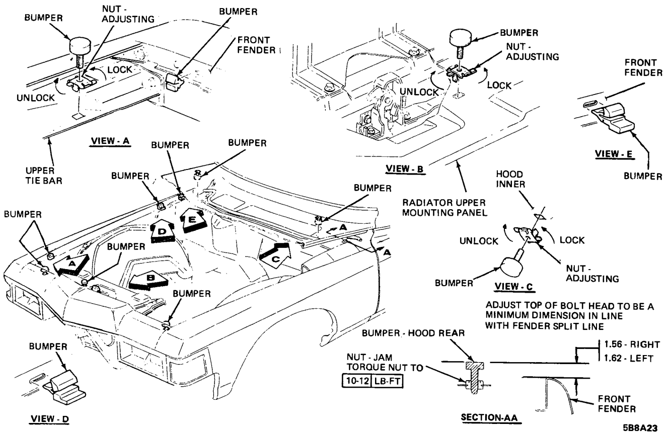
Figure 8A-23 E Series Hood Bumpers
