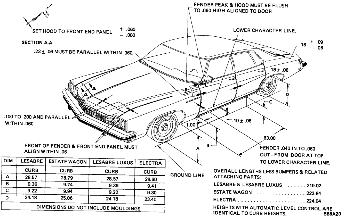
Figure 8A-20 B-C Series Hood Dimensions
