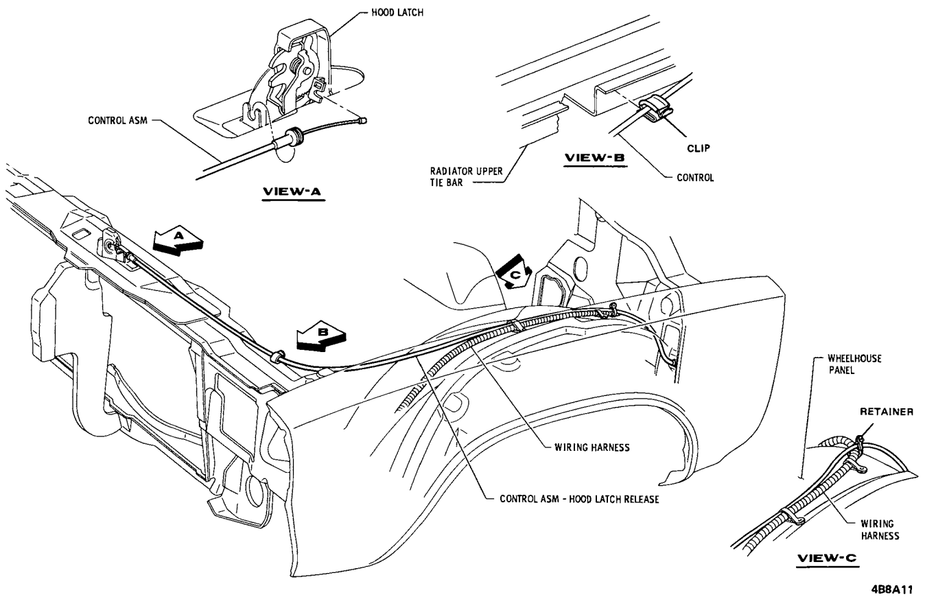
Figure 8A-12 A Series Hood Release Cable
