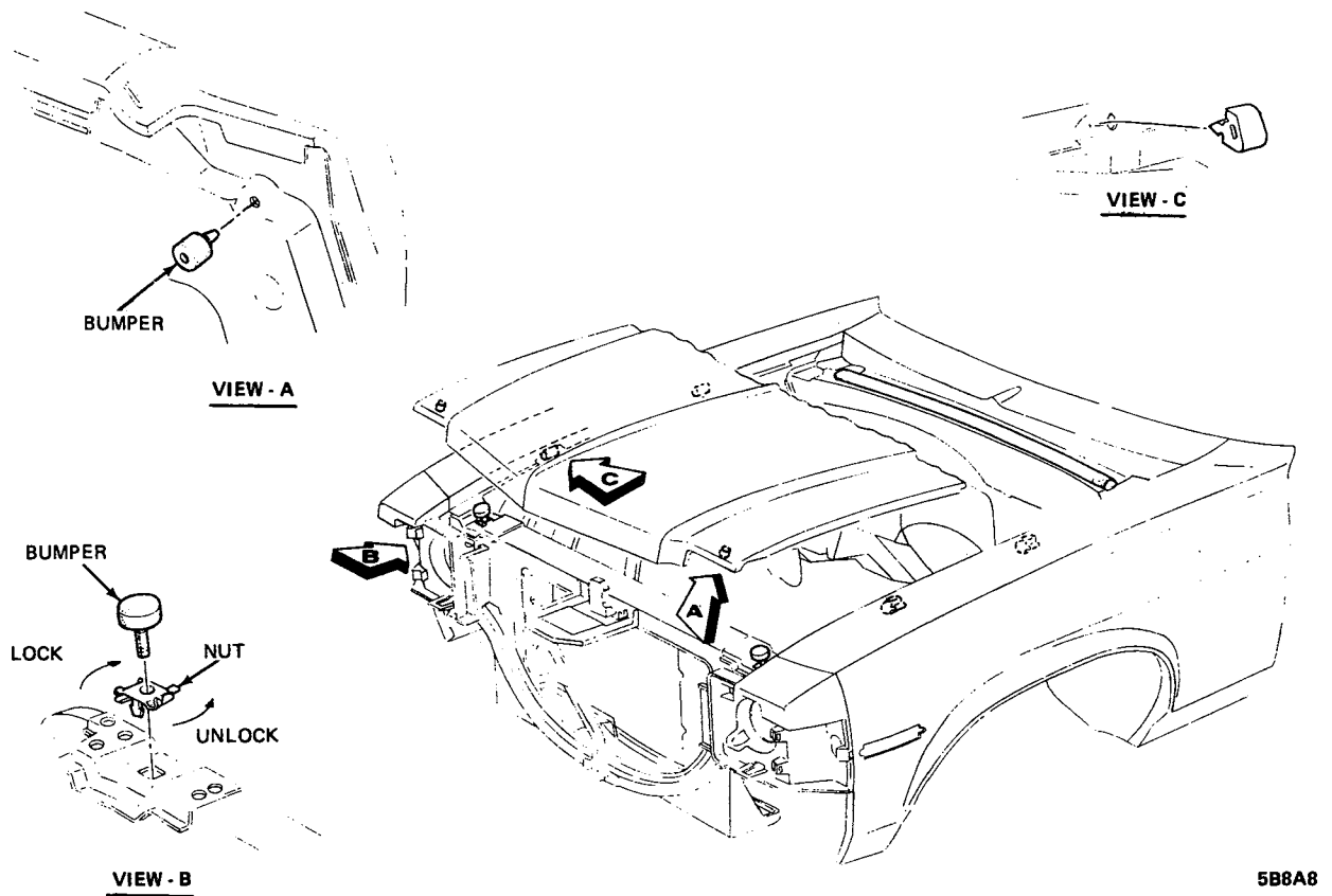
Figure 8A-8 X Series Hood Bumpers
