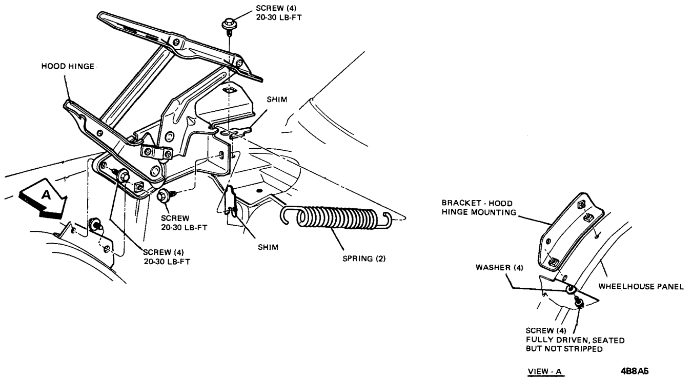
Figure 8A-5 B-C Series Hood Hinge Spring
