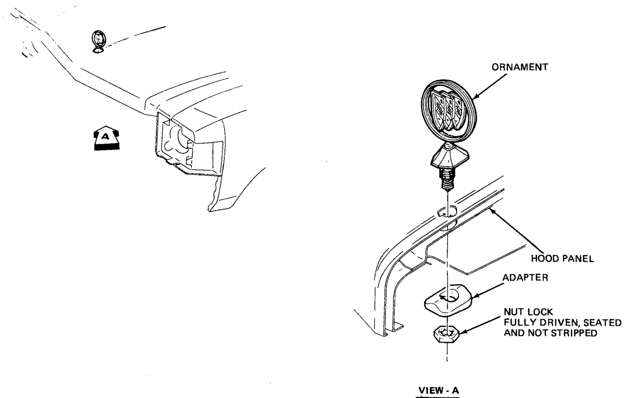
Figure 8A-9 X Series Hood Ornamentation
