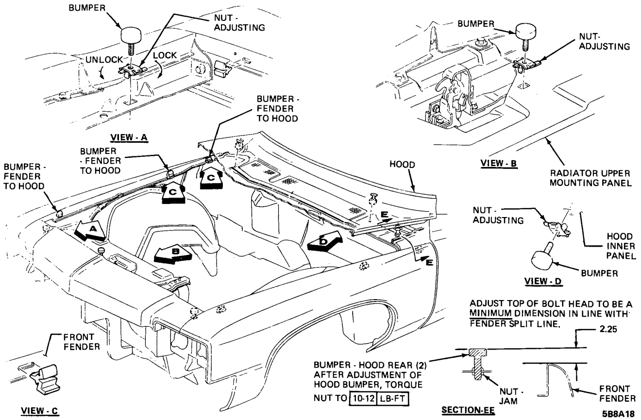
Figure 8A-18 B-C Series Hood Bumpers
