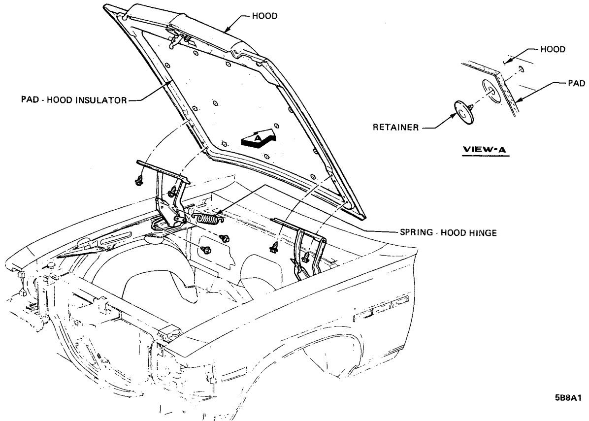
Figure 8A-1 X Series Hood
