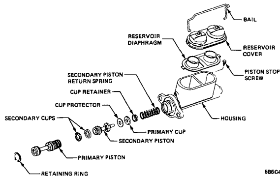
Figure 5C-4 - Exploded View - Master Cylinder H Car
