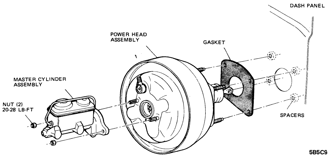
Figure 5C-9 Master Cylinder Mounting - B-C-E Car
