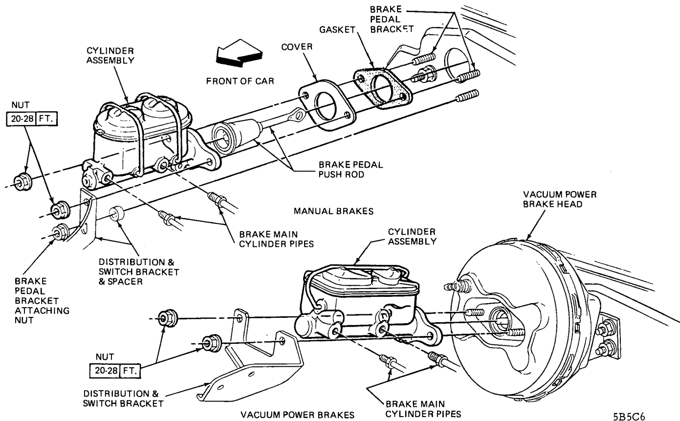
Figure 5C-6 Master Cylinder Mounting-X Car
