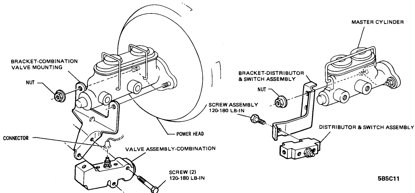
Figure 5C-11 Combination Valve and Distributor Switch to Master Cylinder Mounting - X Car
