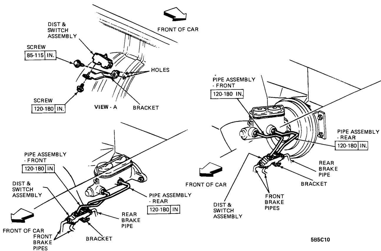
Figure 5C-10 - Distributor Switch to Master Cylinder Mounting - H Car
