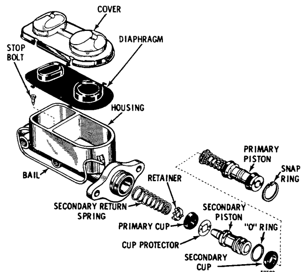
Figure 5C-2 Exploded View - Manual Brake Master Cylinder A - Car
