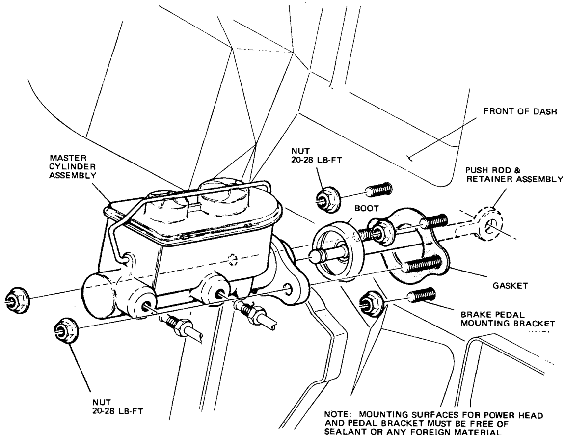
Figure 5C-6 Master Cylinder Mounting-X Car
