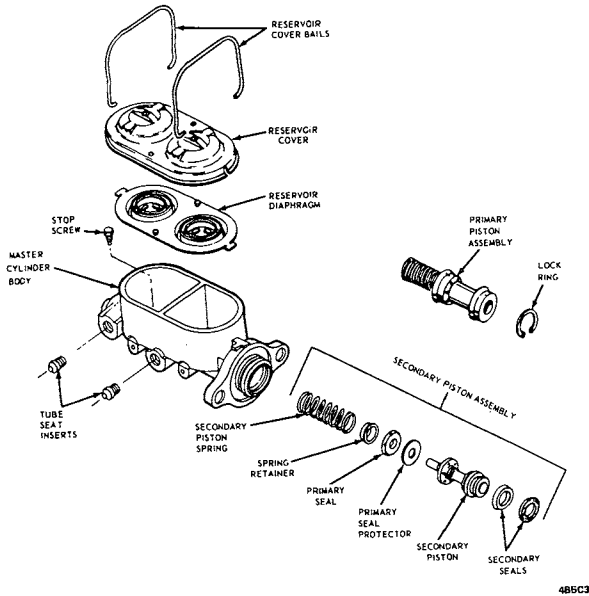
Figure 5C-3 Exploded View - Power Brake Master Cylinder X-Car
