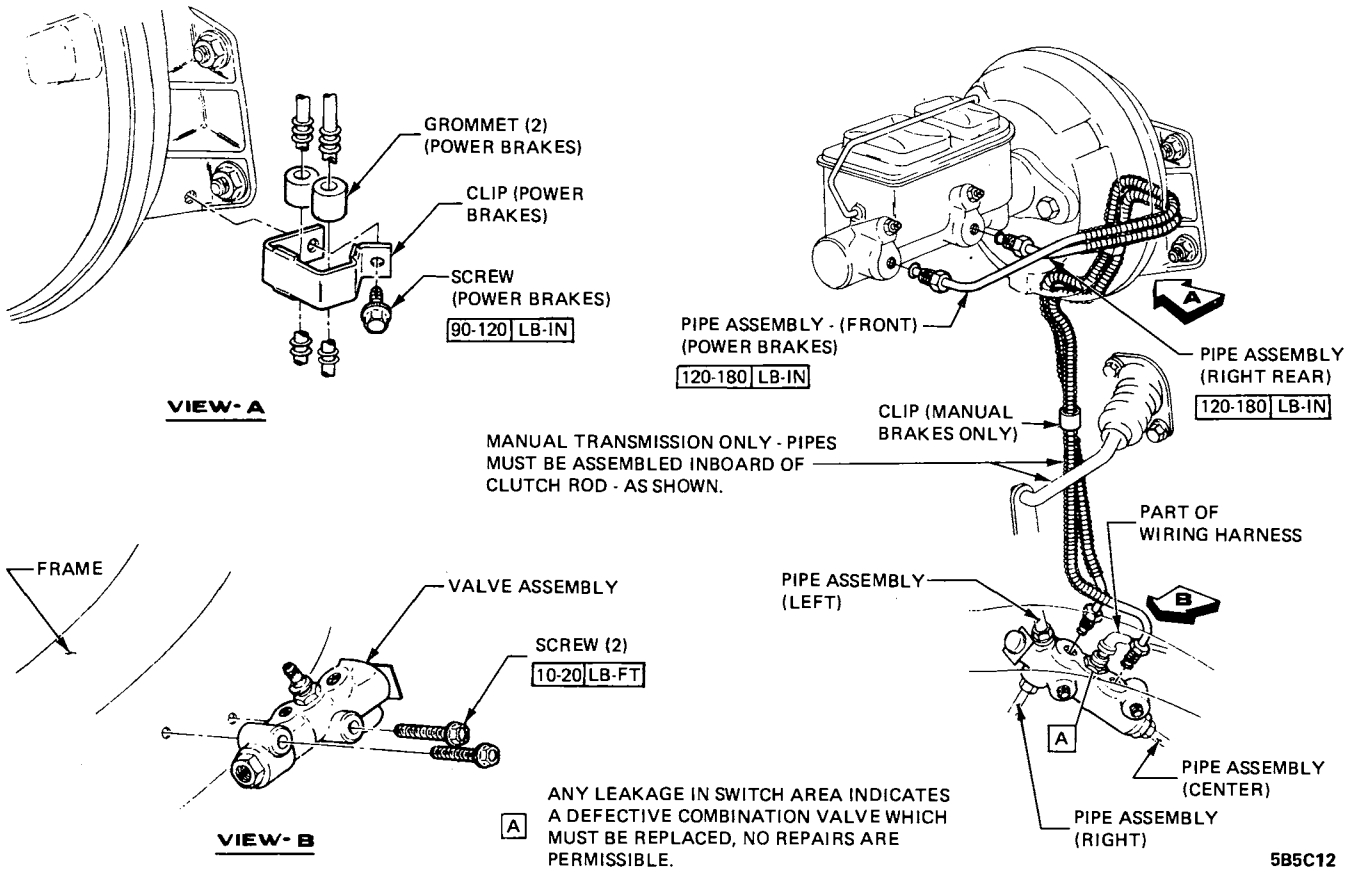
Figure 5C-12 Brake Lines - Master Cylinder to Combination Valve - A Car
