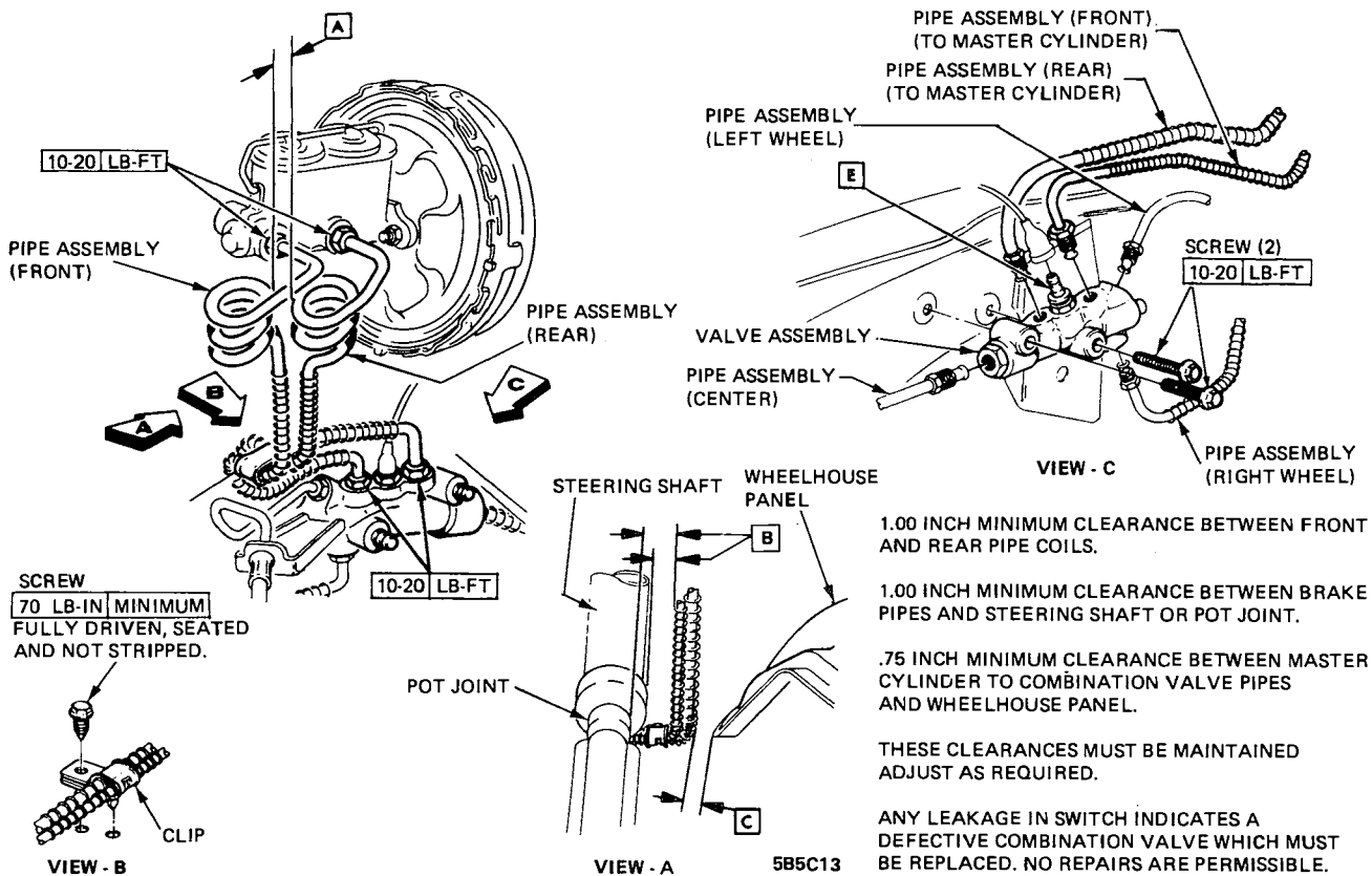
Figure 5C-13 Brake Lines - Master Cylinder to Combination Valve - B-C-E Car
