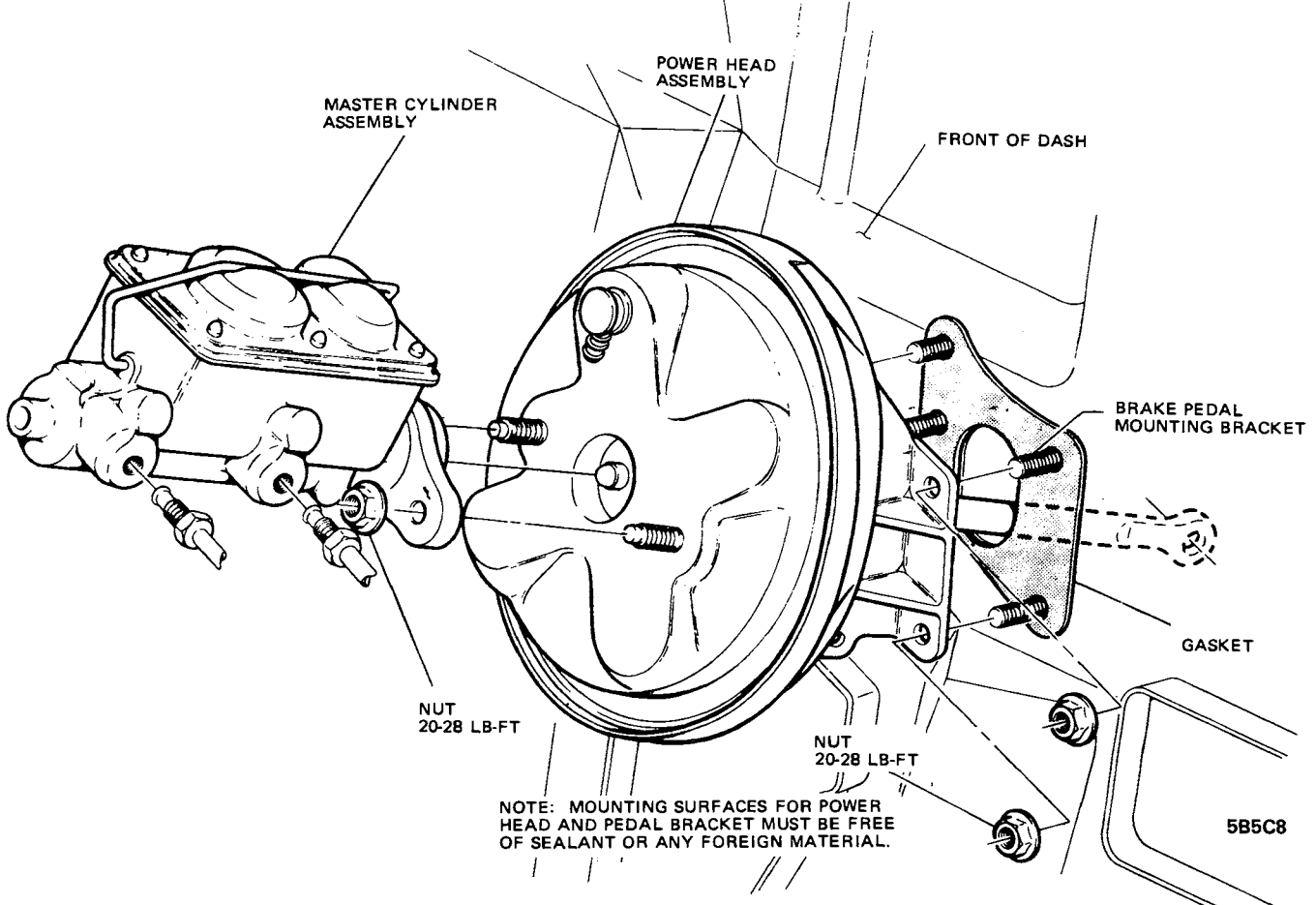
Figure 5C-8 Master Cylinder Mounting - A Car Power Brakes
