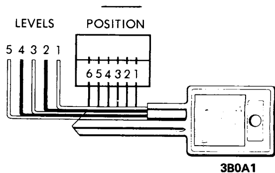
Figure 0A-1 - Key Code Diagram
