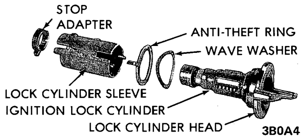
Figure OA-4 Ignition Lock Assembly - Exploded View
