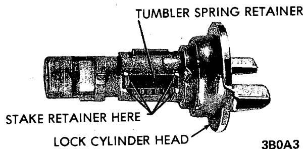
Figure 0A-3 - Installing Spring Retainer
