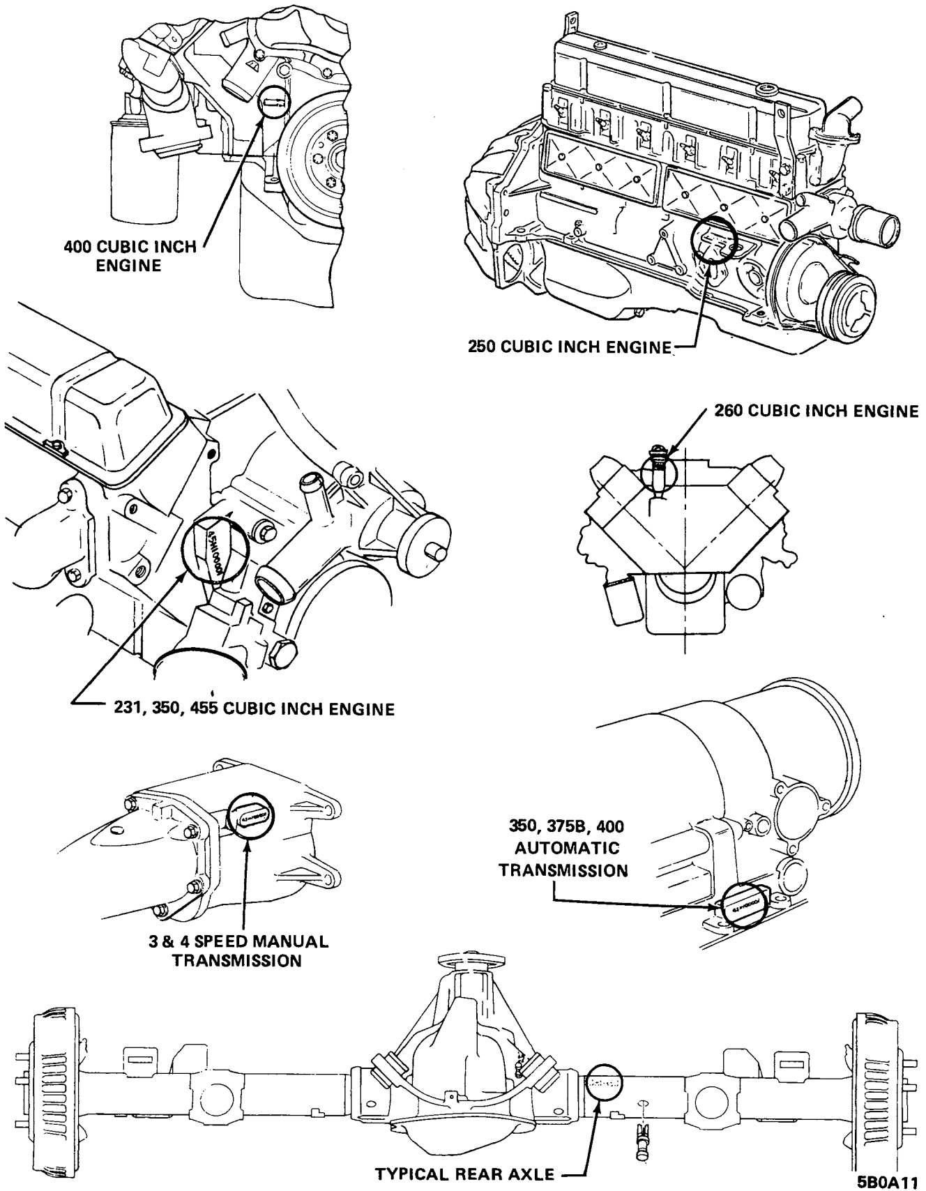
Figure 0A-10 Major Component Serial Number Locations
