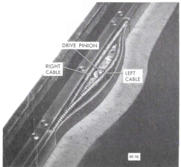
Figure 8E-16 Drive Cables Installed
