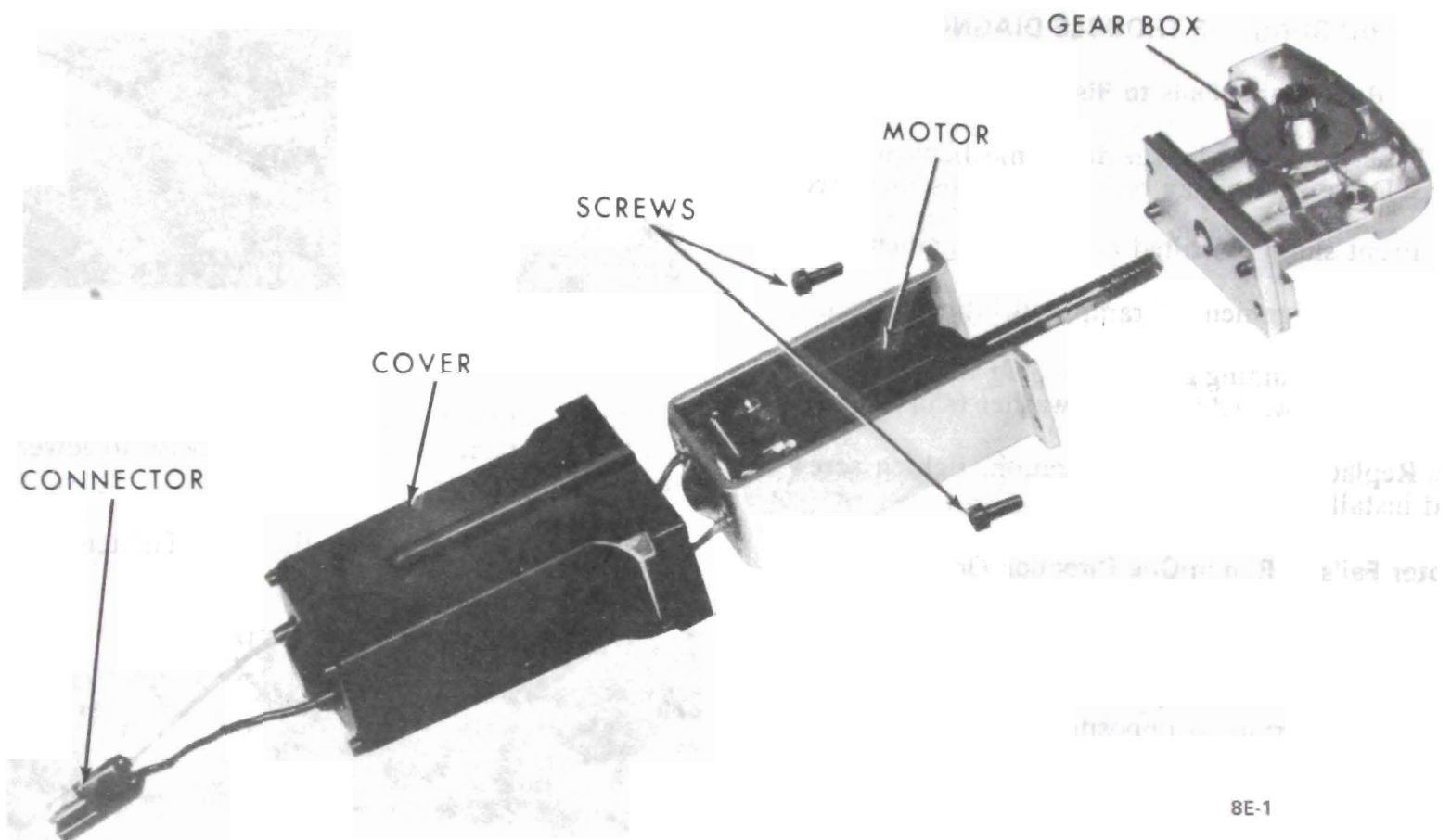
Figure 8E-1 Motor and Drive Unit
