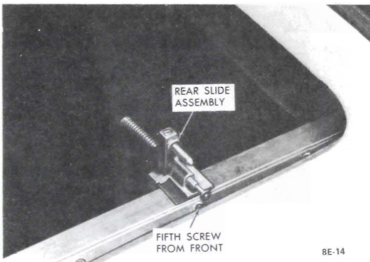
Figure 8E-14 Rear Slide in Centered Position
