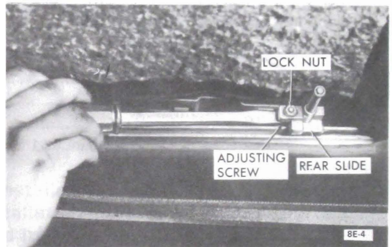
Figure 8E-4 Panel Alignment - Rear
