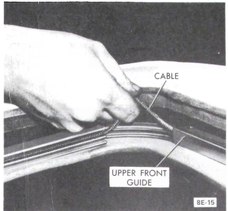
Figure 8E-15 Installing Cable Into Upper Front Guide
