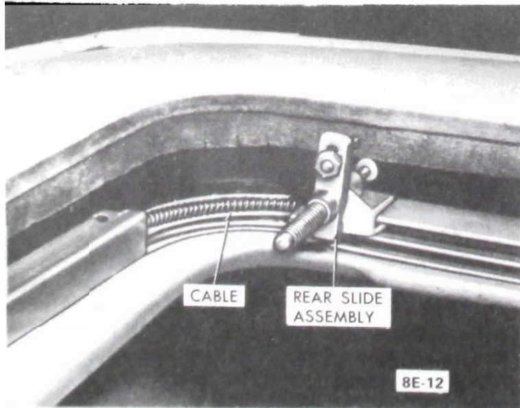
Figure 8E-12 Pull Cable and Slide Assembly Forward
