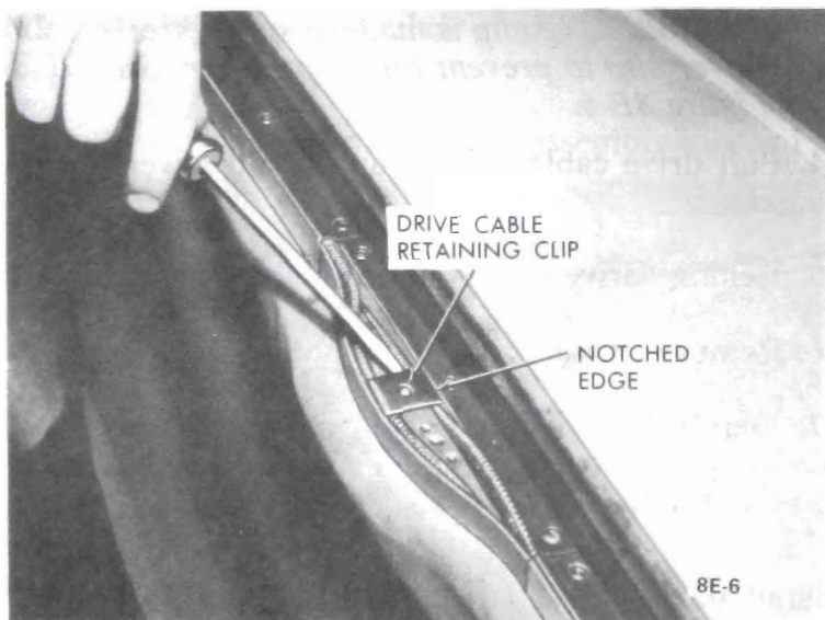
Figure 8E-6 Remove Drive Cable Retaining Clip
