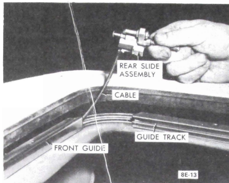
Figure 8E-13 Slide Removed
