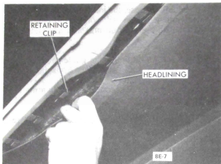
Figure 8E-7 Headlining Panel Removal
