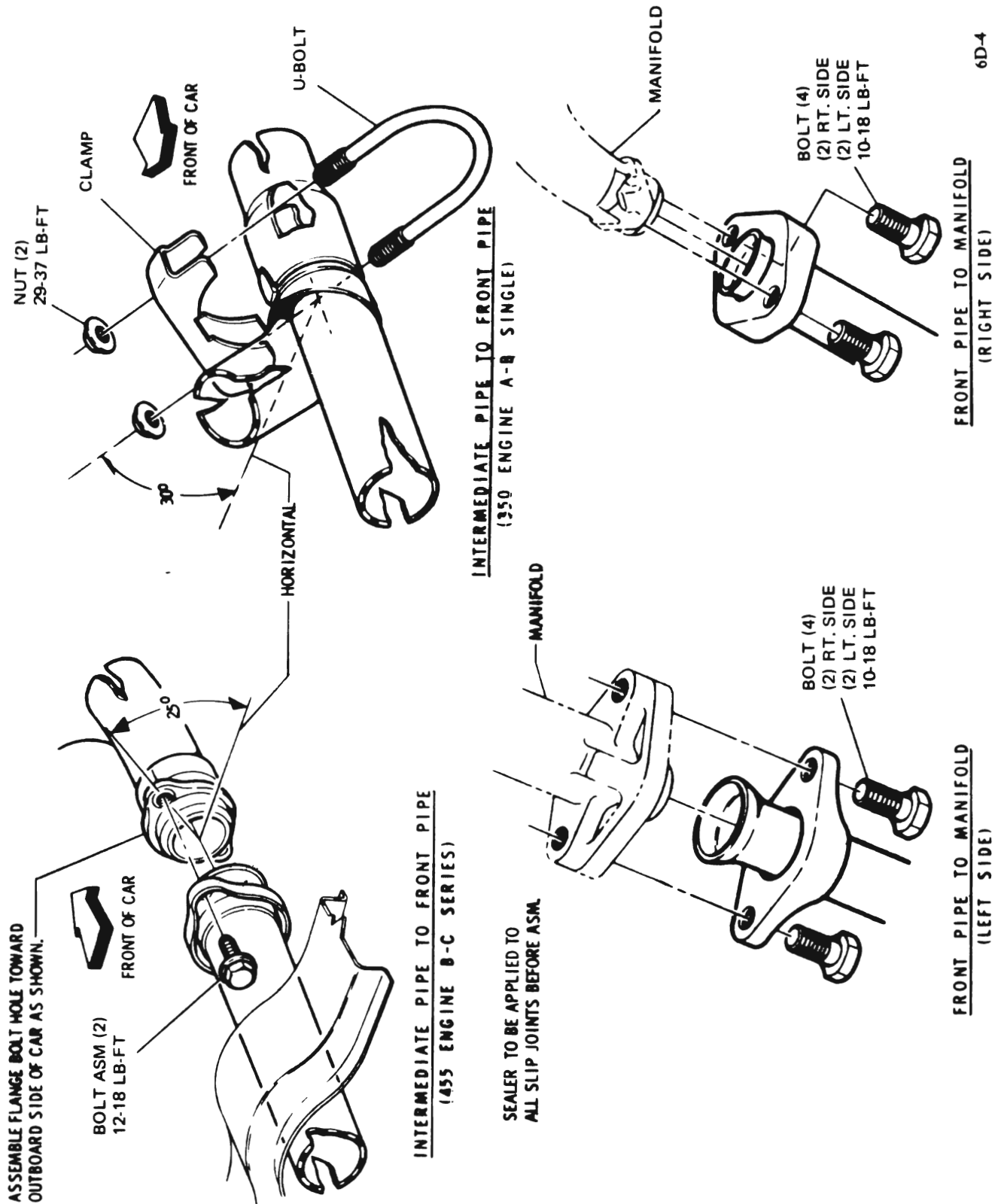
Figure 6D-4 "A" Series Exhaust Pipes to Manifold Attachments
