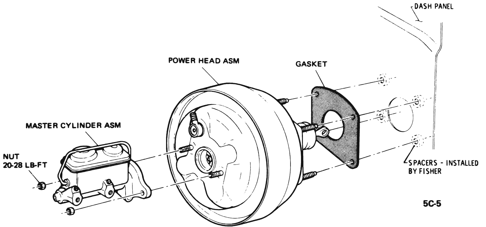
Figure 5C-5 Master Cylinder Mounting - B-C-E Car Power Brakes
