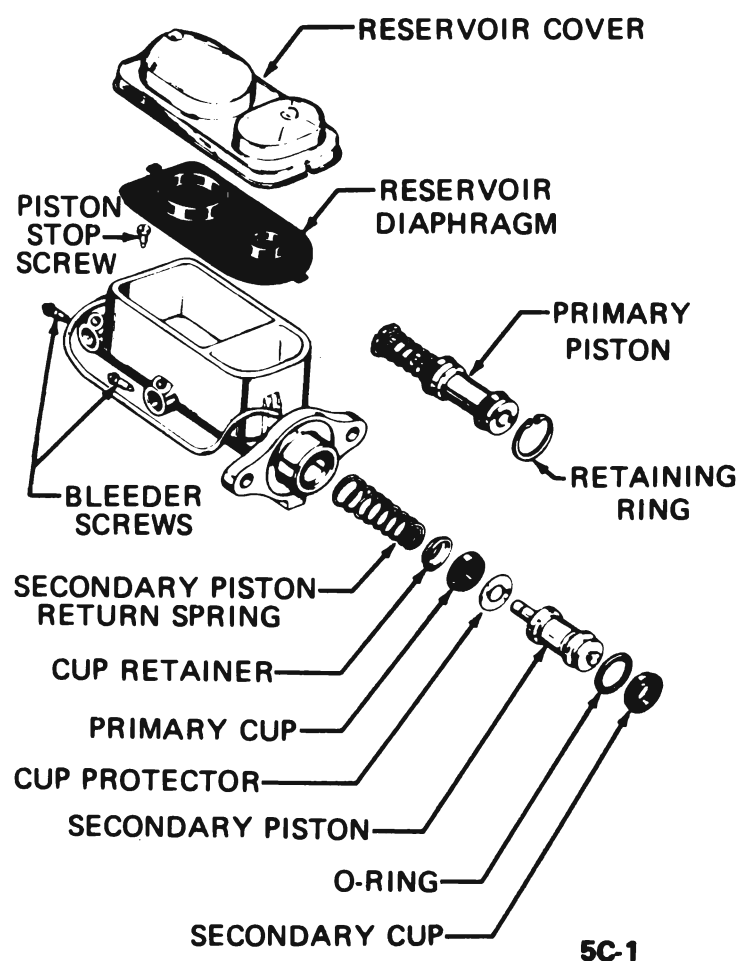
Figure 5C-1 Exploded View - Power Brake Master Cylinder
