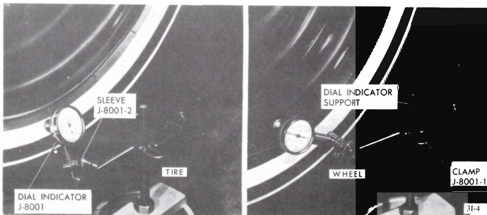
Figure 31-4 Checking Lateral Runout
