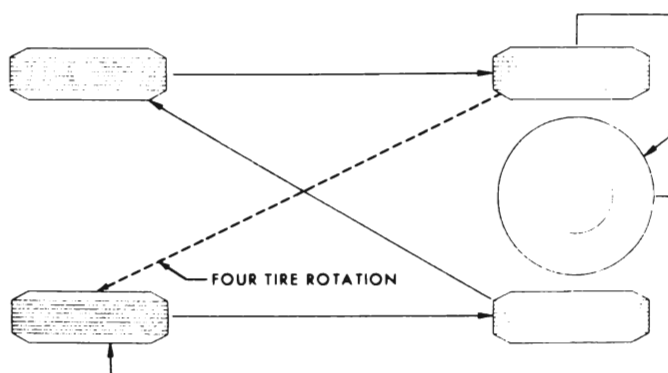
Figure 31-6 Standard Tire Rotation
