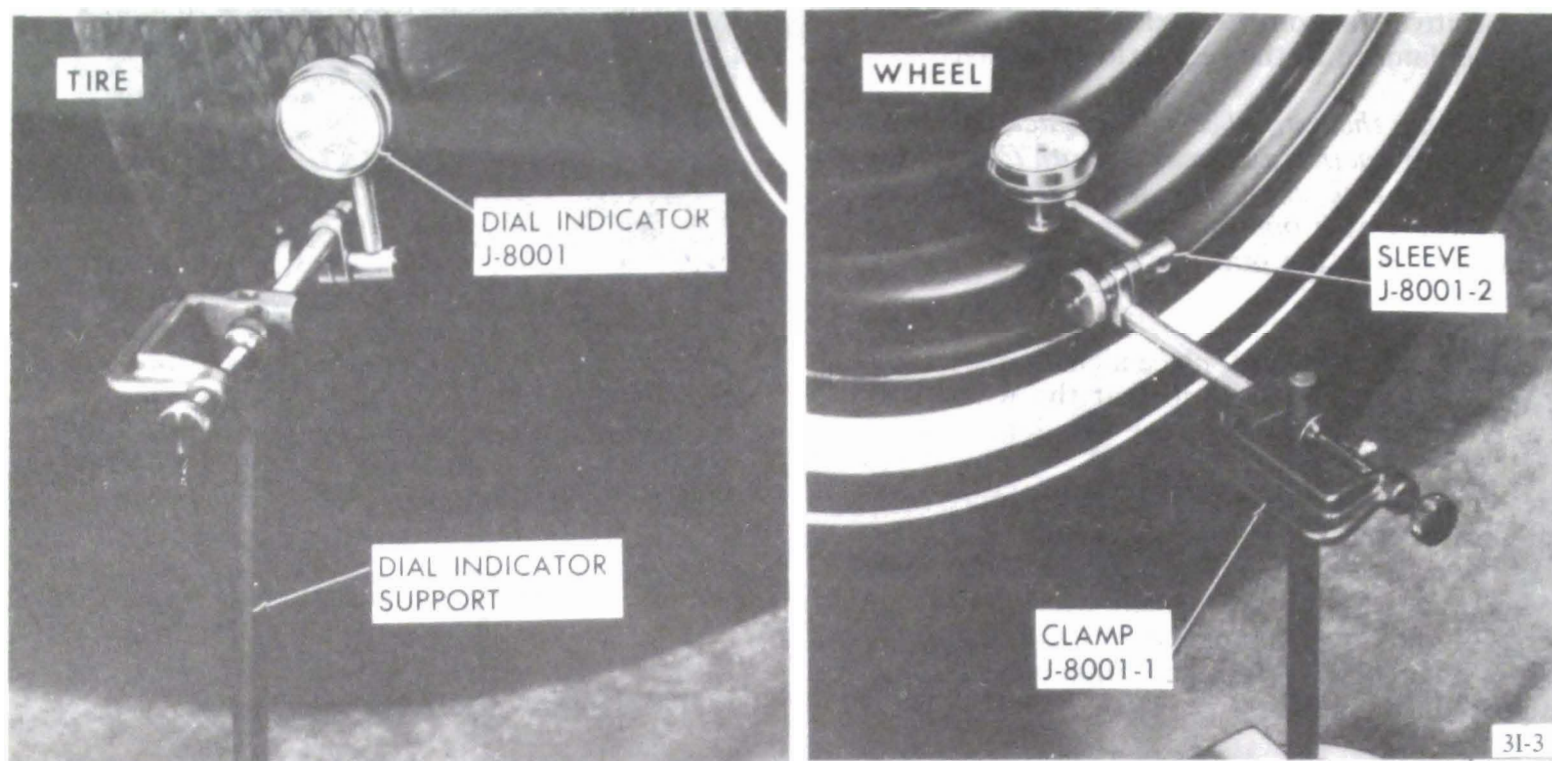
Figure 31-3 Checking Radial Runout
