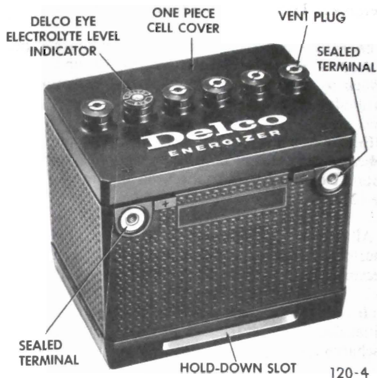
Figure 120-4 Side Terminal Battery - All Series
