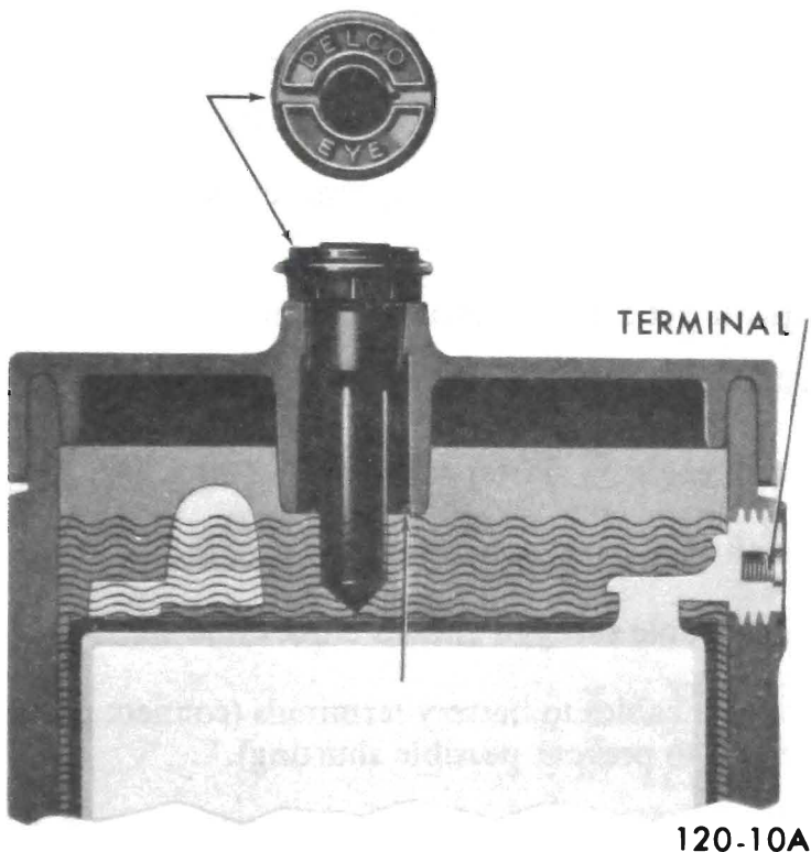
Figure 120-9 Electrolyte Level Correct
