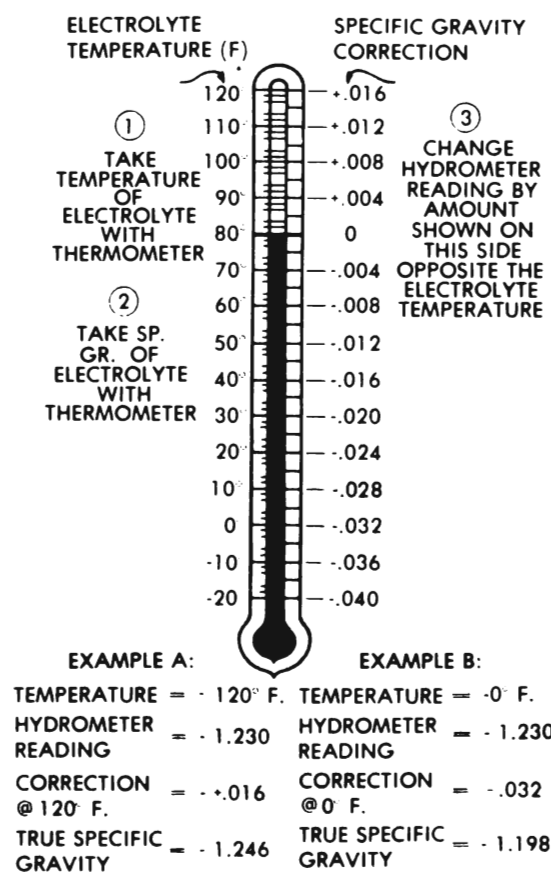
Figure 120-3 Specific Gravity Temperature Correction Scales
