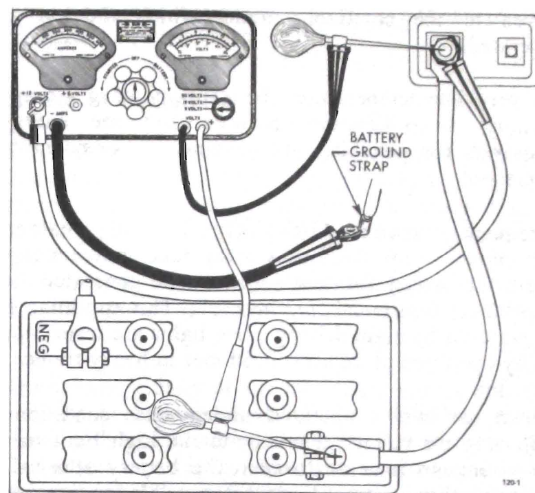
Figure 120-1 Battery, Cable Test Connections
