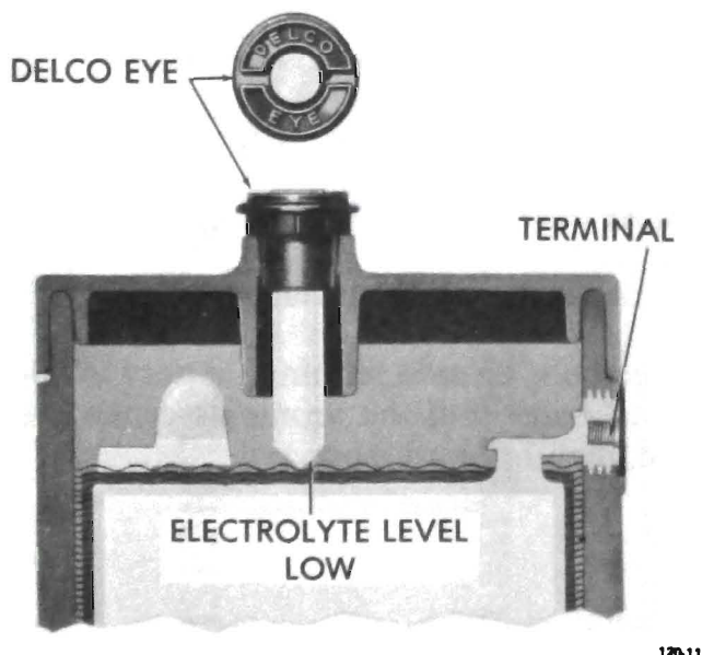
Figure 120-10 Low Electrolyte Level
