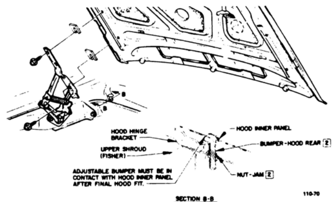
Figure 110-1 Shimming Hood to Hood Hinge
