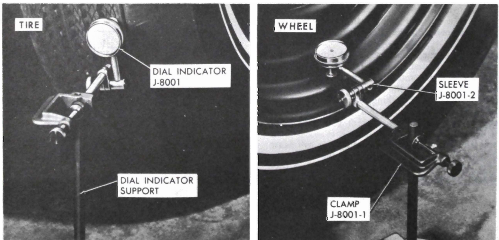
Figure 100-3 Checking Radial Runout
