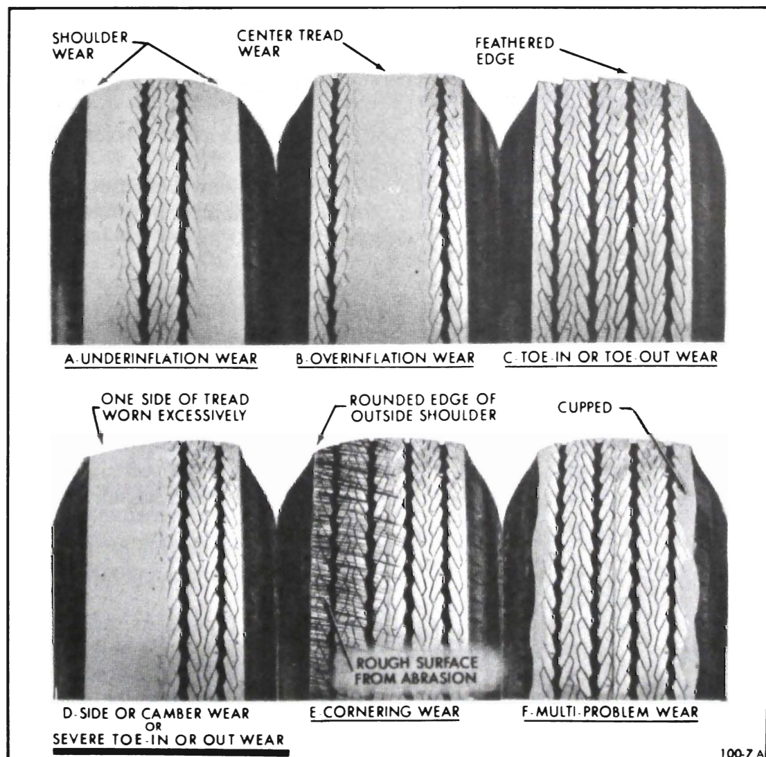
Figure 100-9 Abnormal Tire Wear Patterns
