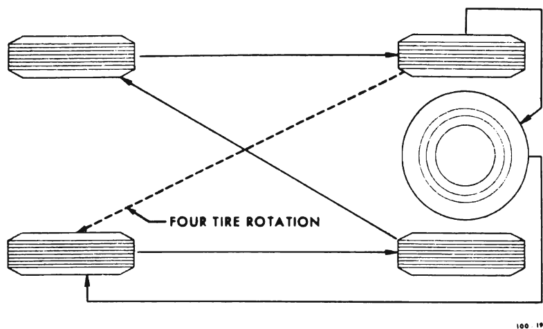
Figure 100-6 Tire Rotation
