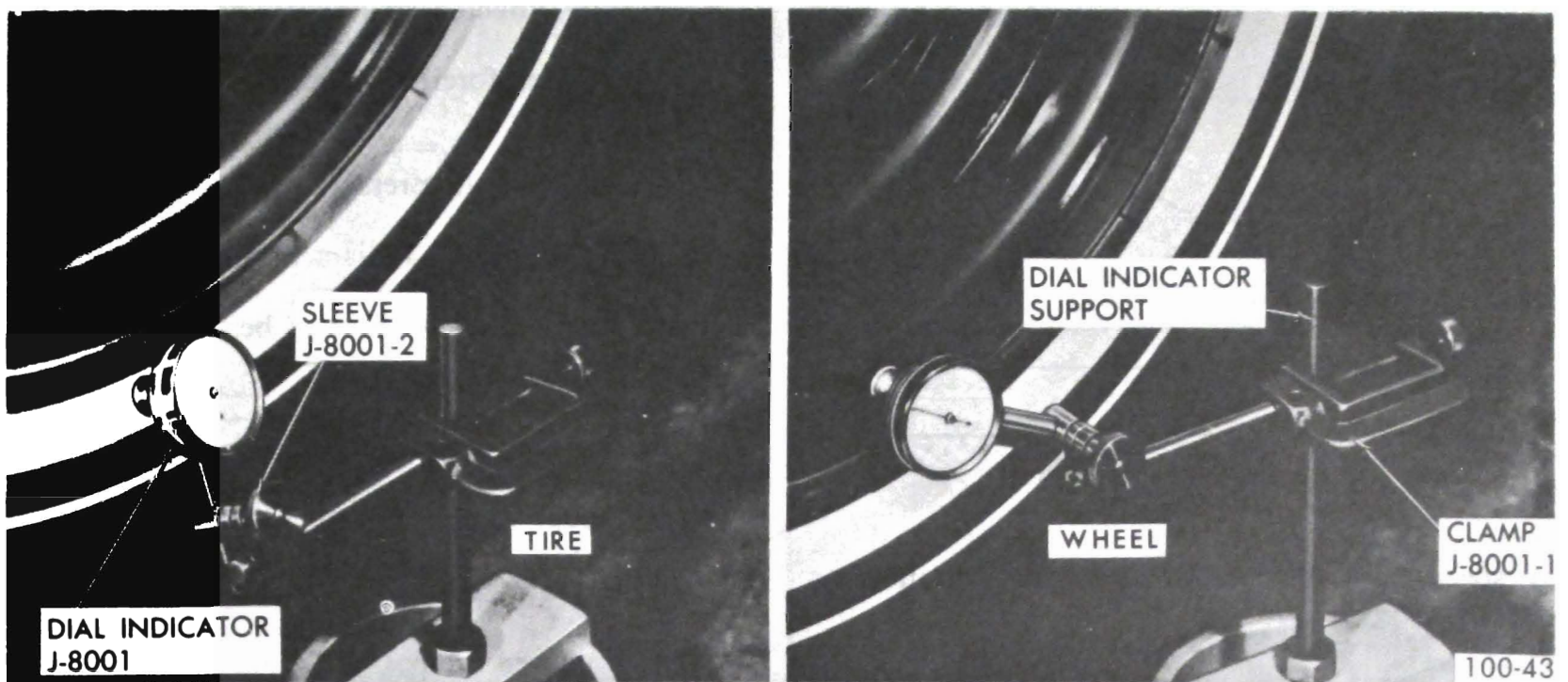
Figure 100-4 Checking Lateral Runout
