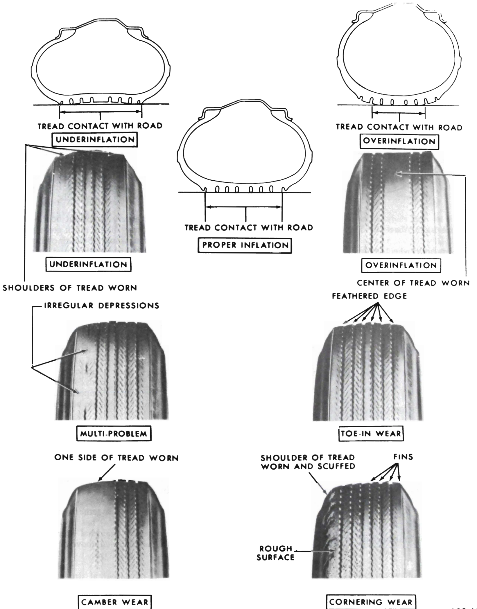
Figure 100-7 Uneven Tire Wear
