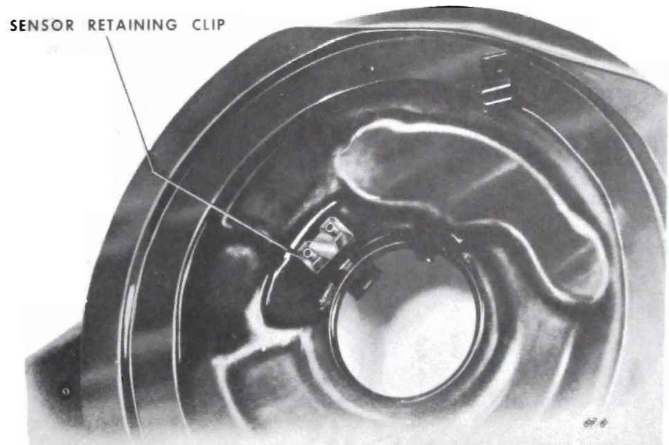
Figure 67-6 - Replacing Sensor Assembly
