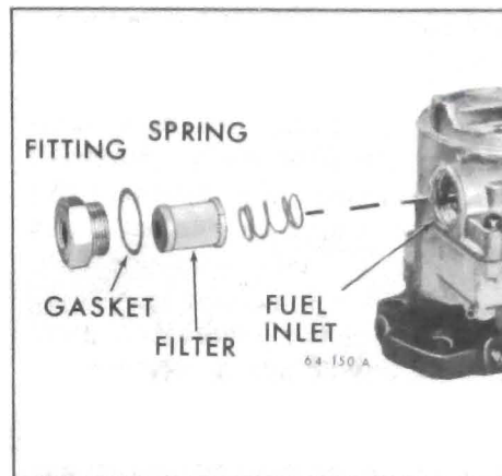
Figure 64-6 - Fuel Filter Parts
