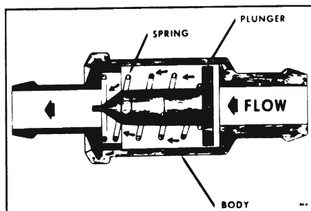
Figure 64-7 - Positive Crankcase Ventilator Valve
