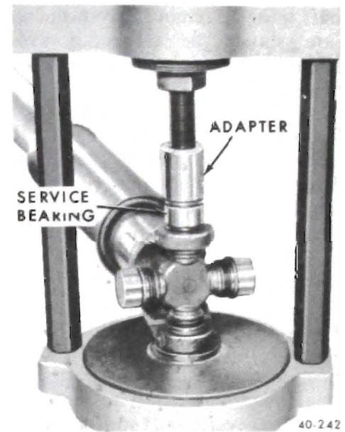
Figure 40-52 - Installing U-Joint Bearing
