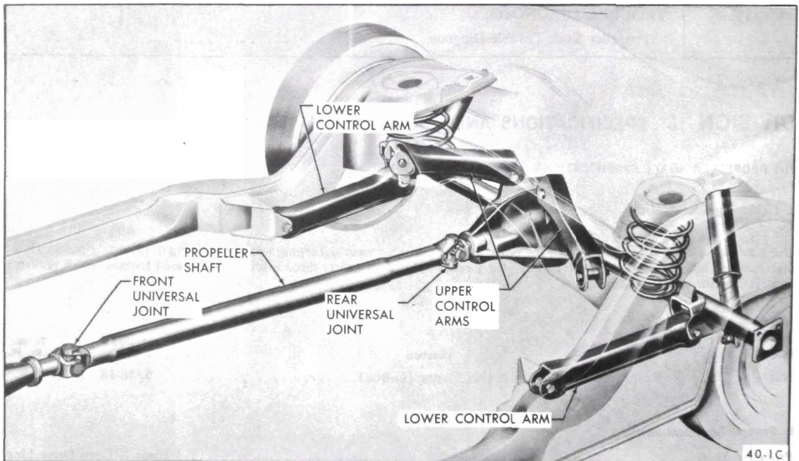
Figure 40-45 - Propeller Shaft Assembly
