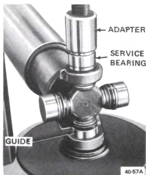
Figure 40-51 - Installing U-Joint Bearing With Guide in Place.
