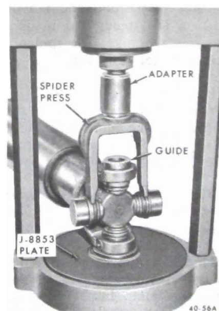
Figure 40-49 - Pressing Out U-Joint Bearing With Guide Installed
