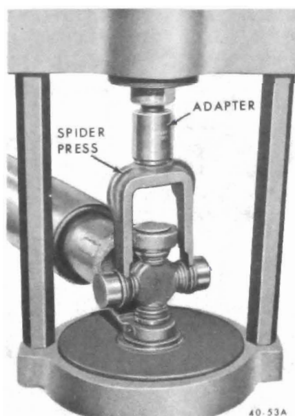
Figure 40-48 - Pressing Out U-Joint Bearing
