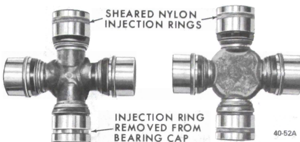
Figure 40-47 - Production Universal Joints
