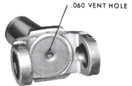
Figure 40-46 - Slip Yoke With Vent Hole
