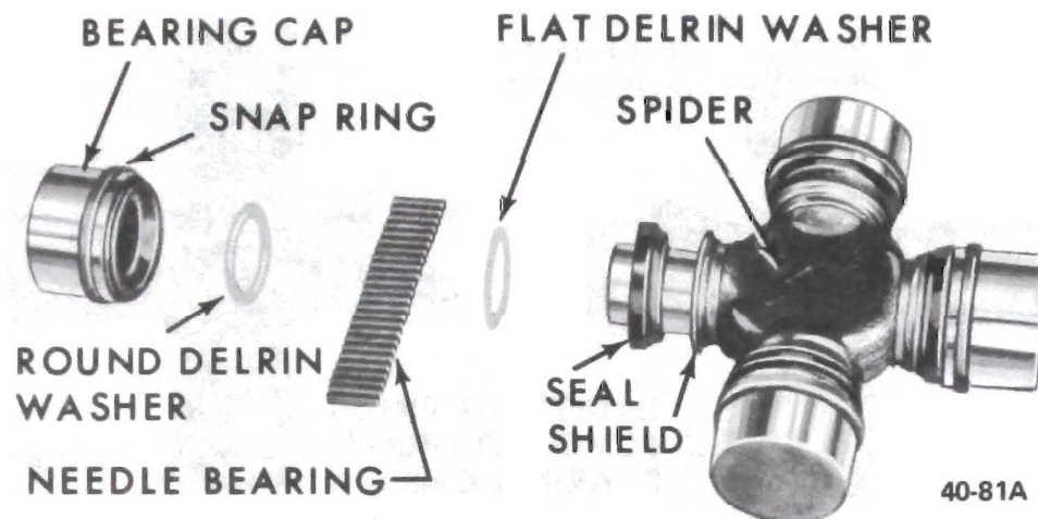
Figure 40-50 - Service Universal Joint
