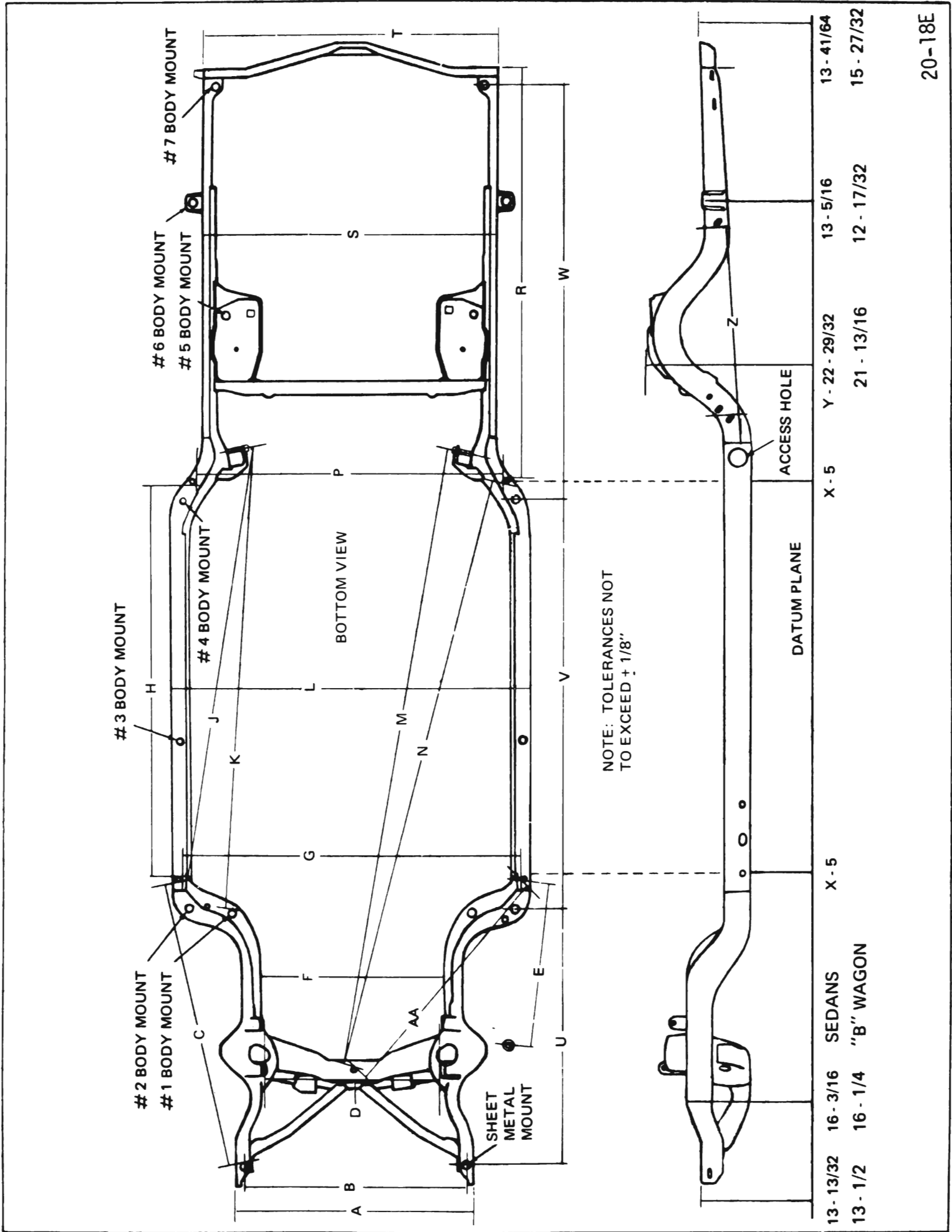
Figure 20-7 - 45-46-48000 Frame Details
