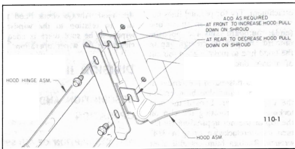
Figure 110-9 Shimming Hood to Hood Hinge
