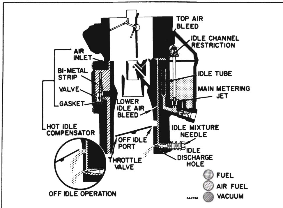
Figure 64-55 - Idle (Low Speed) System
