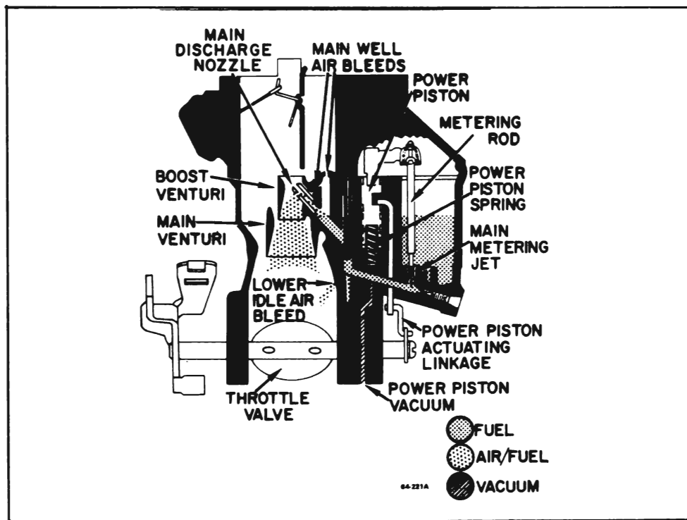
Figure 64-57 - Power System
