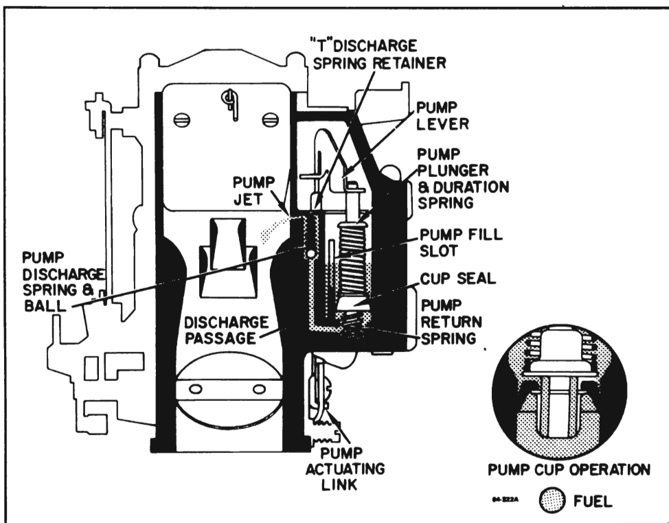
Figure 64-58 - Accelerating Pump System
