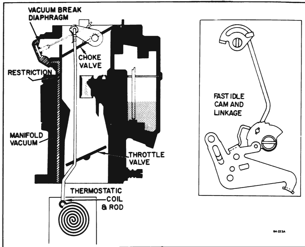
Figure 64-59 - Choke System
