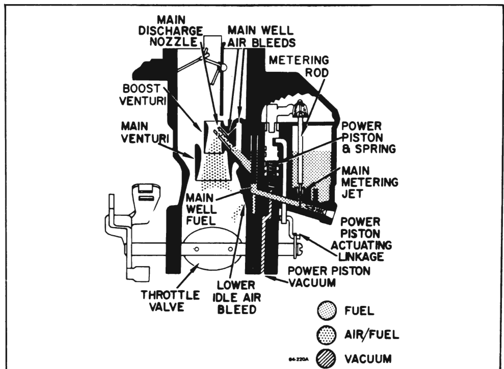
Figure 64-56 - Main Metering (High Speed) System
