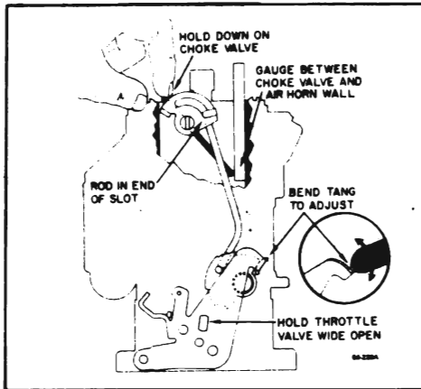
Figure 64-65 Choke Unloader Adjustment
