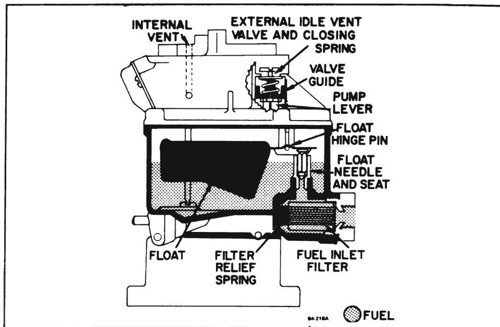
Figure 64-54 - Float System
