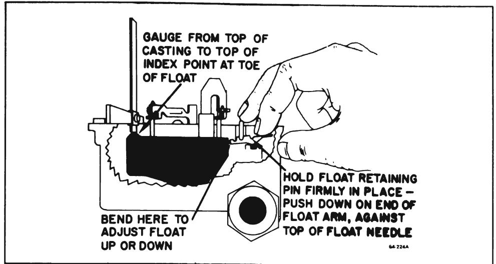
Figure 64-60 - Float Level Adjustment
