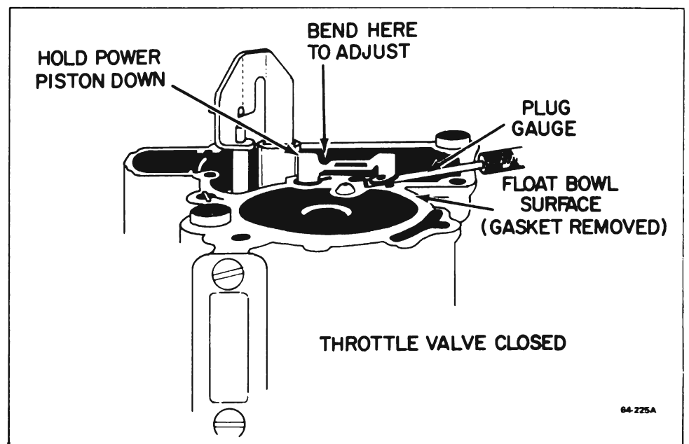
Figure 64-61 - Metering Rod Adjustment
