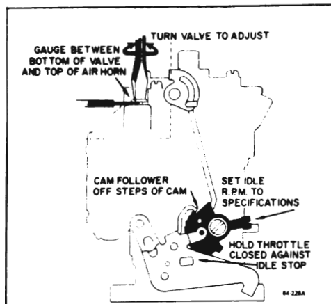
Figure 64-62 Idle Vent Adjustment
