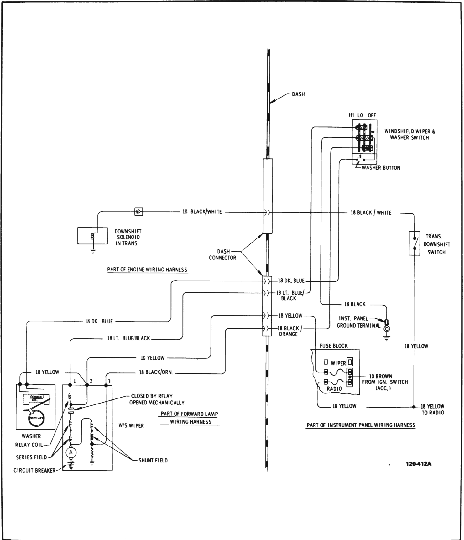
Figure I20-118 Wiper and Transmission Downshift Switch Wiring Diagram - LeSabre, Wildcat, Electra and Riviera
