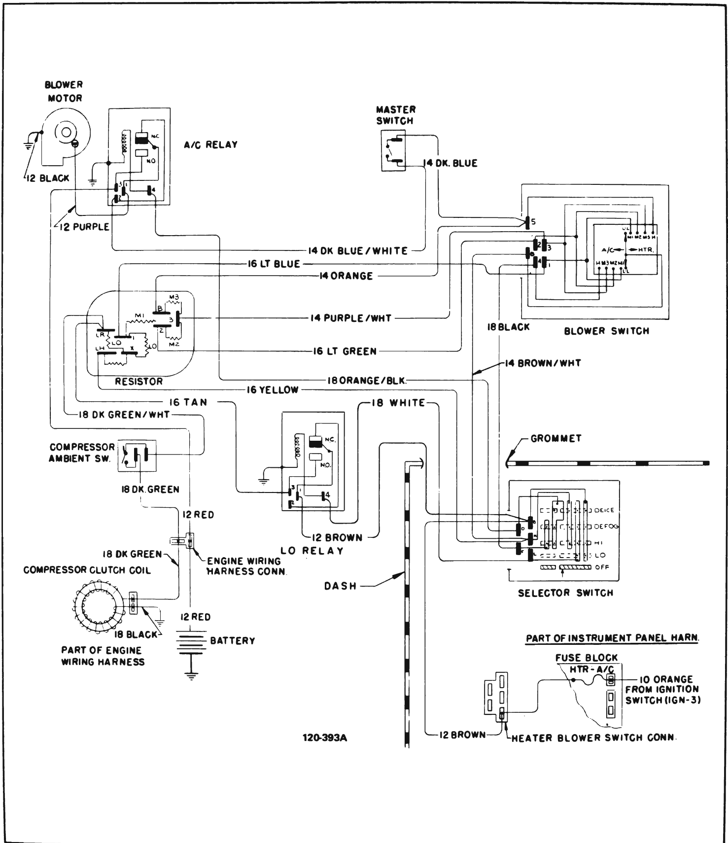
Figure 120-96 Automatic Air Conditioner Wiring Diagram - Riviera
