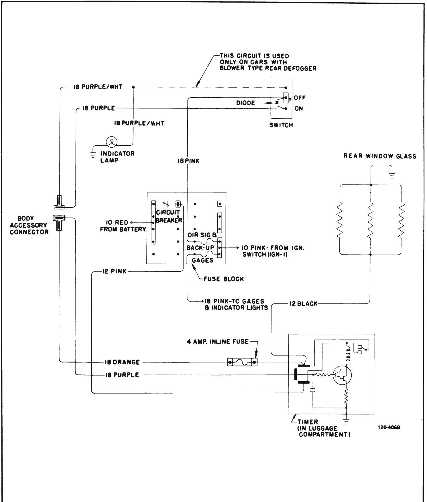
Figure I20-115 Electrically Heated Rear Window Glass - Riviera
