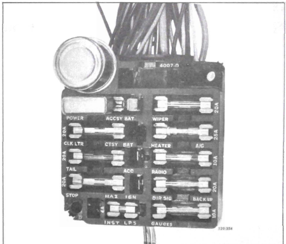
Figure I20-52 Fuse Block - All Series
