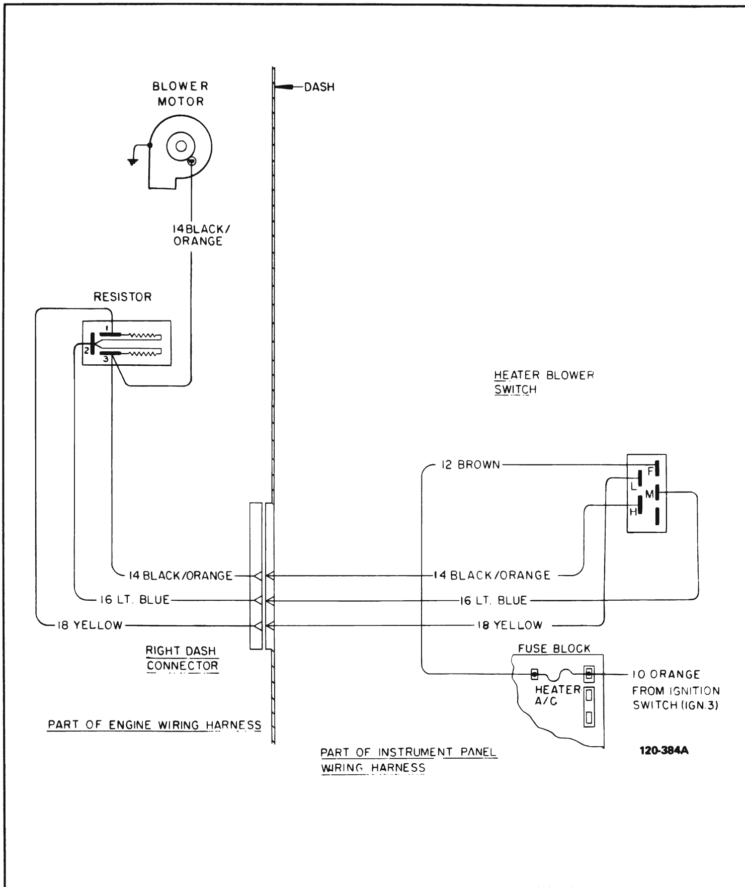
Figure I20-89 Heater Wiring Diagram - Riviera
