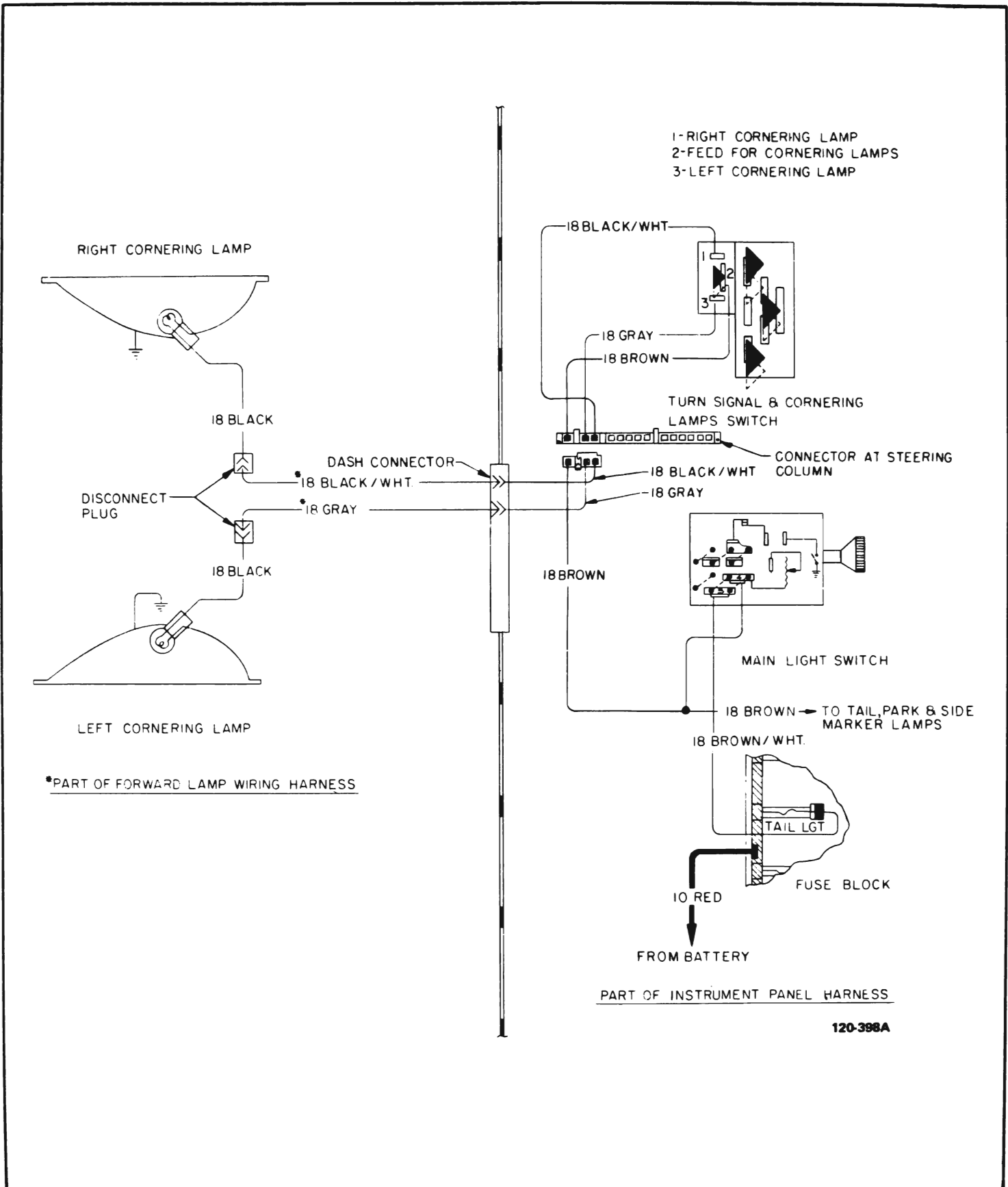
Figure 120-110 Cornering Light Wiring Diagram
