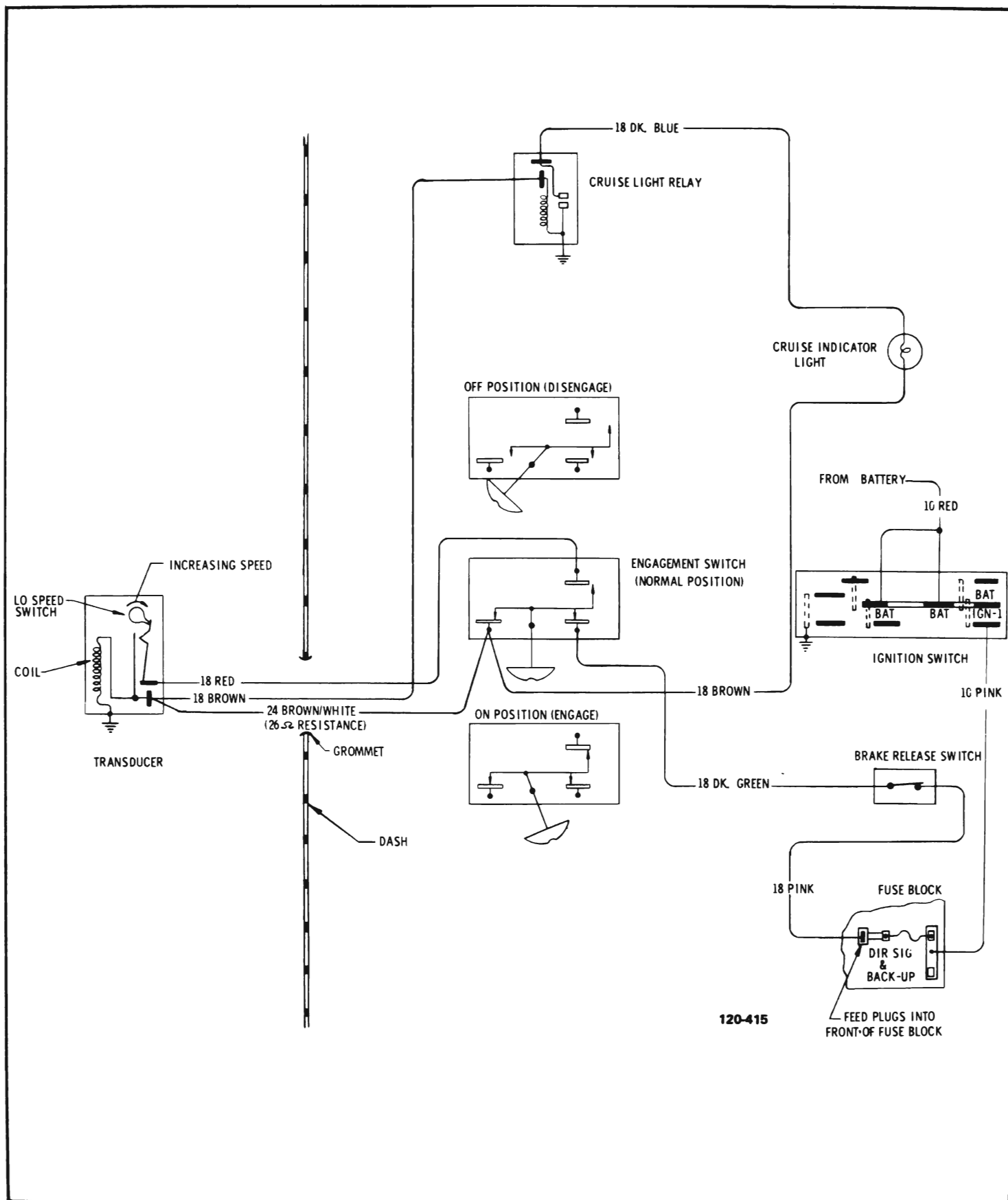
Figure 120-120 Cruise Master Wiring Diagram - 43-44000
