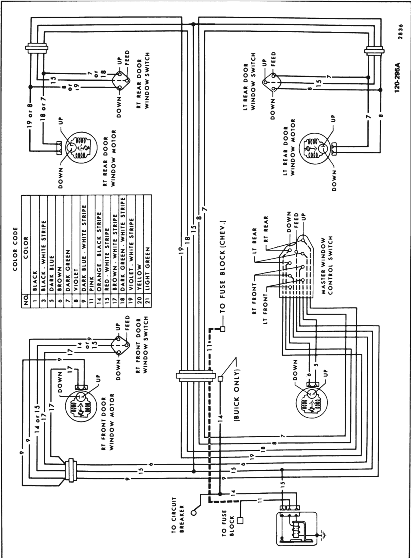
Figure 120-103 Power Window Wiring Diagram - LeSabre, Wildcat and Electra
