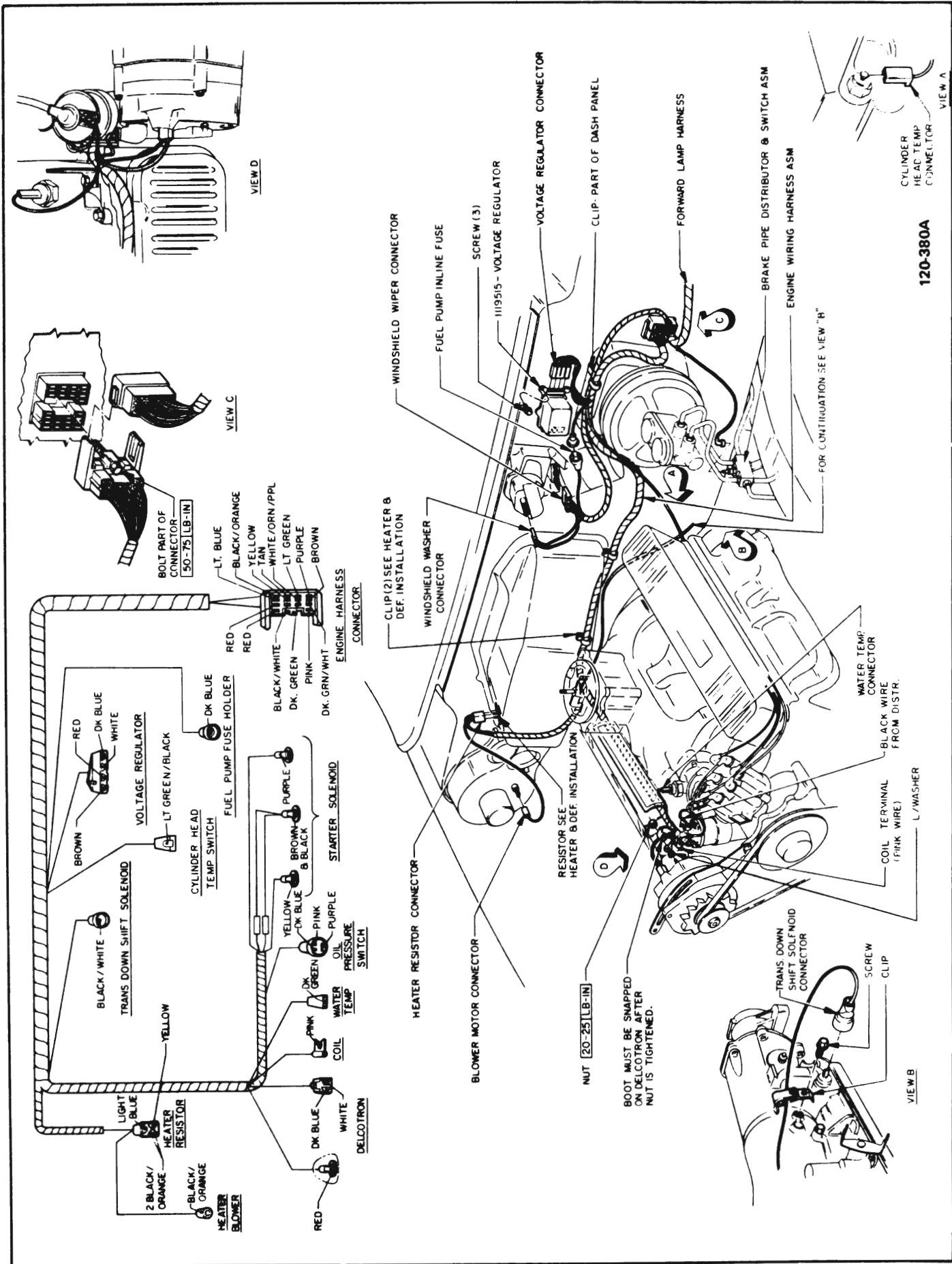
Figure 120-85 Engine Wiring Harness - Riviera
