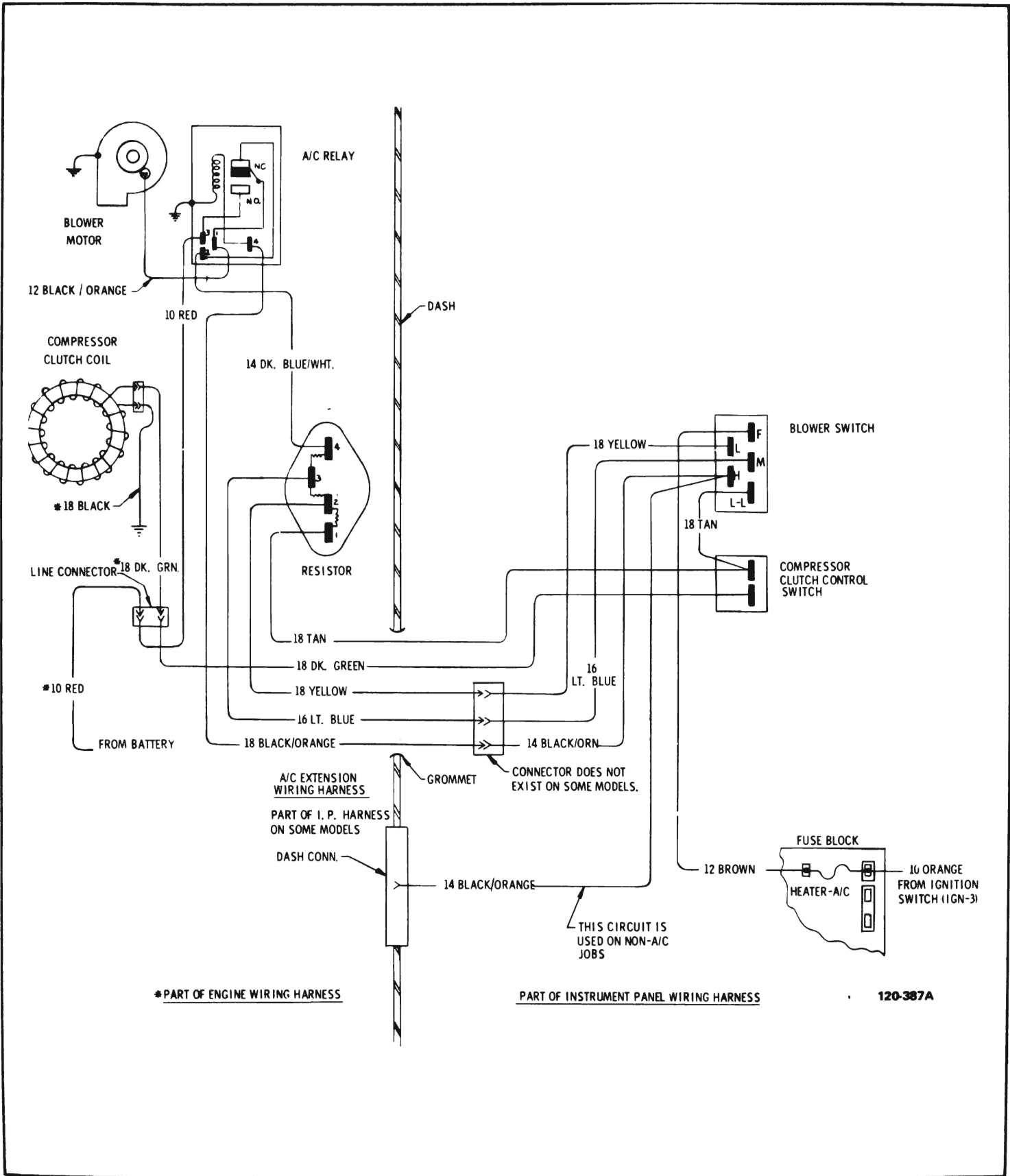
Figure 120-92 Manual Air Conditioner Wiring Diagram - LeSabre, Wildcat and Electra
