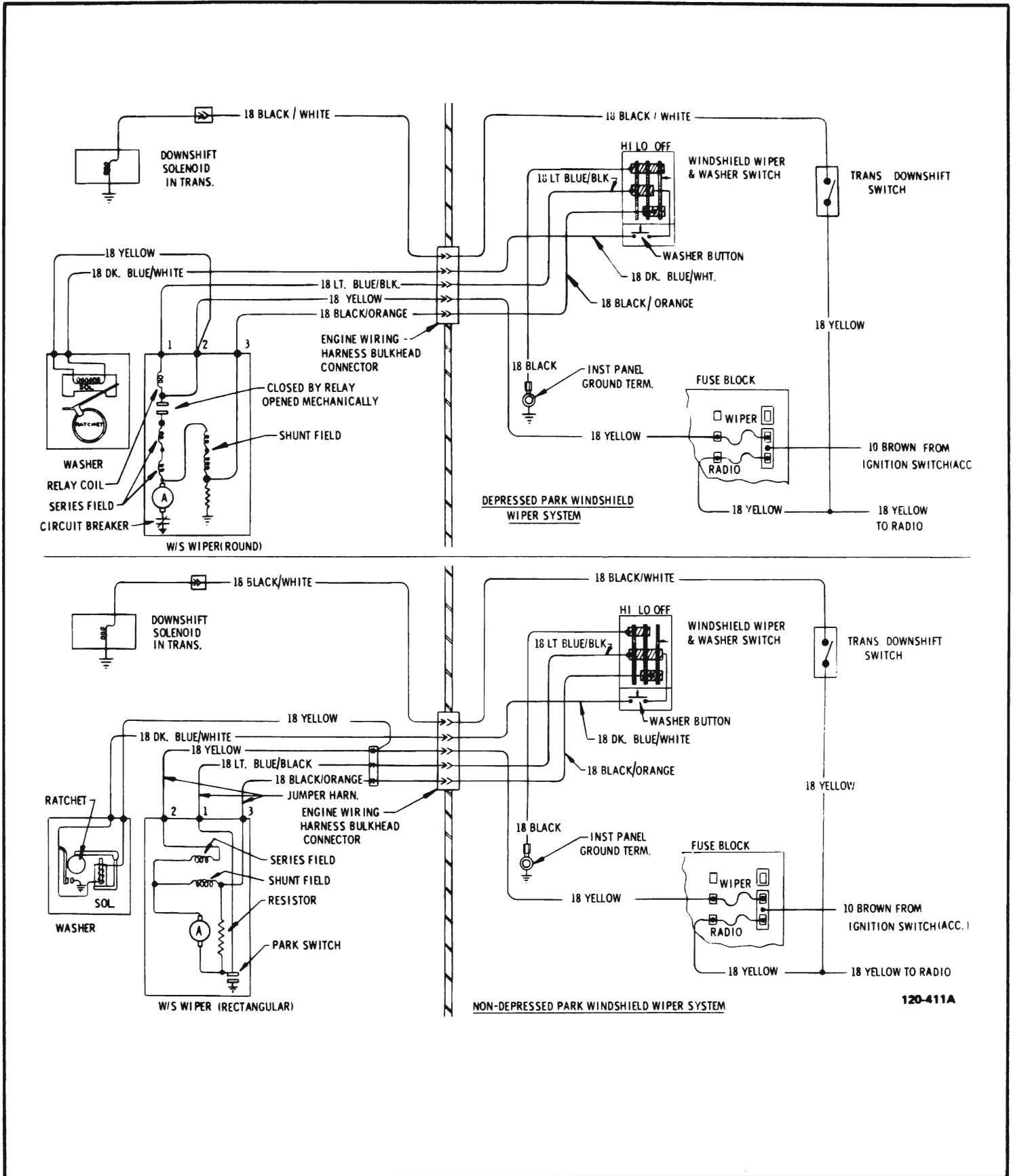
Figure I20-117 Wiper and Transmission Downshift Switch Wiring Diagram - 43-44000
