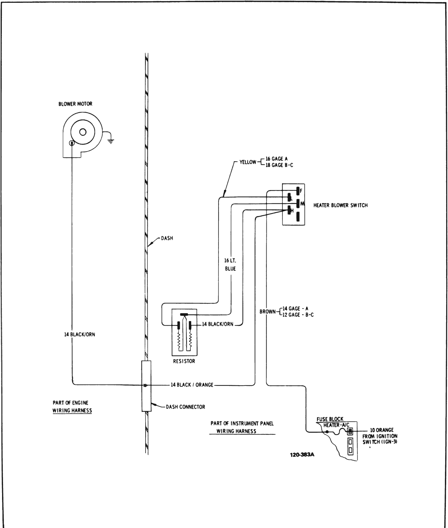
Figure I20-88 Heater Wiring Diagram - Except Riviera
