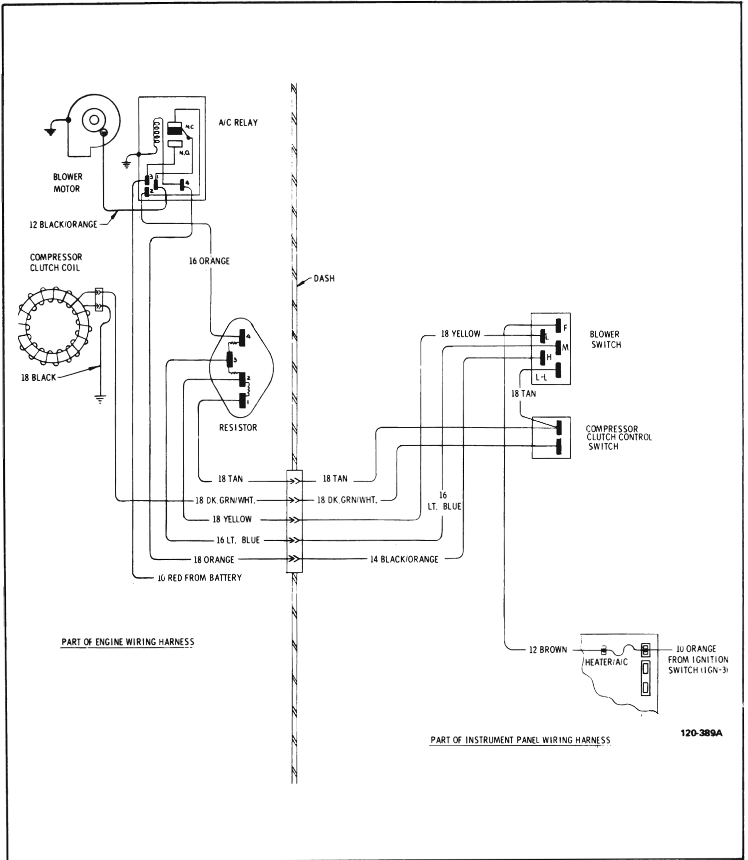
Figure I20-93 Manual Air Conditioner Wiring Diagram - Riviera
