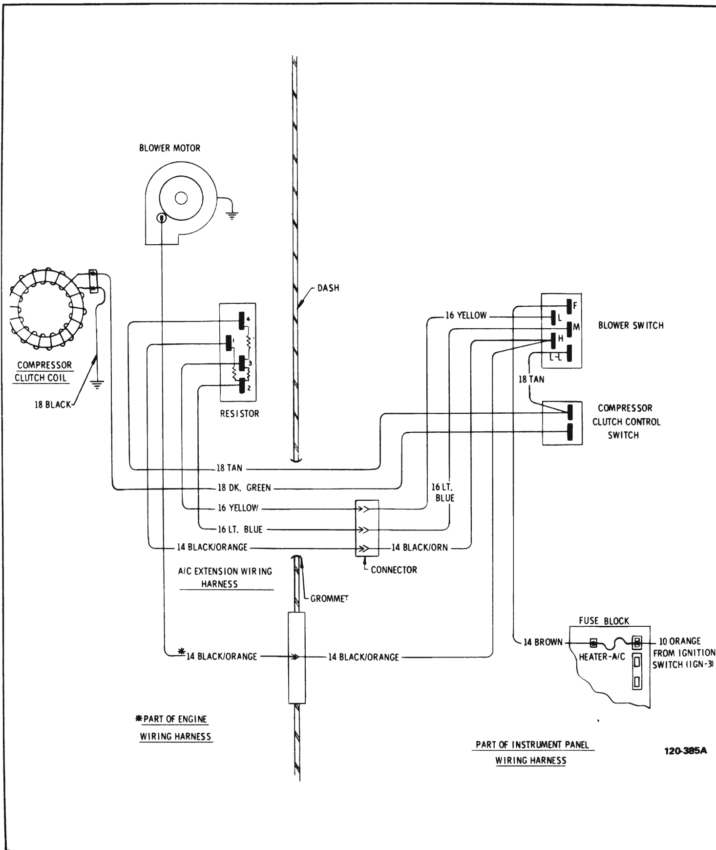
Figure I20-90 Air Conditioner Wiring Diagram - 43-44000
