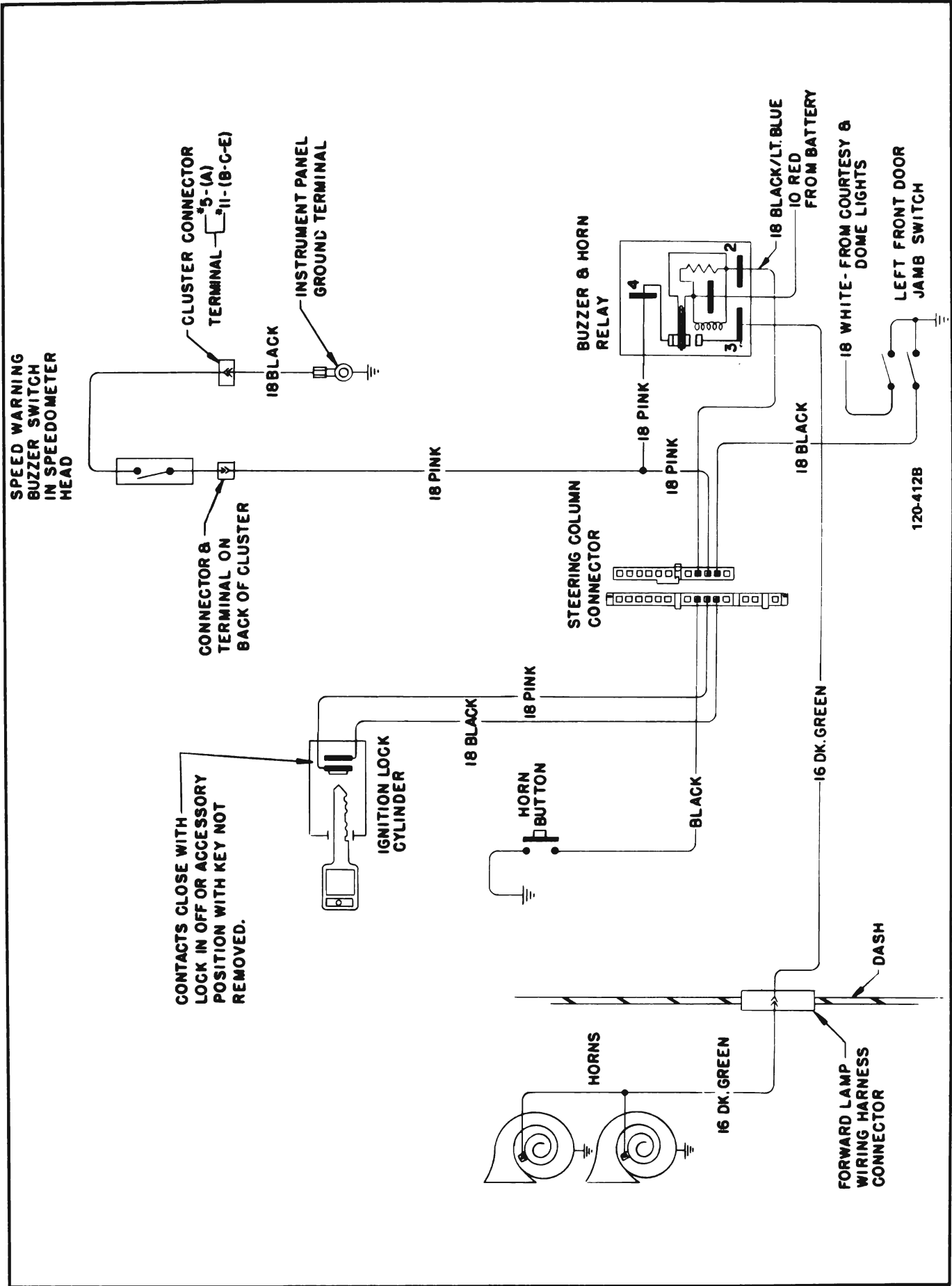
Figure 120-119 Horn Relay, Speedometer and Ignition Key Buzzer Wiring Diagram
