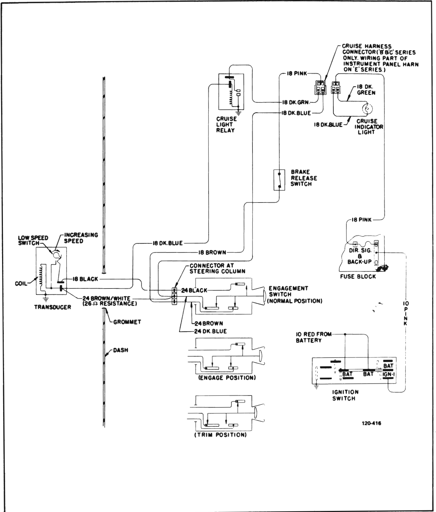
Figure 120-121 Cruise Master Wiring Diagram - 45-46-48-49000
