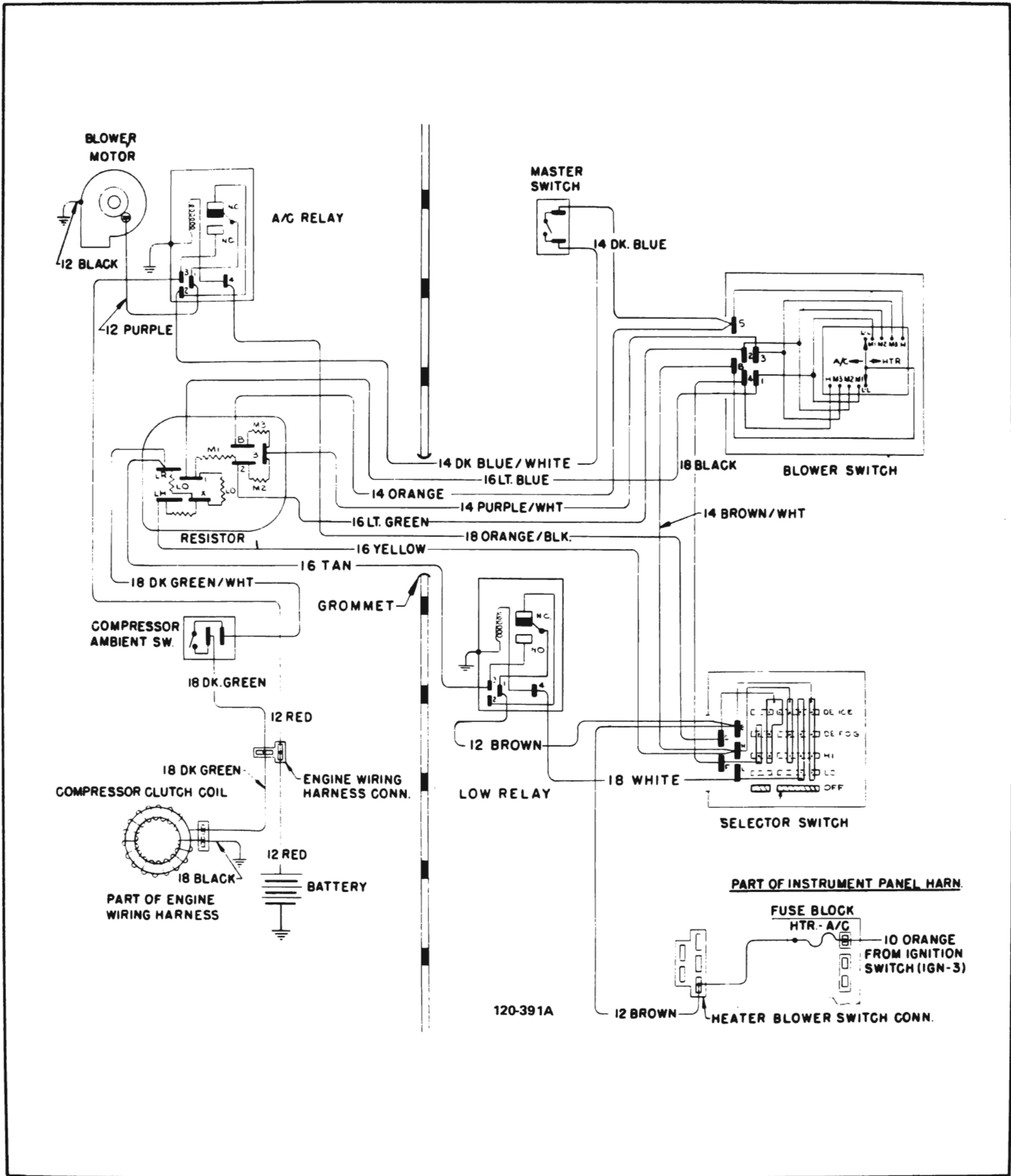
Figure I20-94 Automatic Air Conditioner Wiring Diagram - LeSabre, Wildcat and Electra
