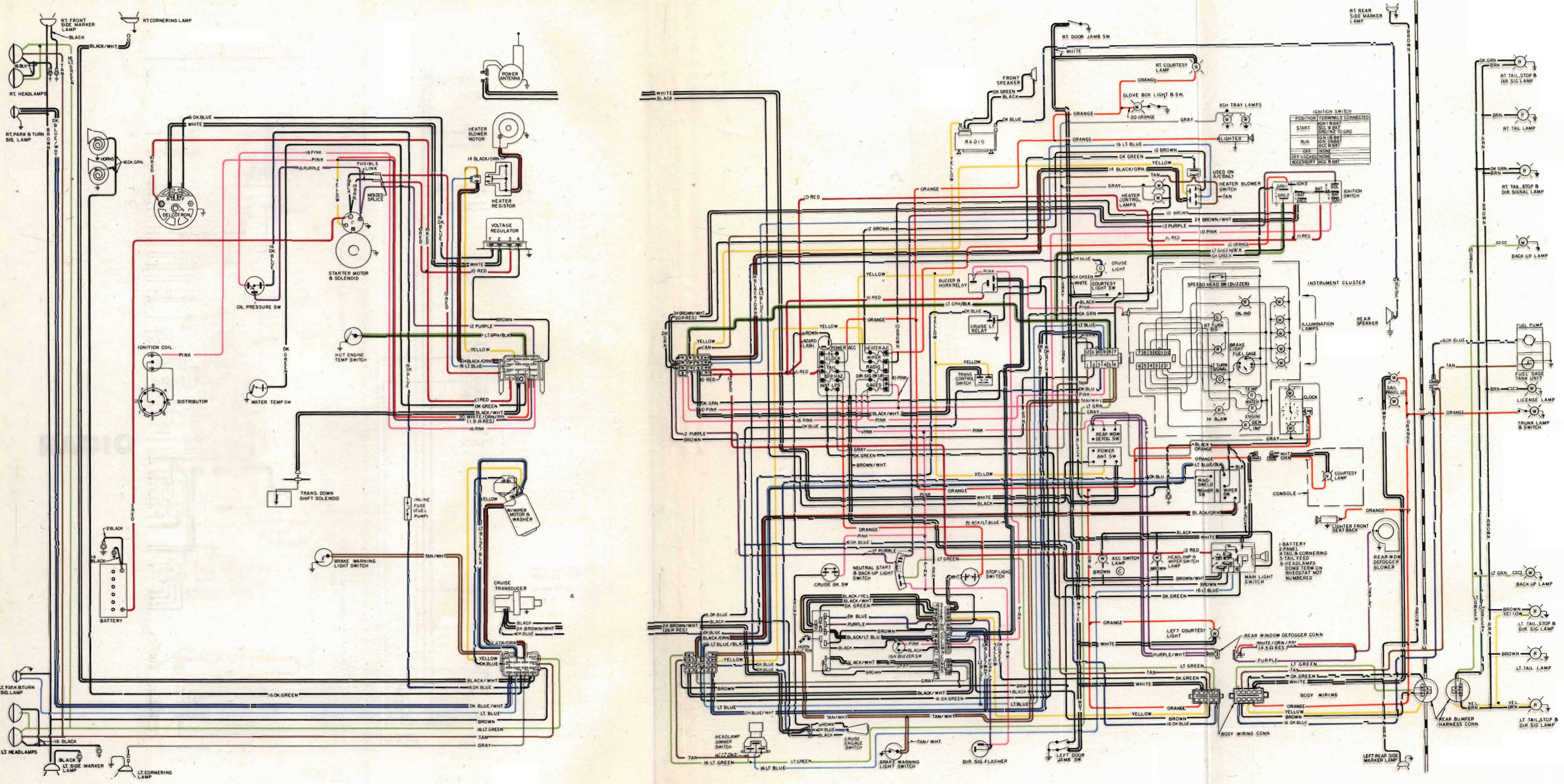
Figure 120-127 Wiring Circuit Diagram - Riviera
