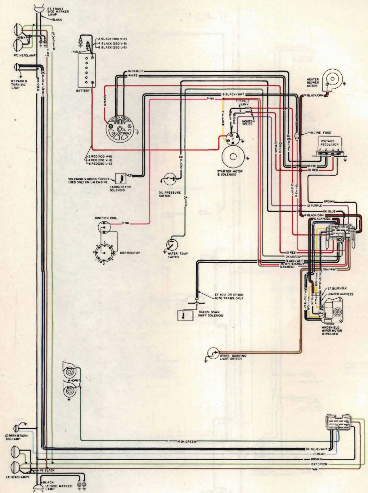
Figure 120-125 Wiring Circuit Diagram - 43-44000
