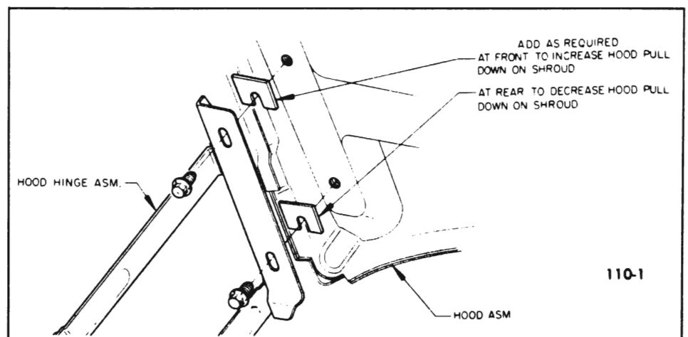
Figure 110-11 Shimming Hood to Hood Hinge
