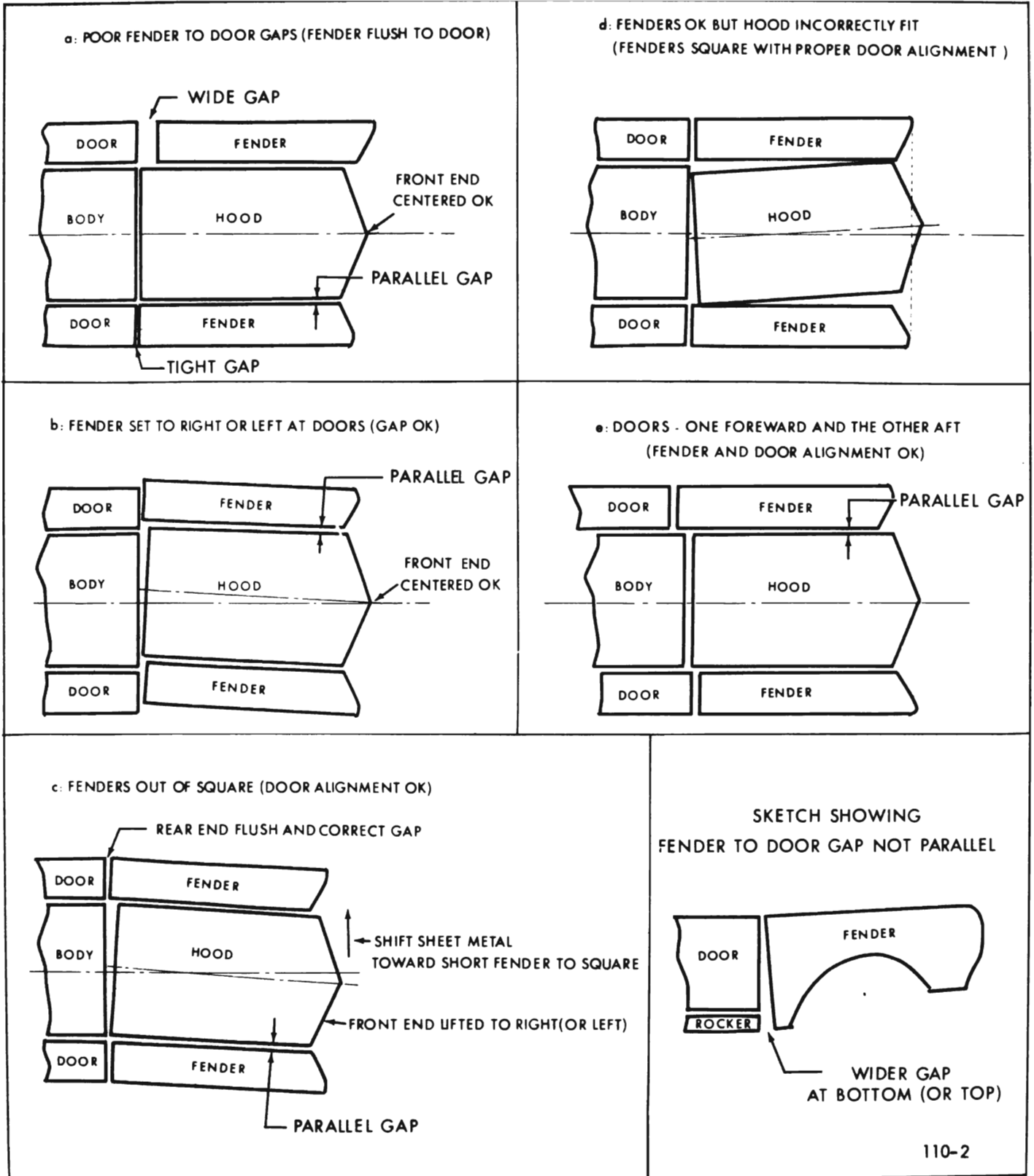
Figure 110-12 Chassis Sheet Metal Alignment
