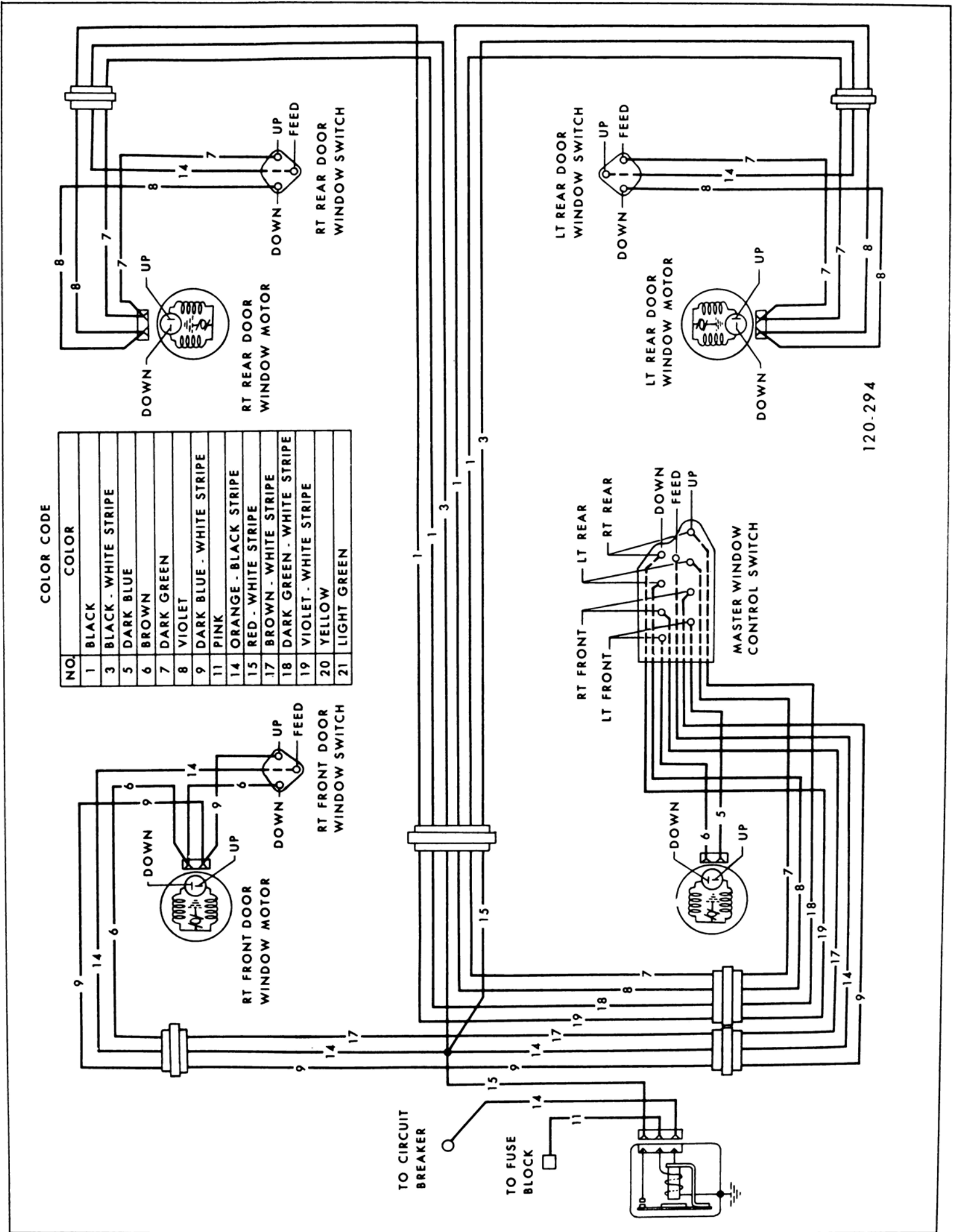
Figure 120-87—Power Window Wiring Diagram 43-44000 Series
