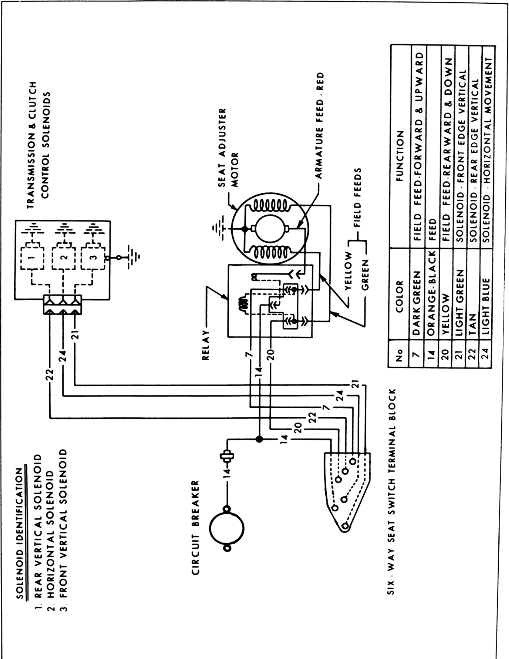
Figure 120-91—Six-Way Power Seat Wiring Diagram
