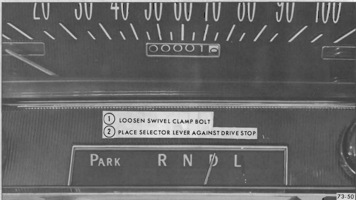
73-1 SUPER TURBINE 300 TRANSMISSION LINKAGE ADJUSTMENT (Column Shift) 43-44000 SERIES
