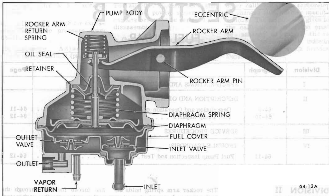
Figure 64-5—Fuel Pump
