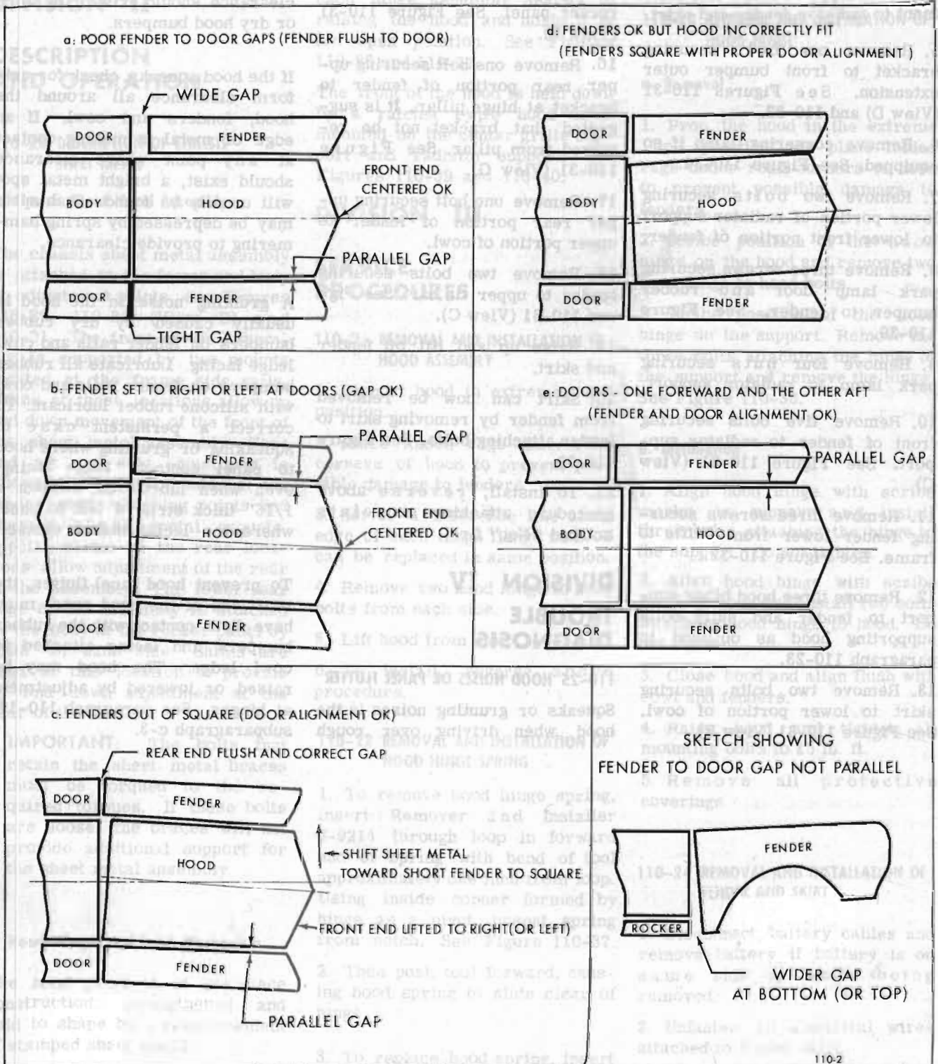
Figure 110-28—Chassis Sheet Metal Alignment
