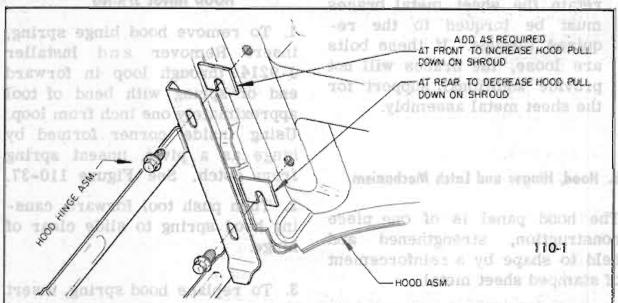
Figure 110-27—Shimming Hood Hinge to Hood
