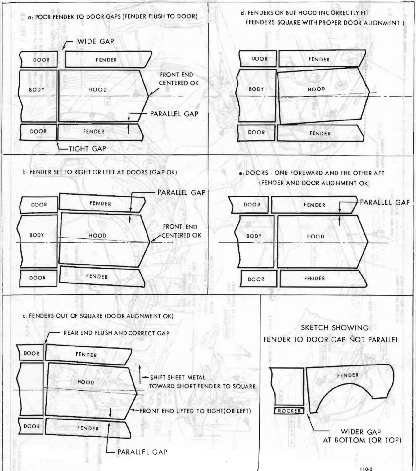
Figure 110-15—Chassis Sheet Metal Alignment
