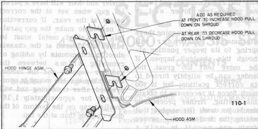
Figure 110-14—Shimming Hood Hinge to Hood
