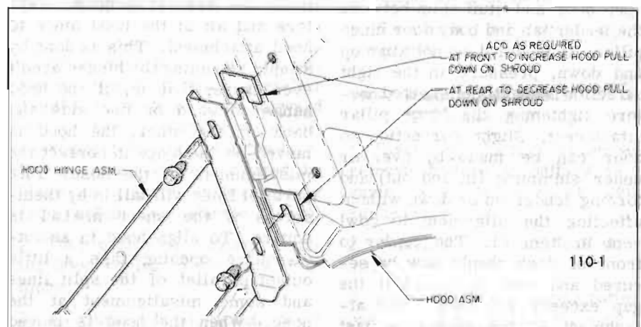
Figure 110-1—Shimming Hood Hinge to Hood
