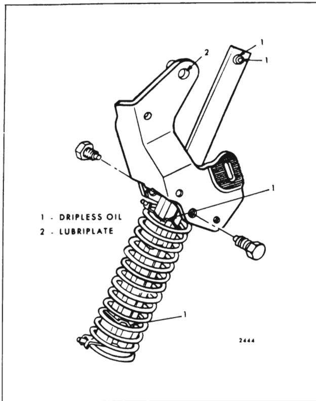
Fig. 2-15—Convertible Top Linkage - "F" Styles
