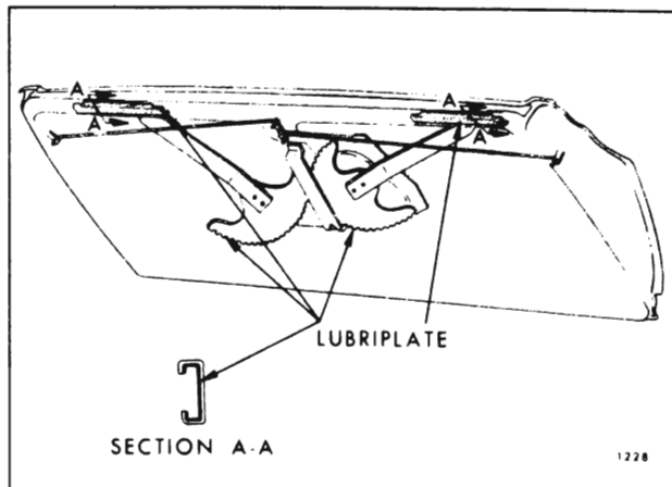
Fig. 2-11—Tail Gate Window Regulator and Cams (Station Wagons)
