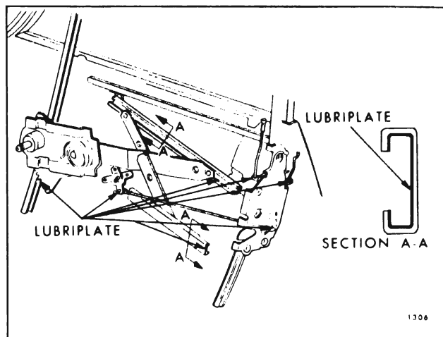
Fig. 2-7 — Door Window Regulator and Cams On Styles With Upper Frames
