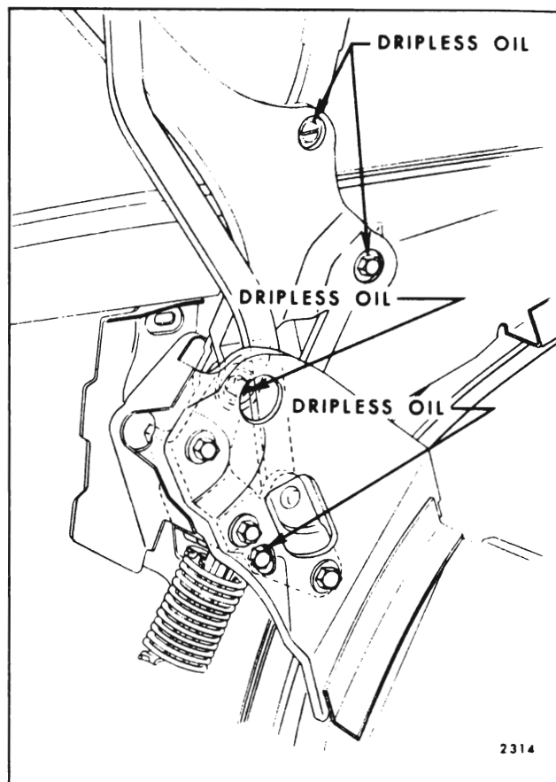
Fig. 2-14 — Convertible Top Linkage - "A" Styles (Manual Type Shown)
