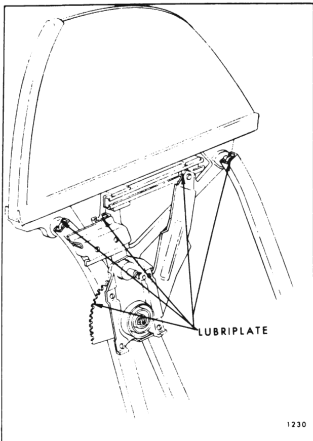
Fig. 2-9—Rear Quarter Window Regulator Cams and Guides
