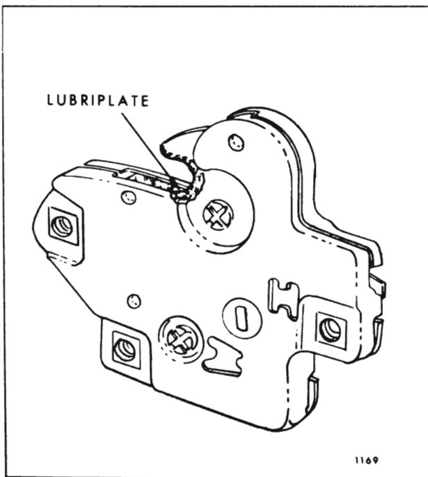
Fig. 2-10—Rear Compartment Lid Lock
