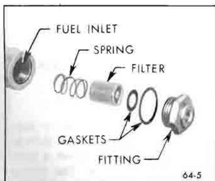
Figure 64-5—Fuel Filter Parts - V-6
