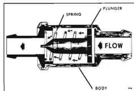
Figure 64-6—Positive Crankcase Ventilator Valve
