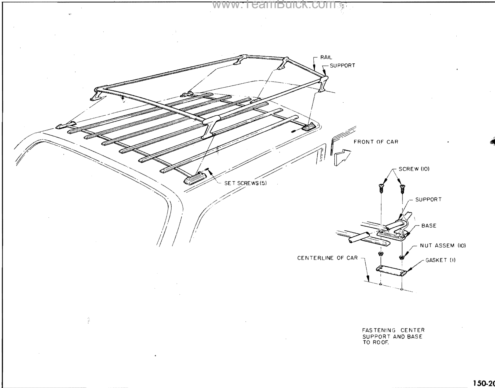
Figure 150-20—Roof Luggage Carrier
