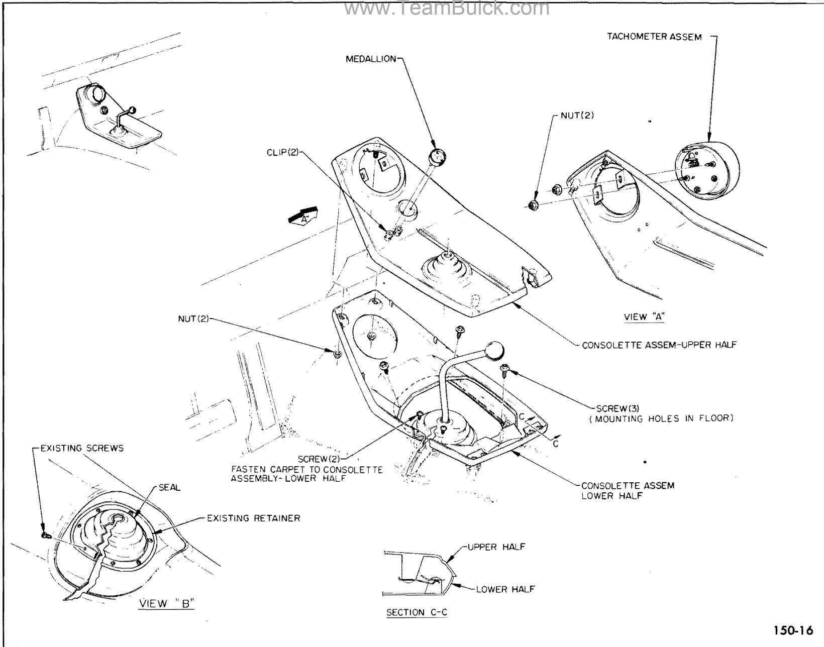
Figure 150-16—Tachometer Installation Skylark Gran Sport 3 or 4 Speed with Consolette
