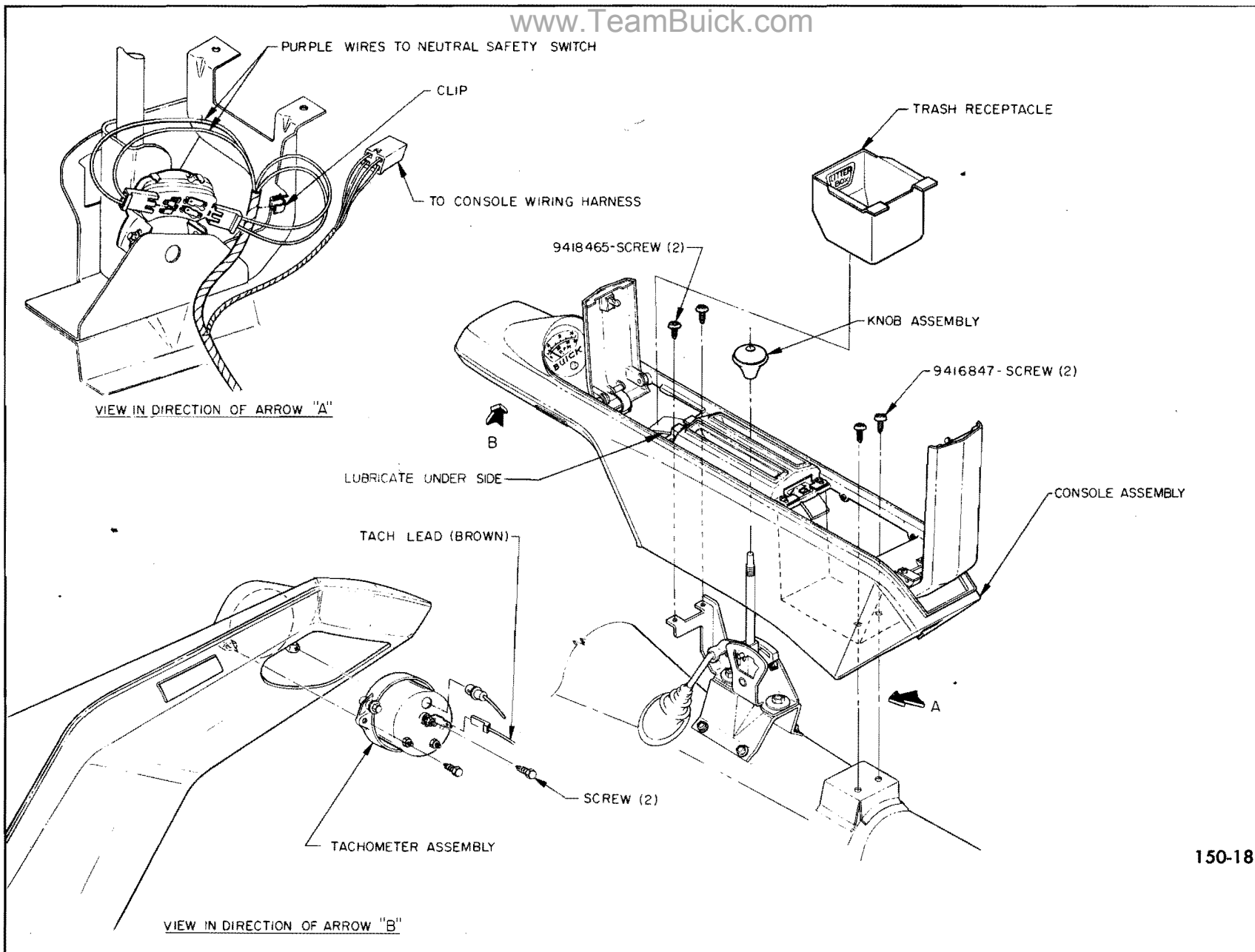
Figure 150-18—Tachometer Installation Upper Series Automatic with Console Shift
