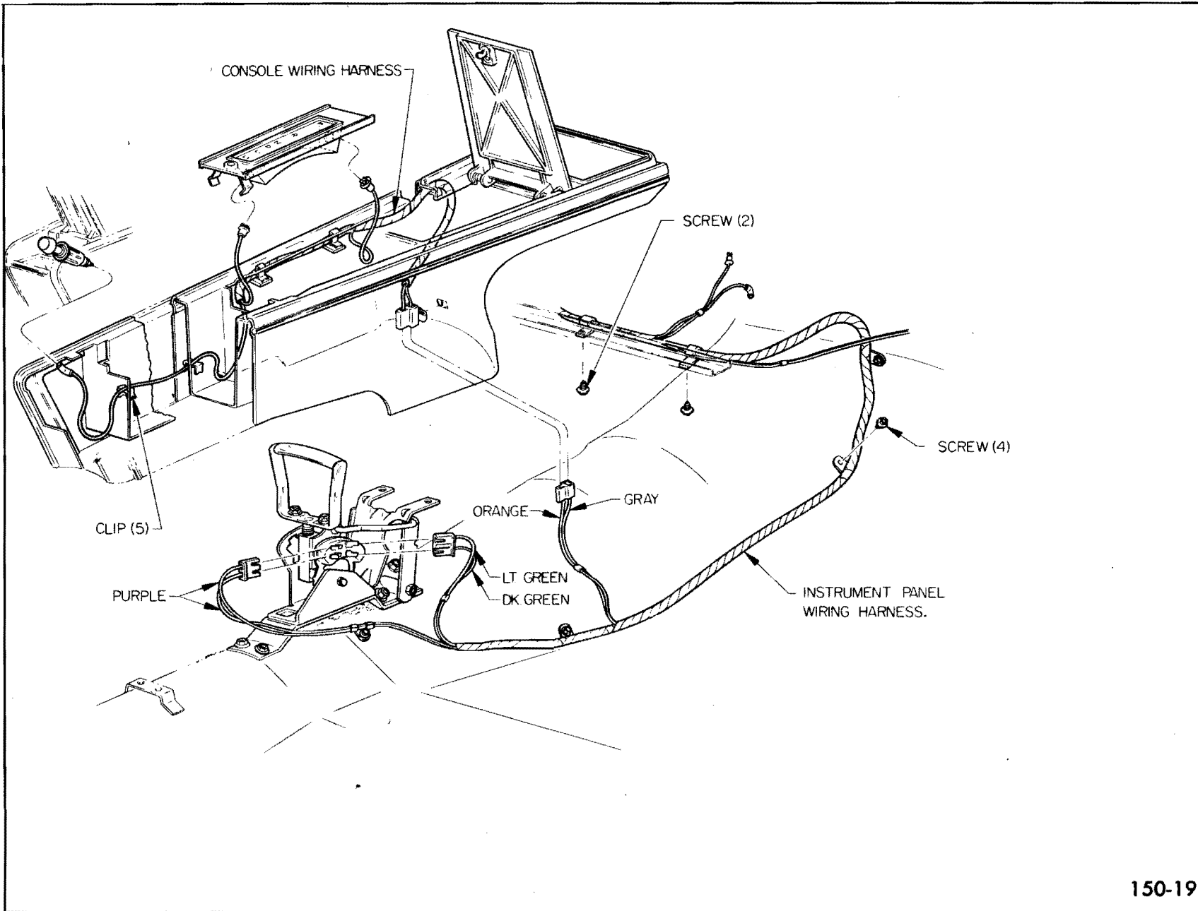
Figure 150-19—Console Information - 49000 Series
