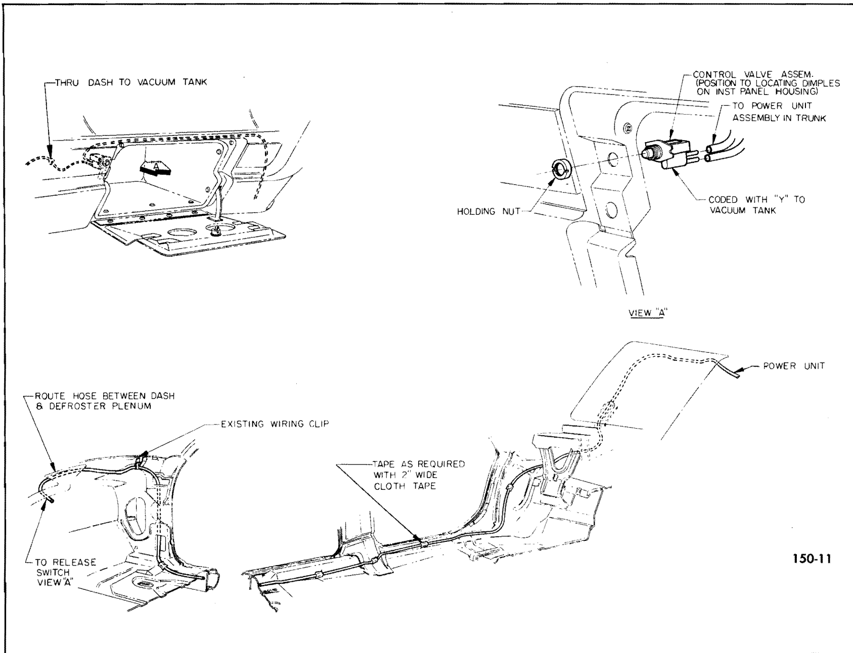
Figure 150-11—Vacuum Trunk Release Line Routing 45-46-48000 Series
