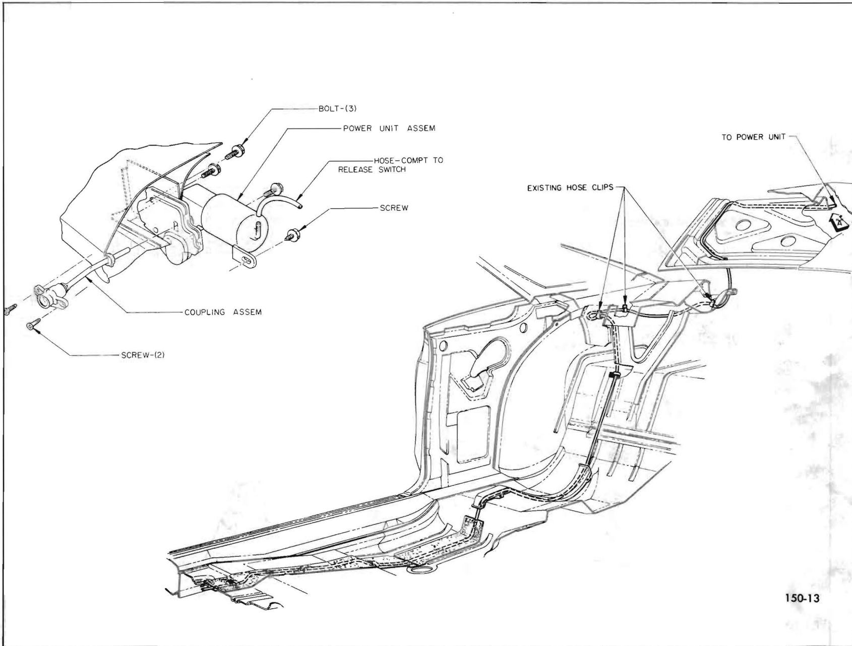
Figure 150-13—Vacuum Trunk Release Line Routing 49000 Series
