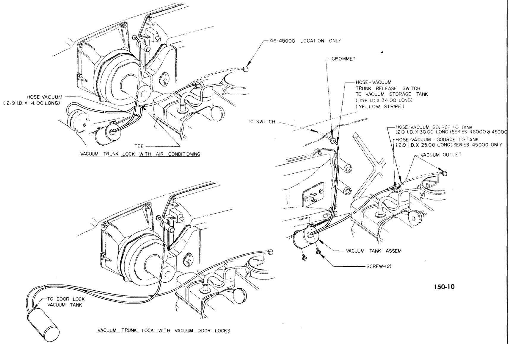
Figure 150-10—Vacuum Trunk Release Tank Installation 45-46-48000 Series
