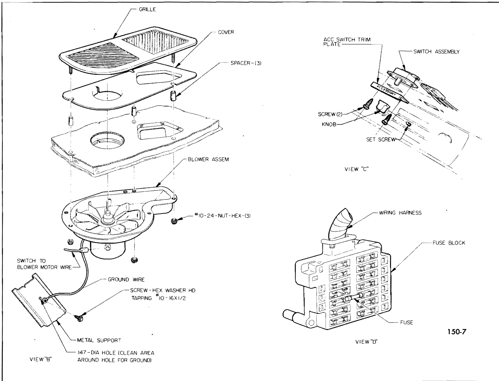
Figure 150-7—Rear Window Defroster 45-46-48000 Series
