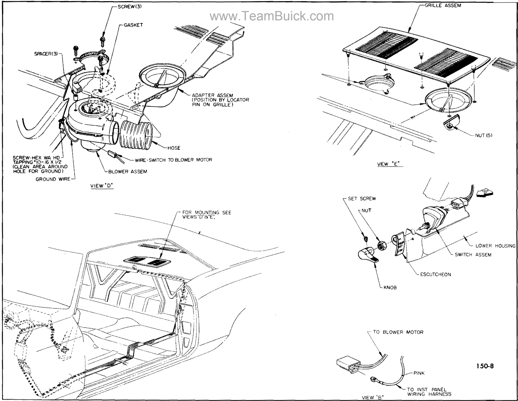
Figure 150-8—Rear Window Defroster 49000 Series
