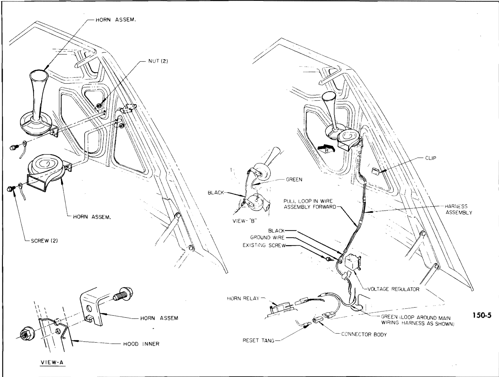
Figure 150-5—Four Note Horns 49000 Series
