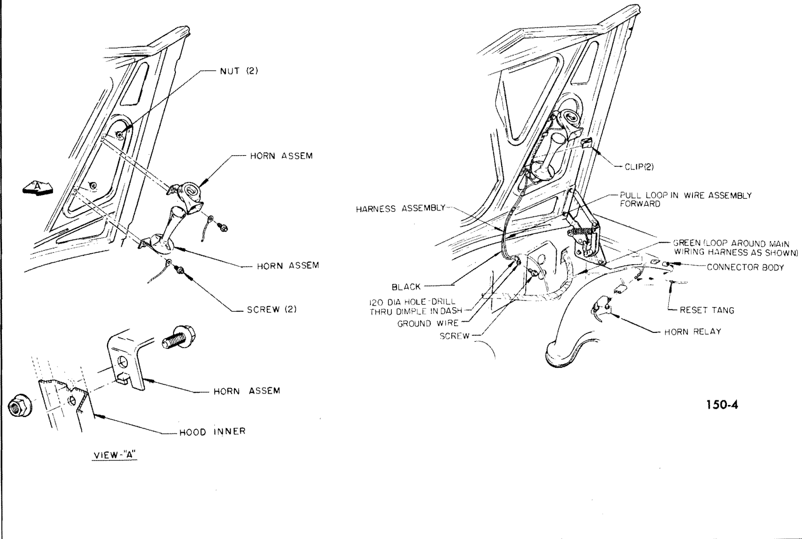
Figure 150-4—Four Note Horns 45-46-48000 Series
