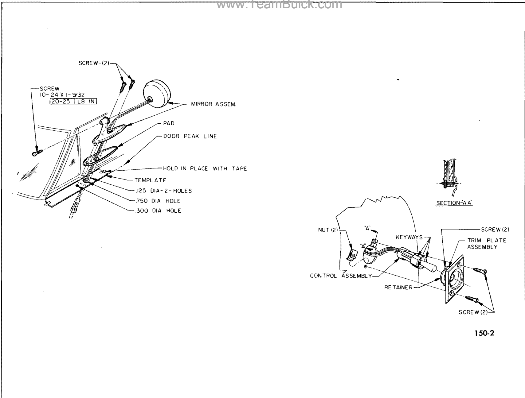
Figure 150-2—Remote Control Outside Rear View Mirror 45-46-48000 Series
