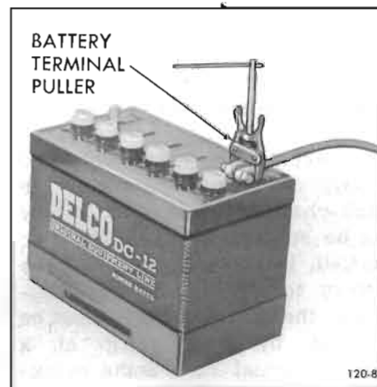
Figure 120-8—Using a Battery Terminal Puller
