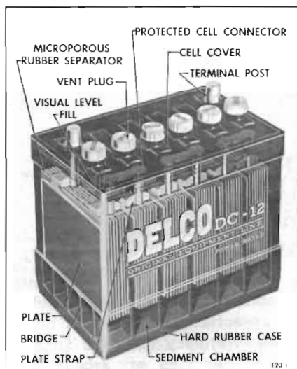
Figure 120-1—Battery - Special, Skylark and LeSabre
