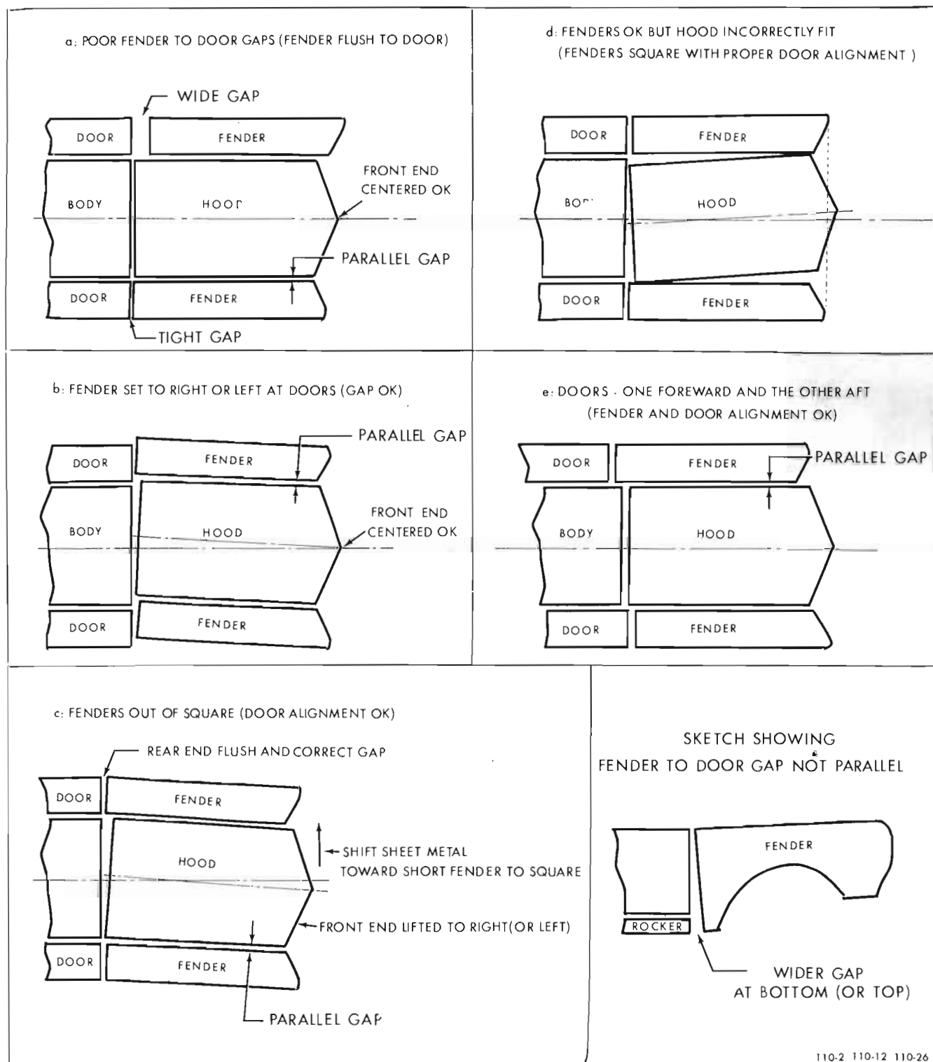
Figure 110-12—Chassis Sheet Metal Alignment
