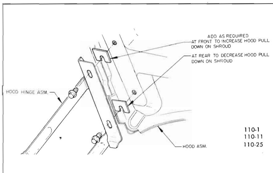
Figure 110-11—Shimming Hood Hinge to Hood
