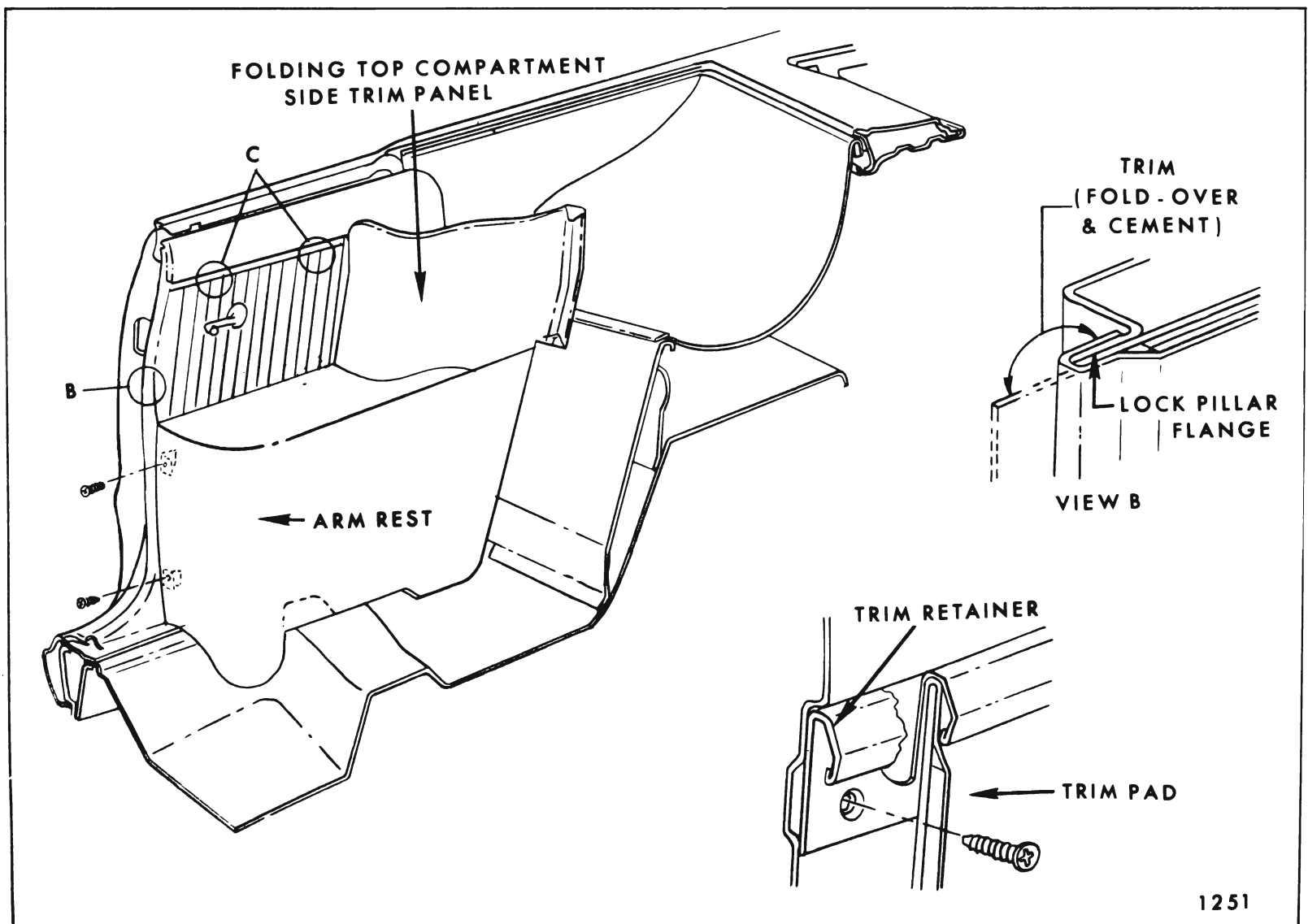
Fig. 8-9—Rear Quarter Trim Assembly - Convertible Styles
