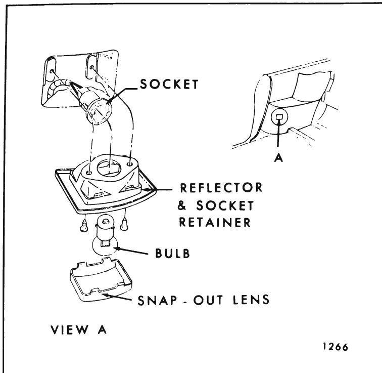
Fig. 8-8—Rear Quarter Arm Rest Courtesy Lamp
