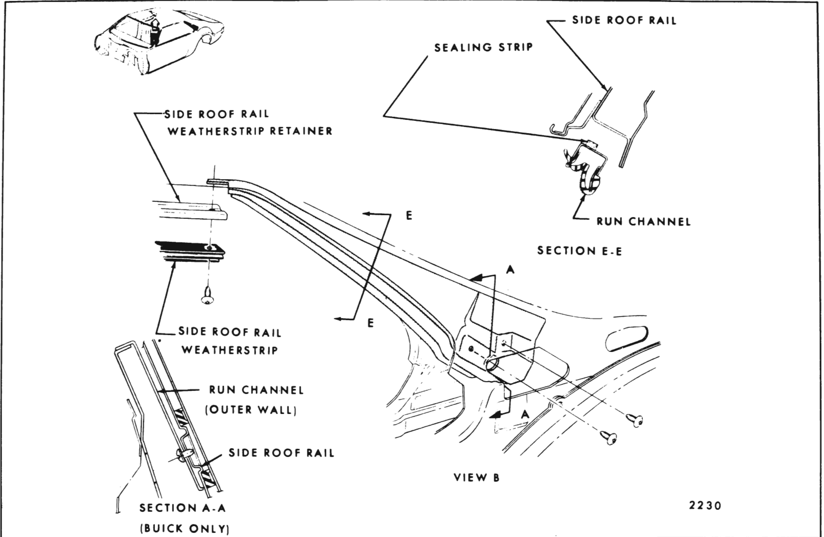
Fig. 8-65—Rear Quarter Window Upper Glass Run Channel - "E" Body Styles
