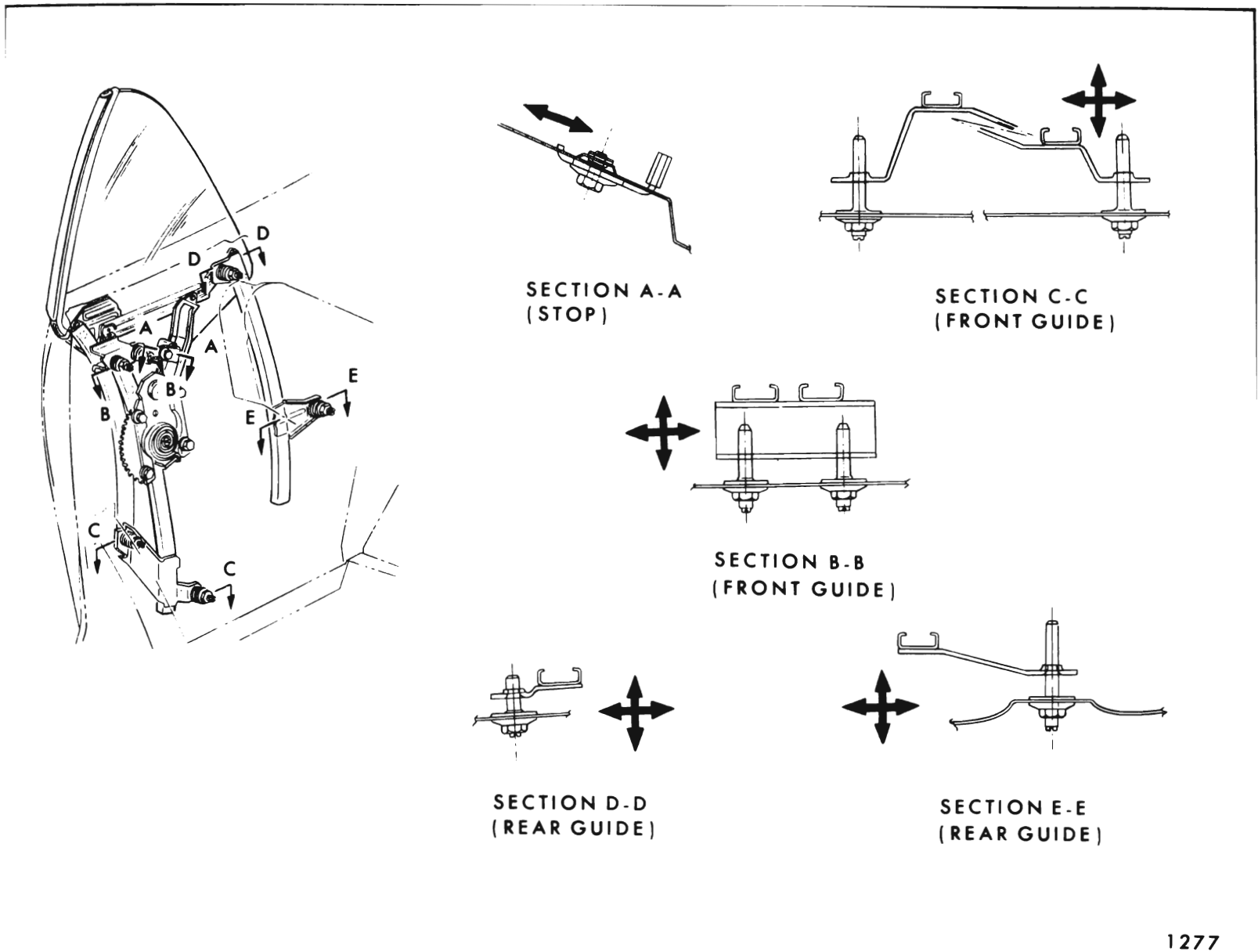
Fig. 8-62—Rear Quarter Window Adjustments - "Z-67" Styles (Arrows Indicate Adjustment Direction Available)
