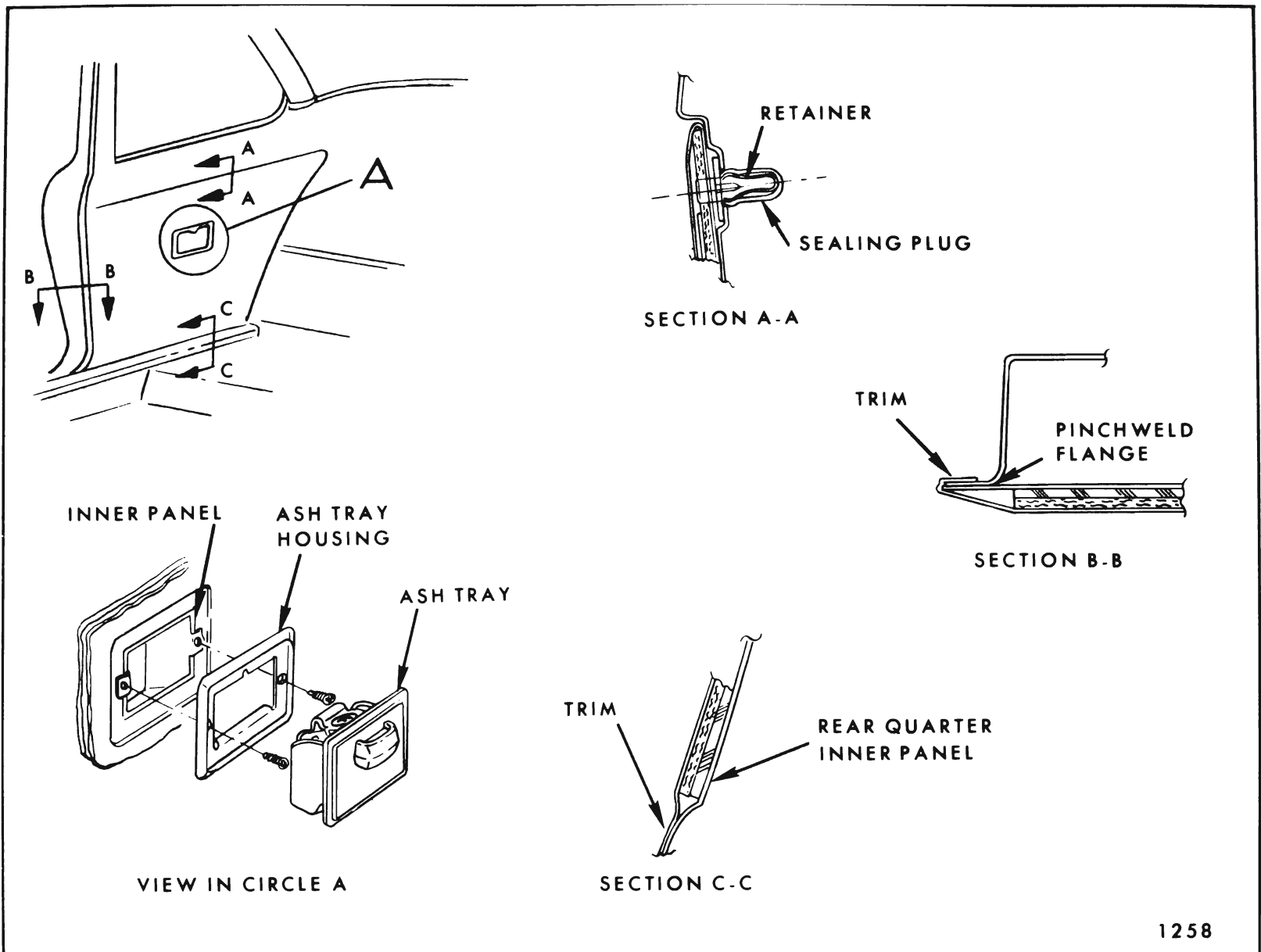
Fig. 8-6—Rear Quarter Trim Assembly - "Z" Body Styles
