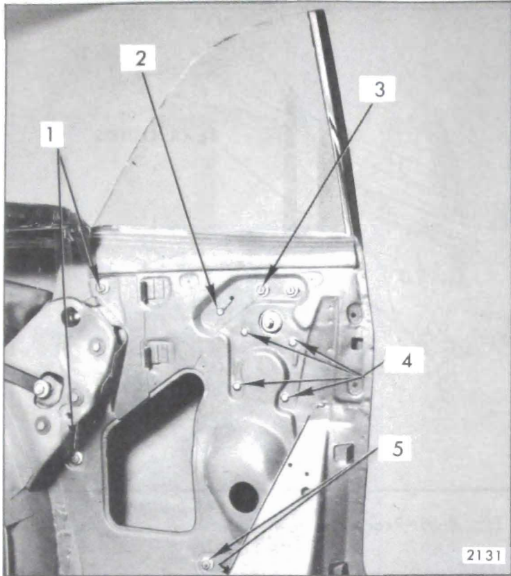
Fig. 8-52—Rear Quarter Hardware - "A-67" Style
