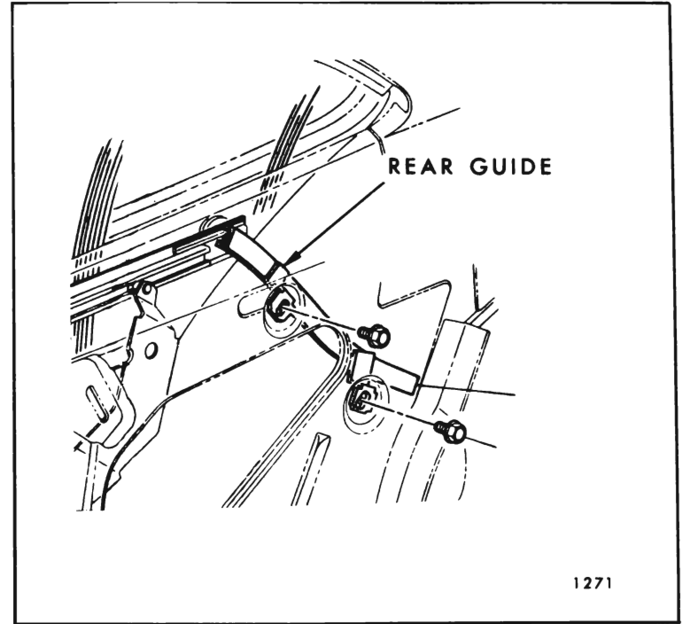
Fig. 8-58—Rear Quarter Window Rear Guide Assembly - "Z-37" Styles
