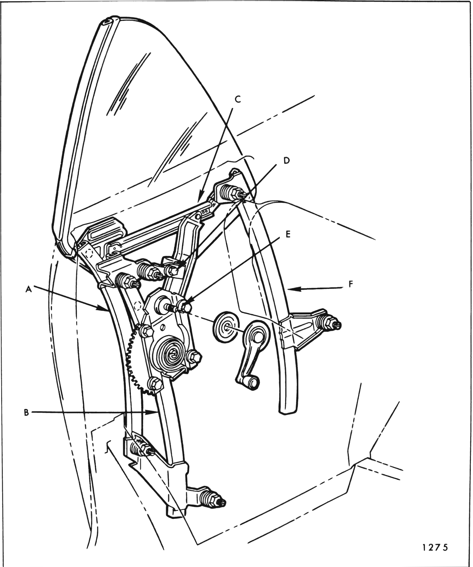
Fig. 8-38—Rear Quarter Hardware - "67" Style
