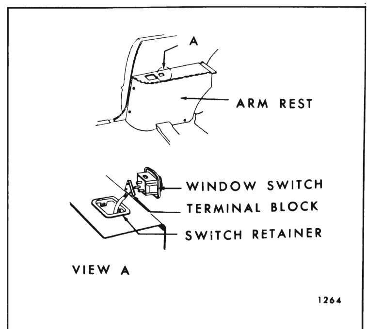
Fig. 8-3—Rear Quarter Arm Rest Window Switch
