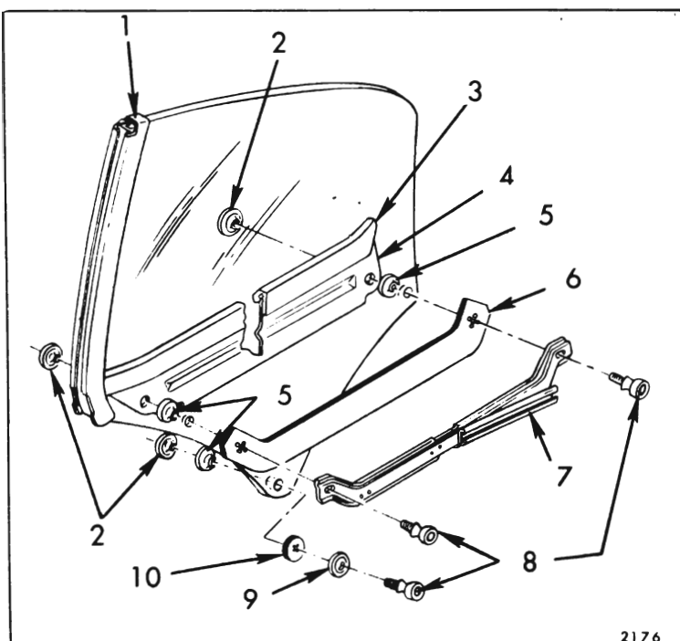
Fig. 8-50—Rear Quarter Window Assembly - Chevrolet "B-47" Style
