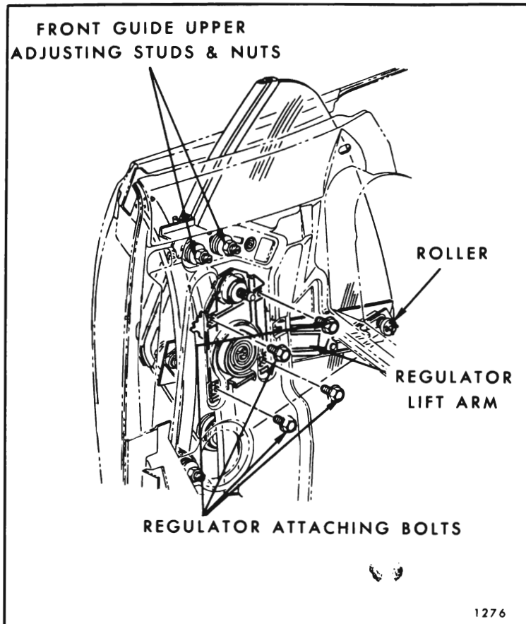
Fig. 8-63—Rear Quarter Window Regulator Attachment - "Z-67" Styles
