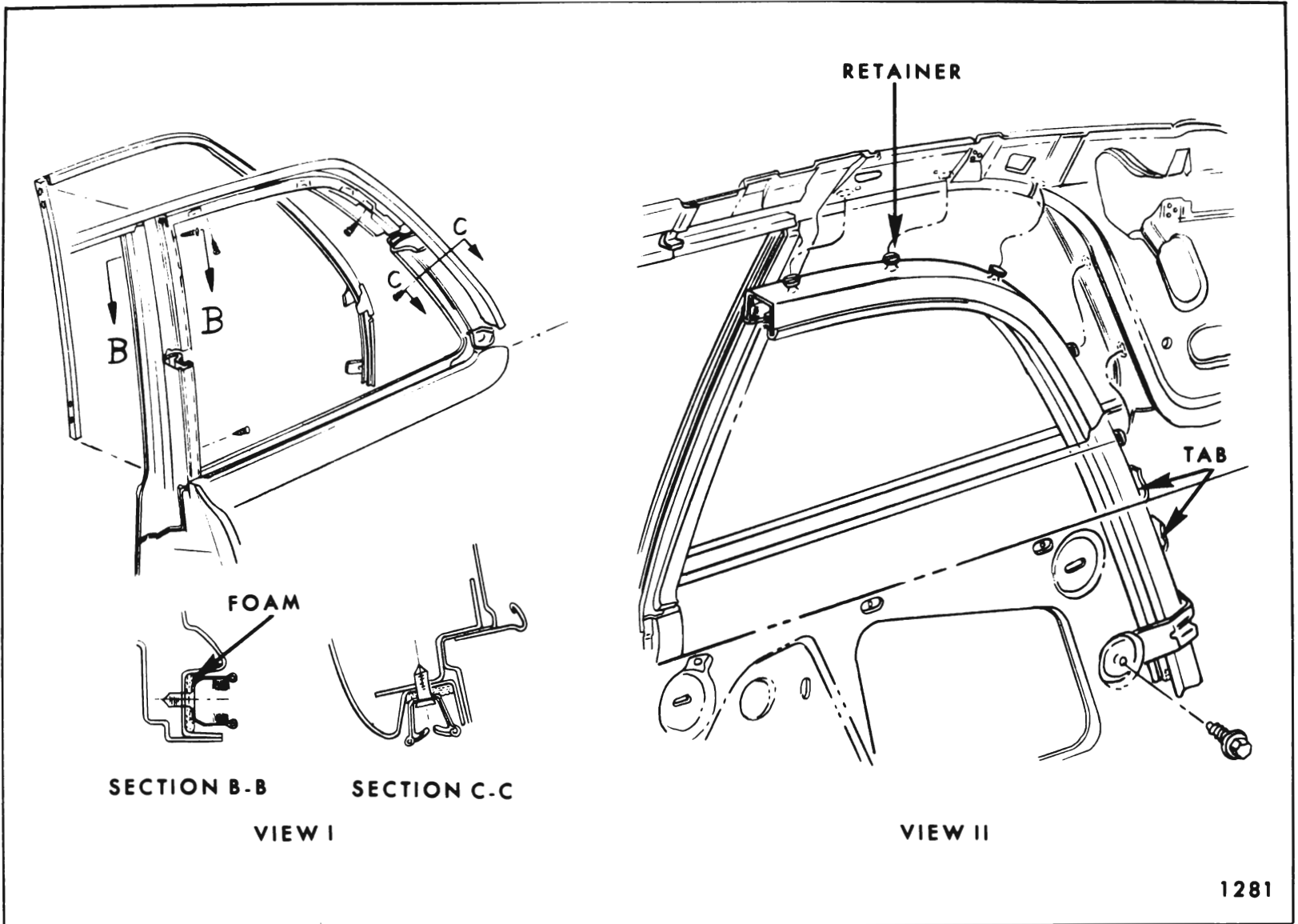
Fig. 8-44—Rear Quarter Window Glass Run Channels - Typical of All Closed Styles
