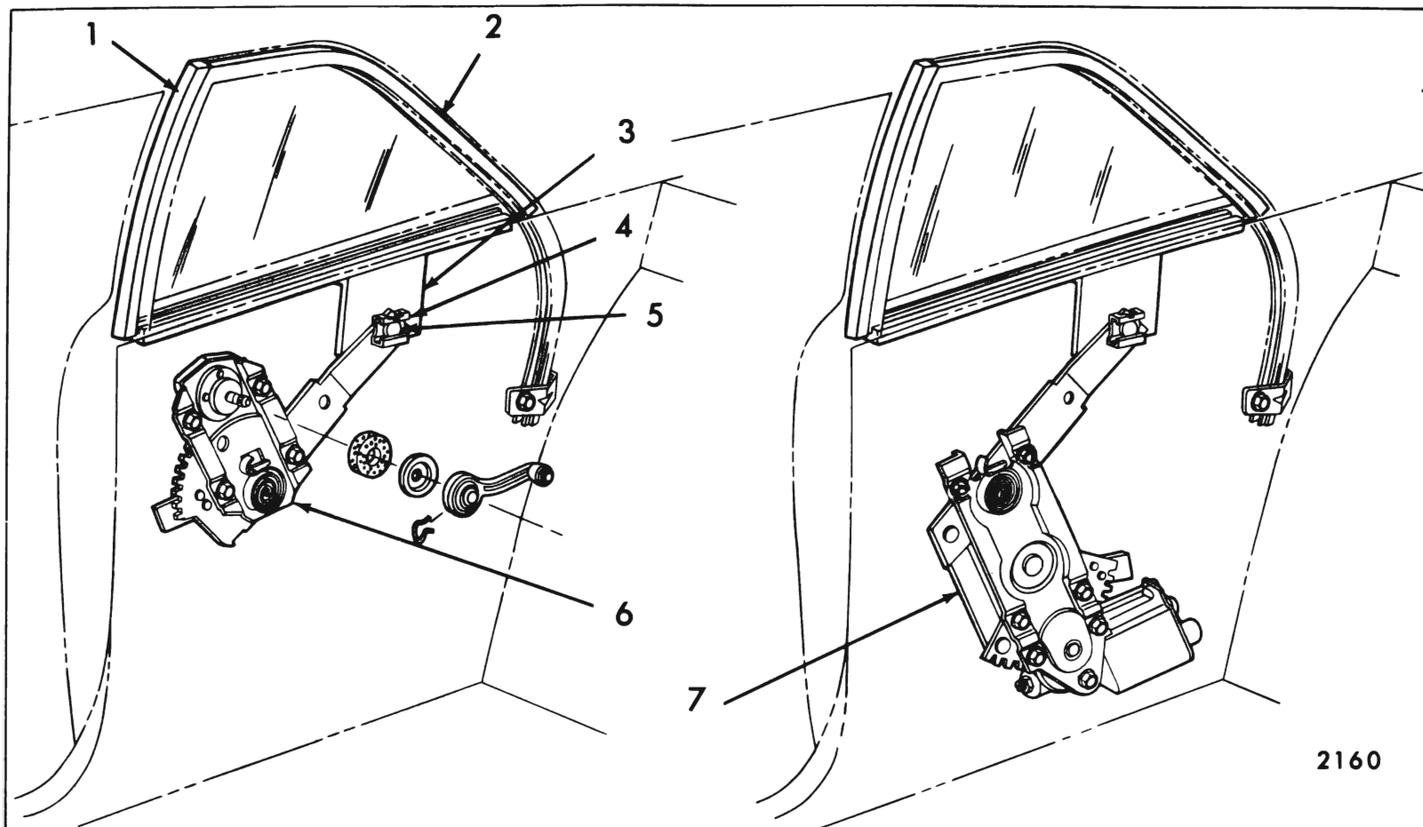
Fig. 8-29—Rear Quarter Hardware - "A-11" Style
