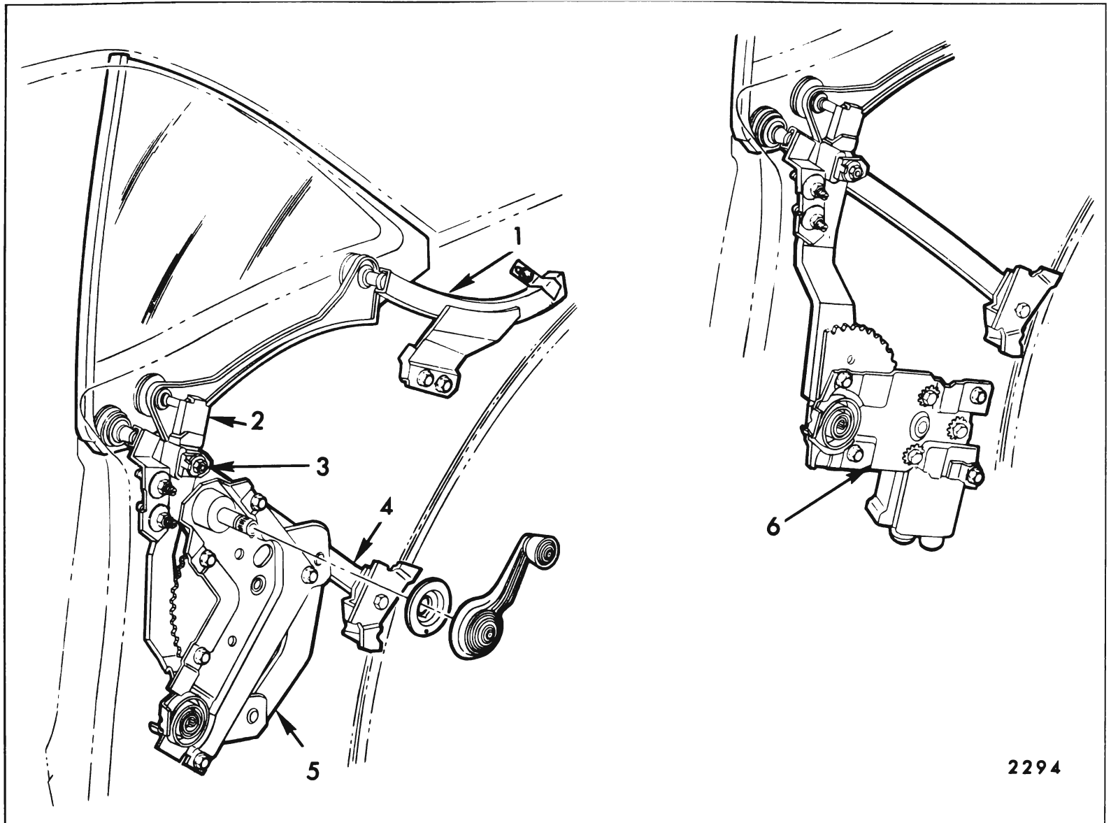
Fig. 8-34—Rear Quarter Hardware - Oldsmobile "E" Body
