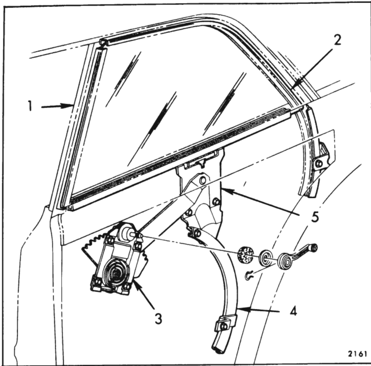
Fig. 8-35—Rear Quarter Hardware - "X-11" Style
