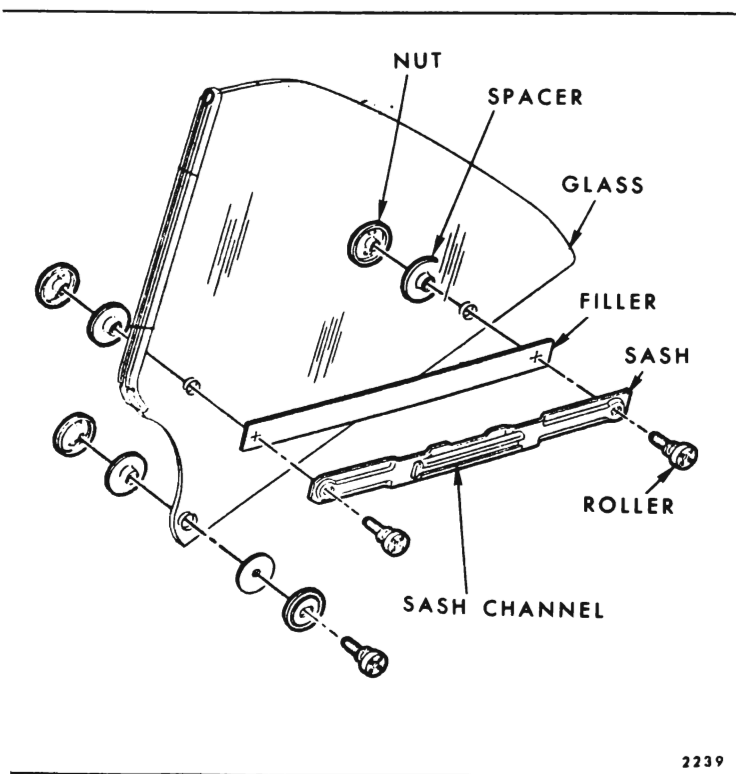
Fig. 8-57—Rear Quarter Window Assembly - "X-37" Style
