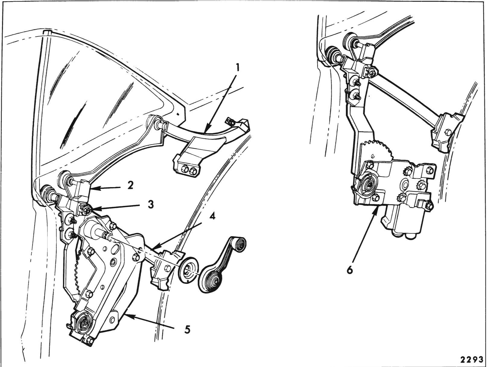
Fig. 8-33—Rear Quarter Hardware - Buick "E" Styles
