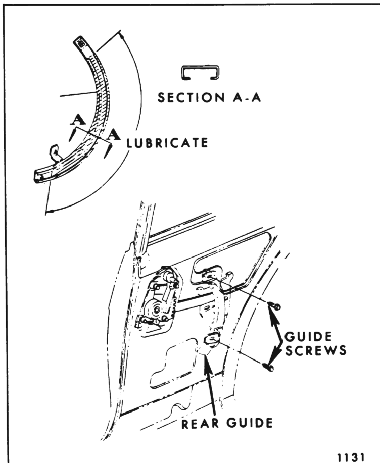
Fig. 8-46—Rear Quarter Window Guide - "X-11" Styles
