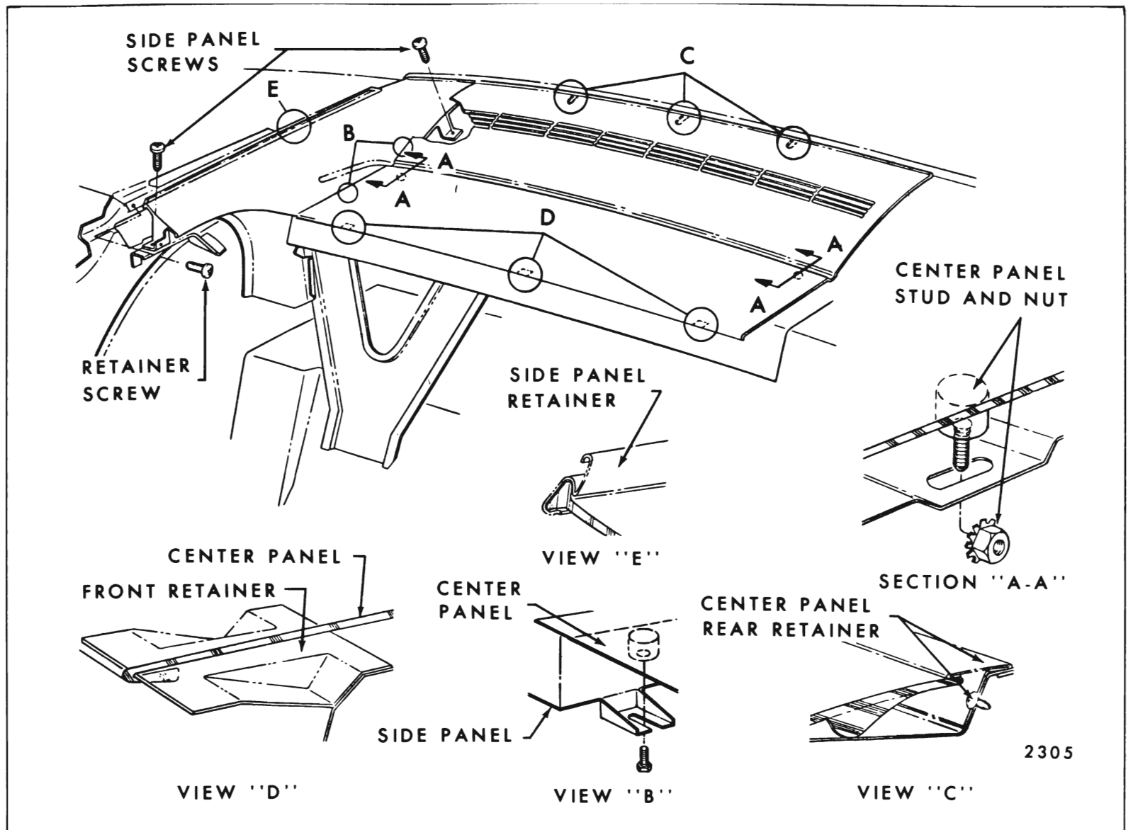
Fig. 8-12—Compartment Shelf Trim - Buick "E" Body
