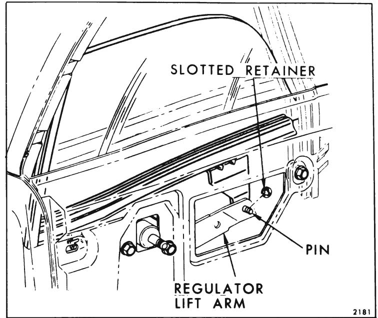
Fig. 8-41—Rear Quarter Window Attachment - "B-11" Styles
