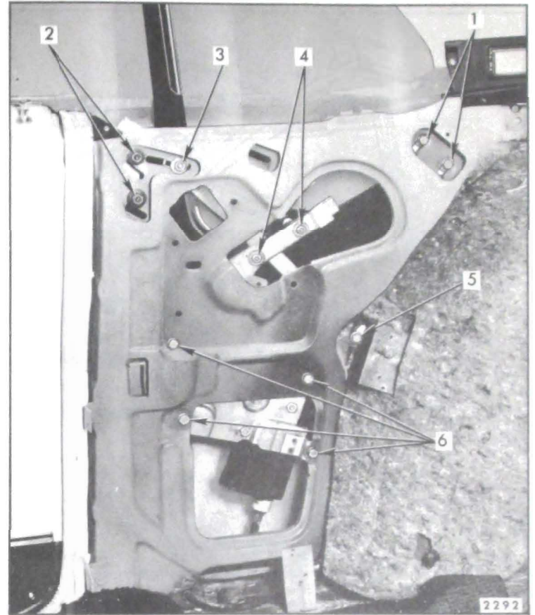
Fig. 8-54—Rear Quarter Hardware - "E" Body
