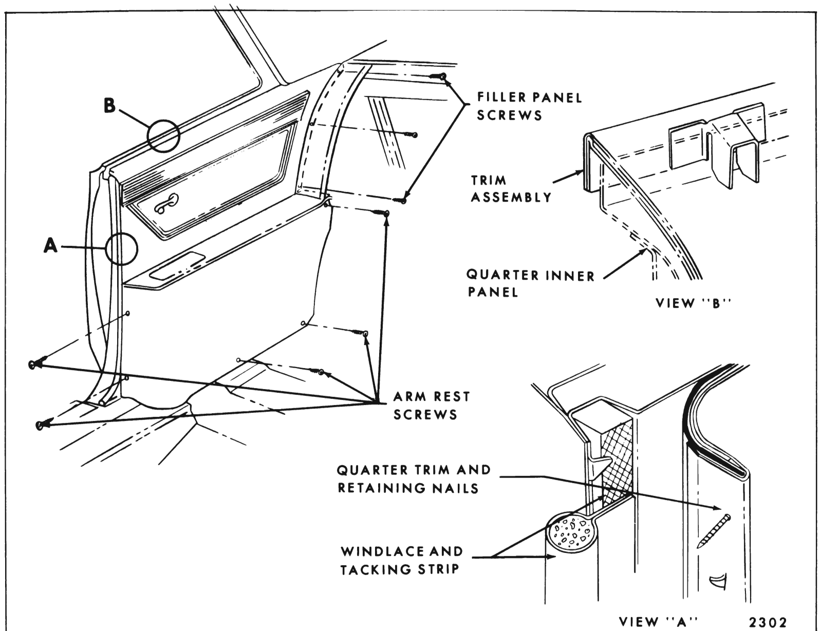
Fig. 8-2—Rear Quarter Trim Assembly (Hang-On Type)
