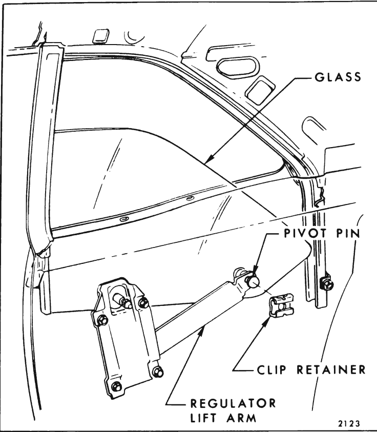
Fig. 8-39—Rear Quarter Window Attachment - "A-07" Styles
