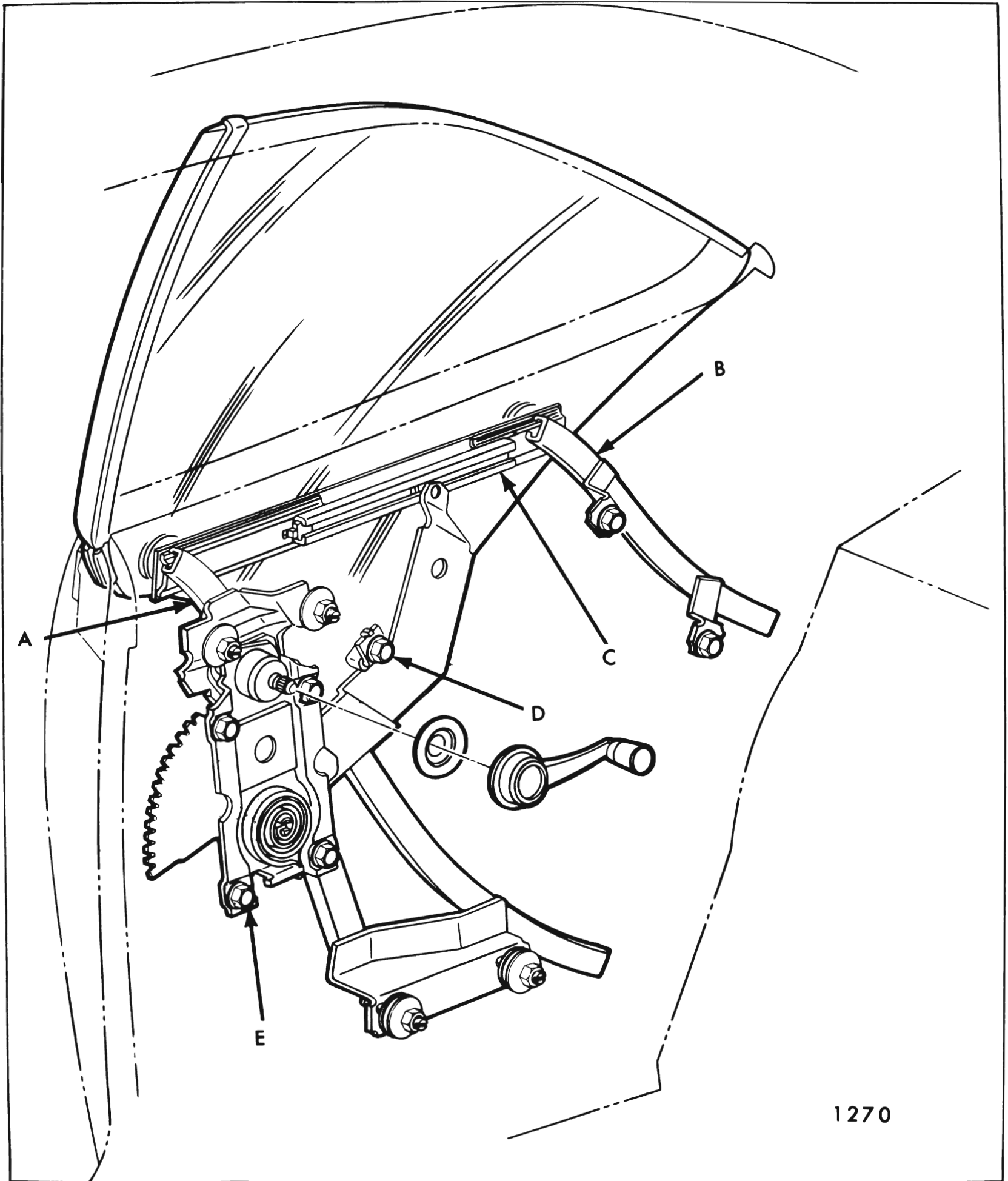
Fig. 8-37—Rear Quarter Hardware - "37" Styles
