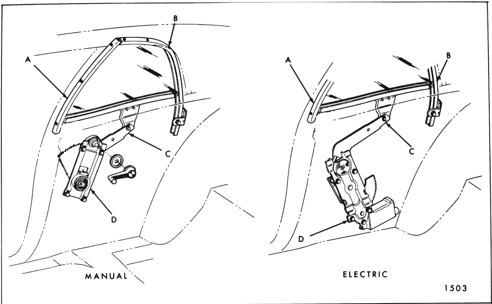
Fig. 8-27—Rear Quarter Window Hardware - "B-11" Styles
