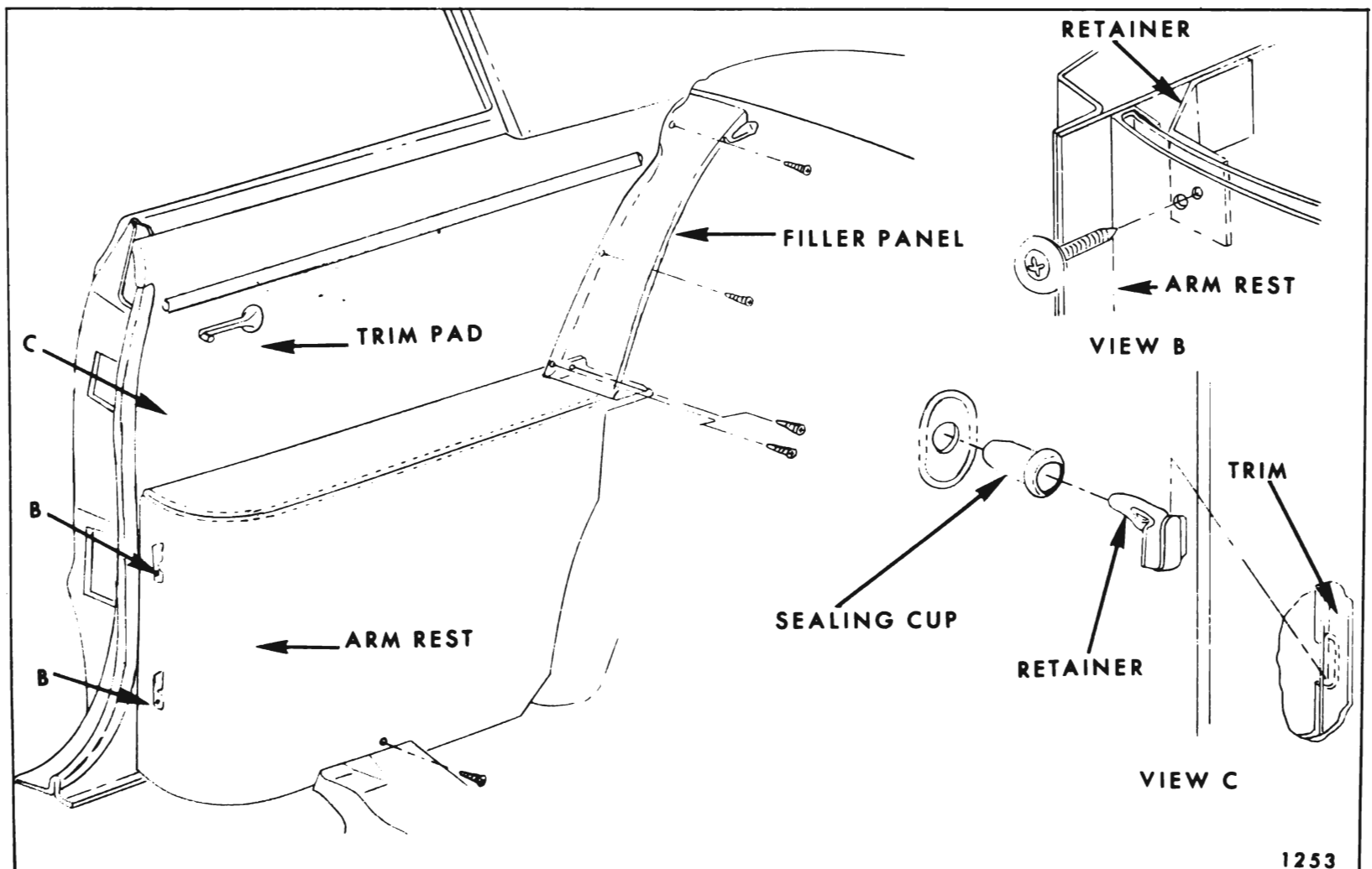
Fig. 8-1—Rear Quarter Trim Assembly (Insert Type)
