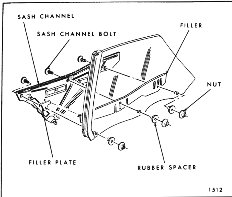
Fig. 8-49—Rear Quarter Window Assembly - "B&C" - "37-57 and 67" Styles
