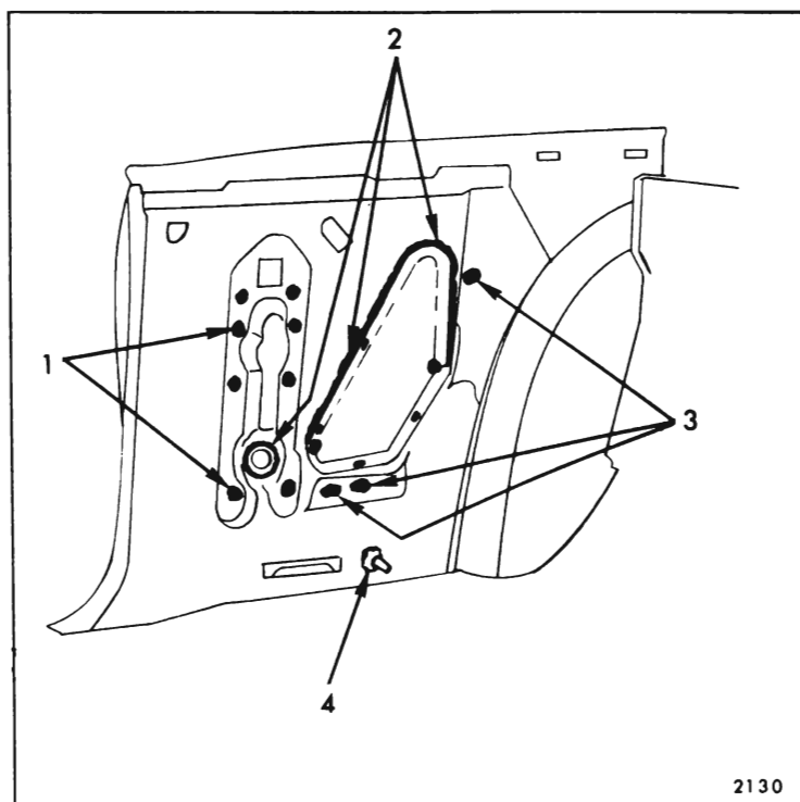
Fig. 8-26—Rear Quarter Inner Panel Sealing - "67" Styles
