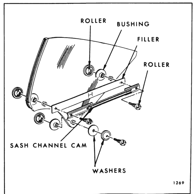
Fig. 8-59—Rear Quarter Window Assembly - "Z-37" Styles
