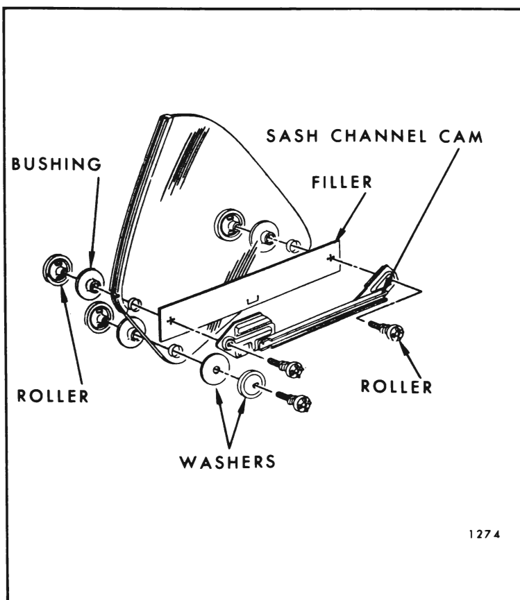
Fig. 8-61—Rear Quarter Window Assembly - "Z-67" Styles
