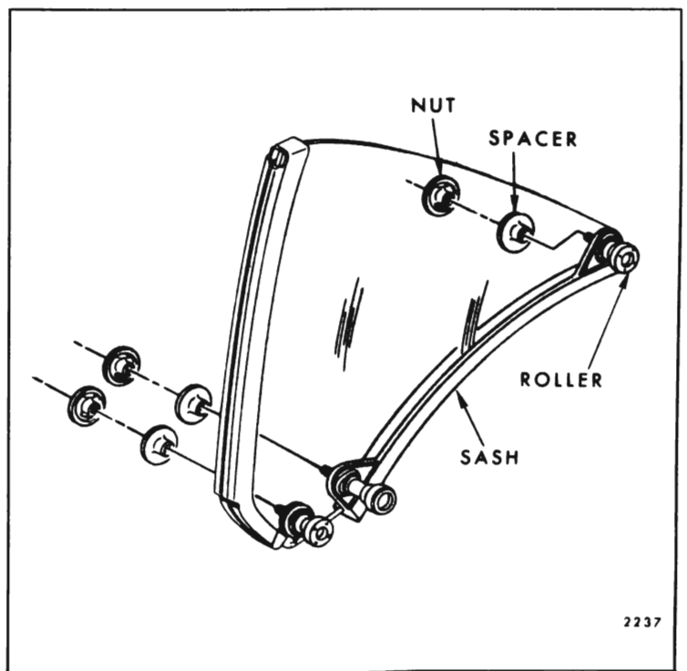
Fig. 8-55—Rear Quarter Window Assembly - "E" Body Styles
