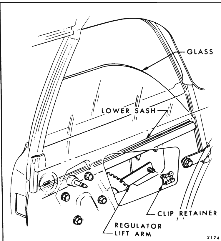
Fig. 8-40—Rear Quarter Window Attachment - "A-11" Styles
