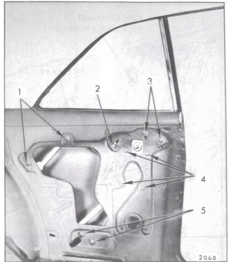
Fig. 8-51—Rear Quarter Hardware - "A-17" Style
