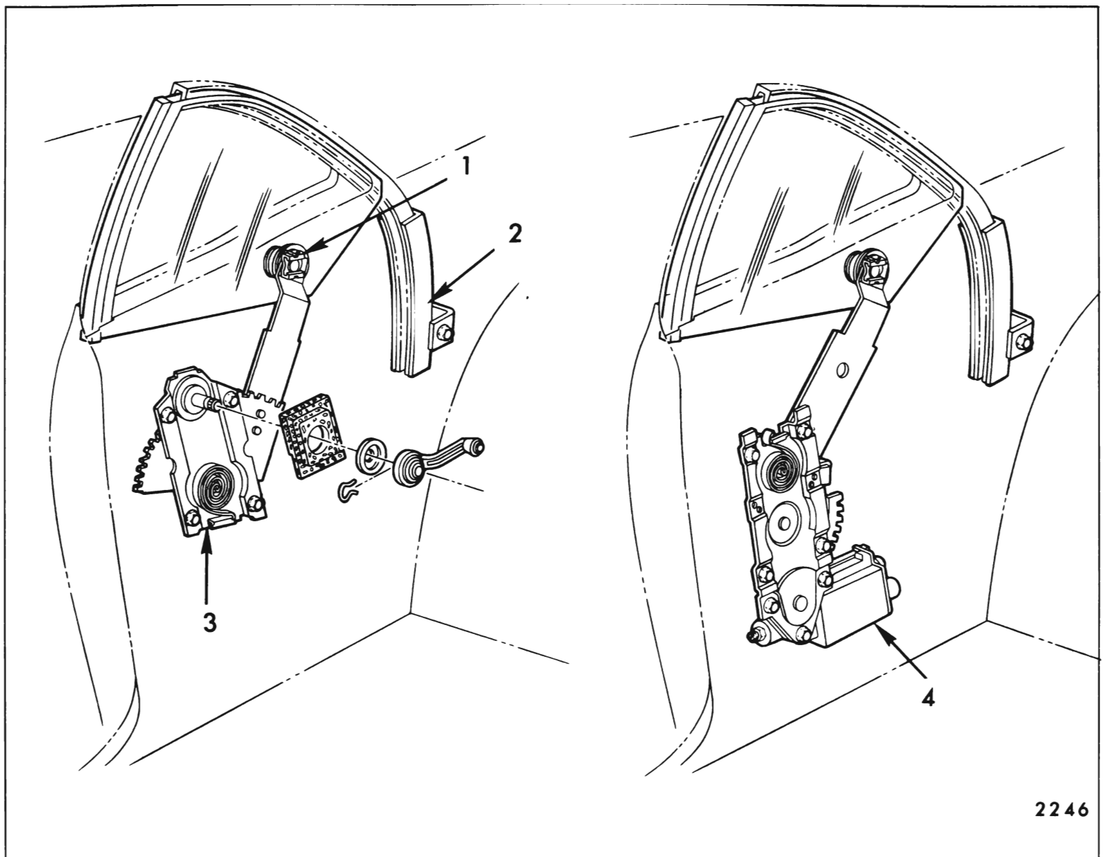
Fig. 8-30—Rear Quarter Hardware - "A-07" Style
