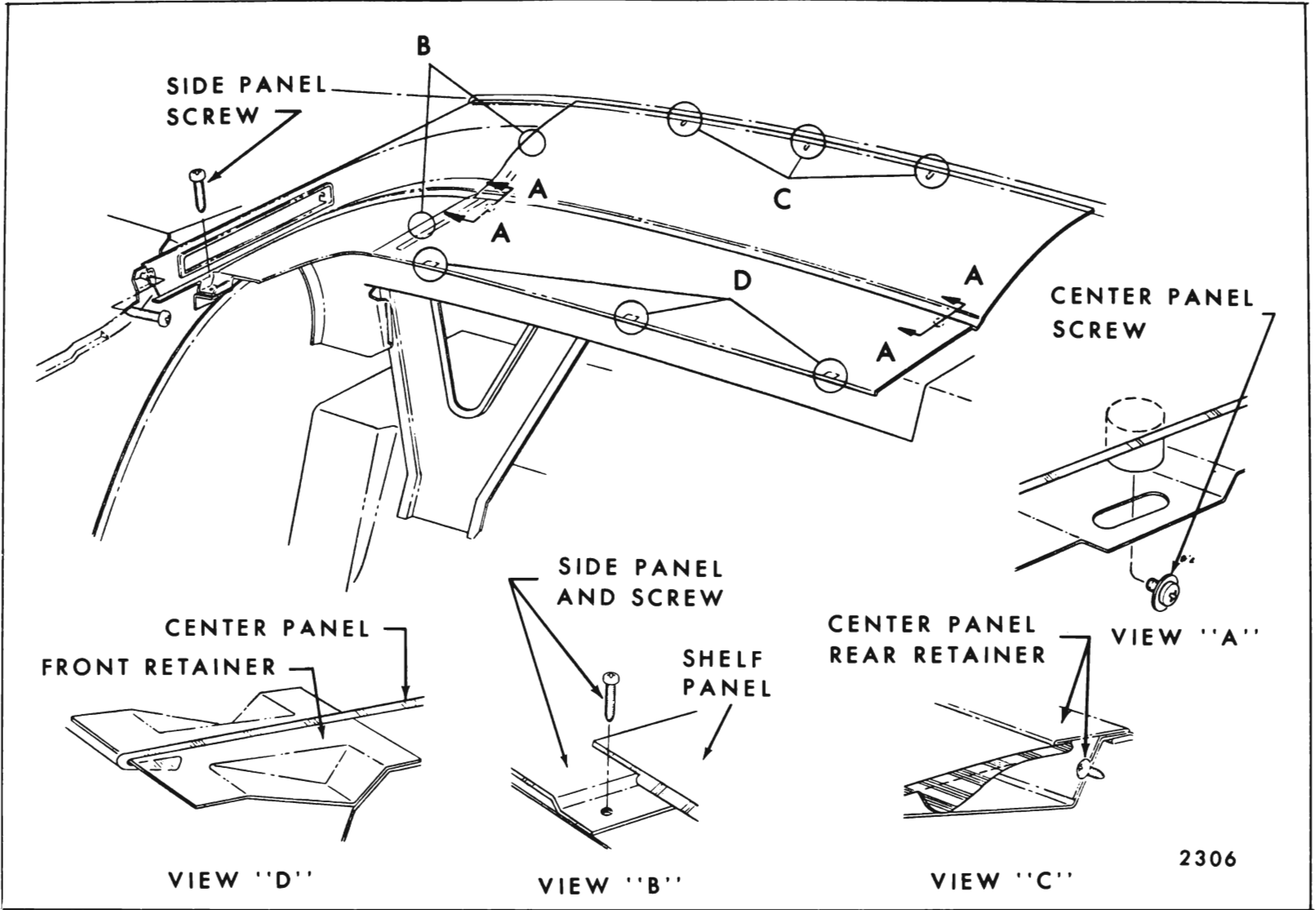
Fig. 8-13—Compartment Shelf Trim - Oldsmobile "E" Body
