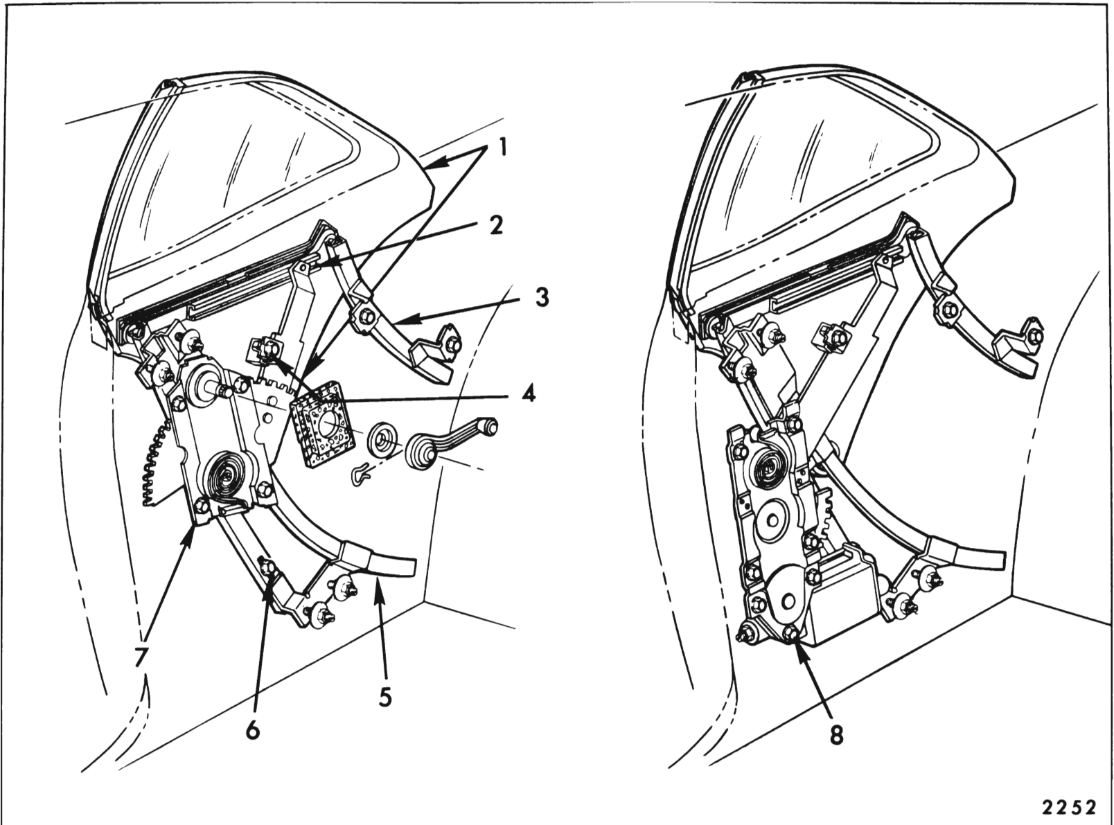
Fig. 8-31—Rear Quarter Hardware - "A-17" Style
