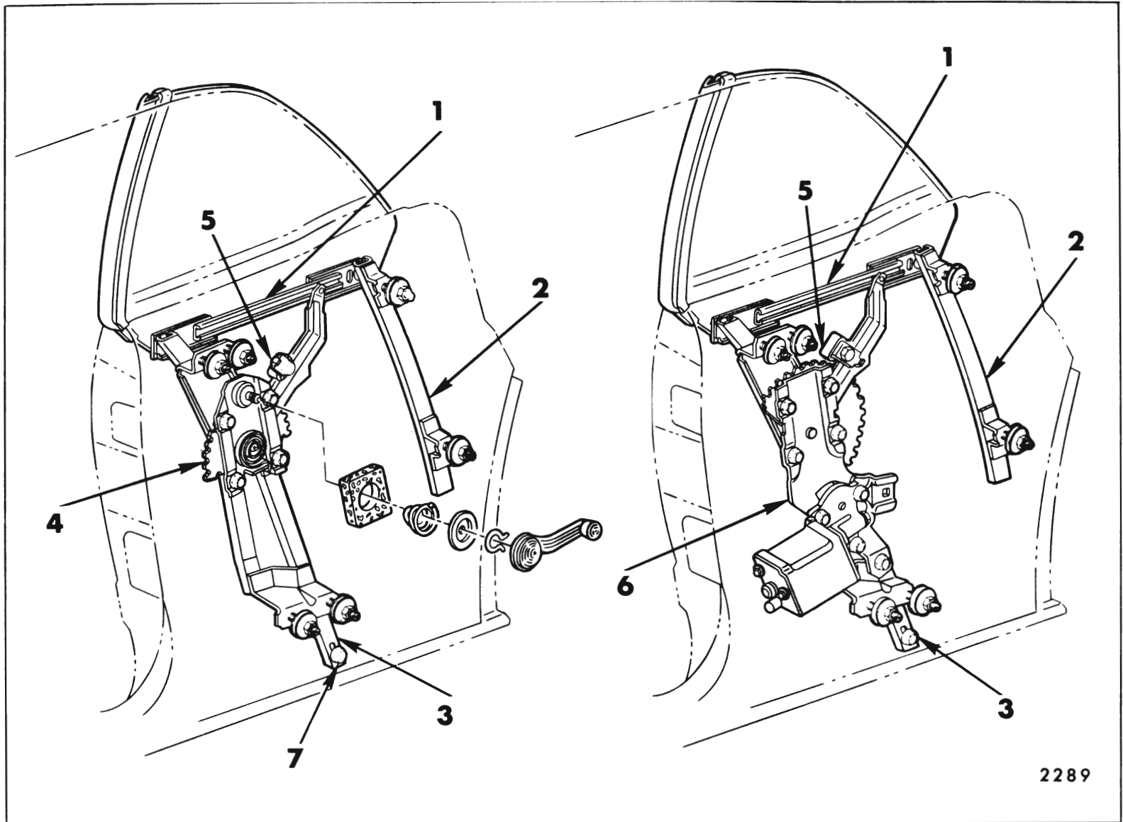
Fig. 8-32—Rear Quarter Hardware - "A-67" Styles
