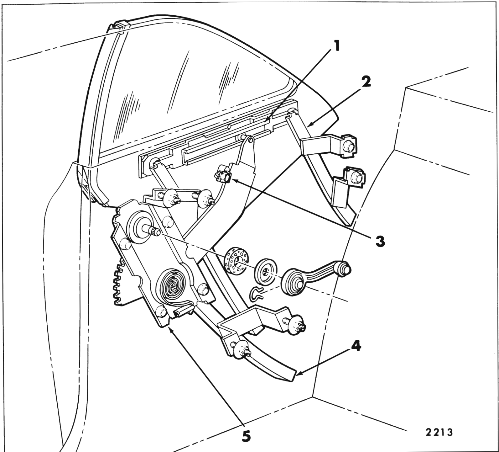
Fig. 8-36—Rear Quarter Hardware - "X-37" Styles
