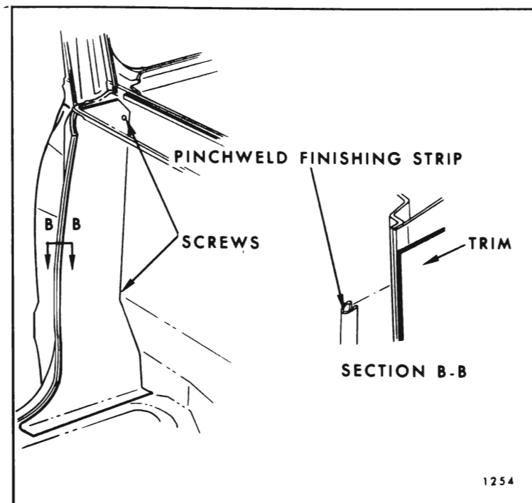
Fig. 8-7—Rear Quarter Trim Assembly - "A-80" Styles
