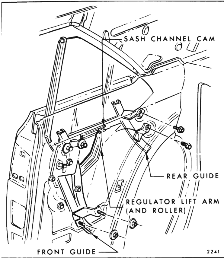
Fig. 8-56—Rear Quarter Hardware - "X"-37 Style
