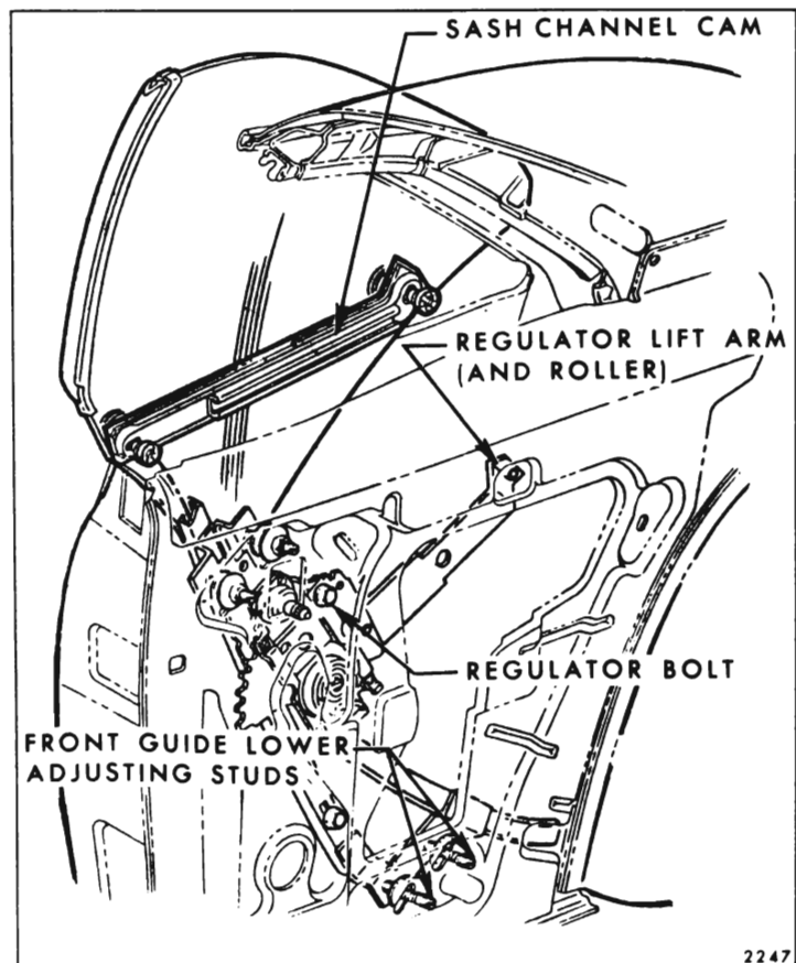
Fig. 8-53—Rear Quarter Window Removal "A-17 and 67" Styles
