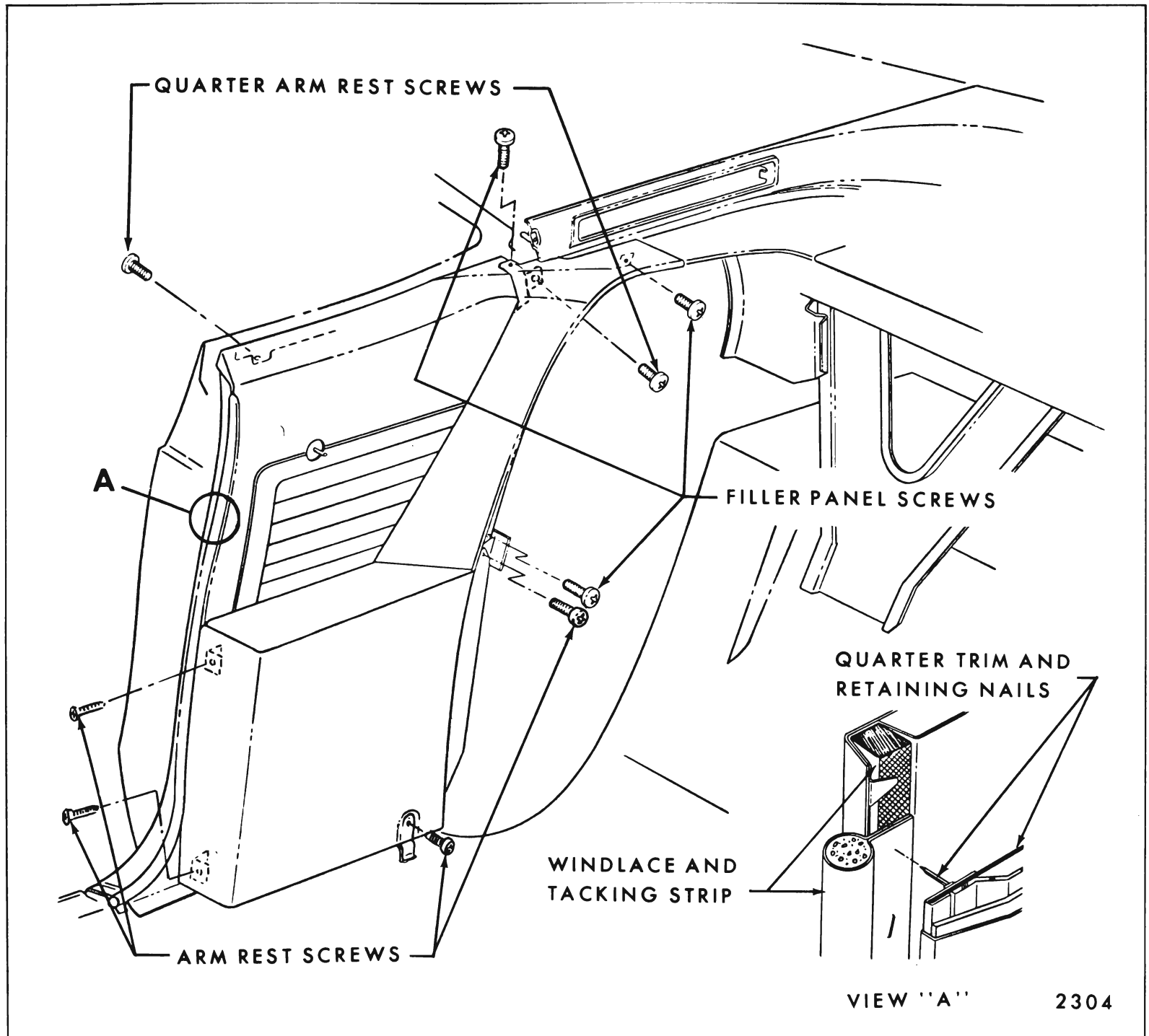
Fig. 8-10—Rear Quarter Trim Assembly - "E" Body 39487 Style
