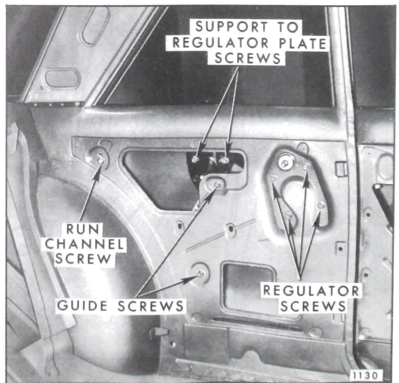
Fig. 8-42—Rear Quarter Hardware Attachment - "X-11" Style
