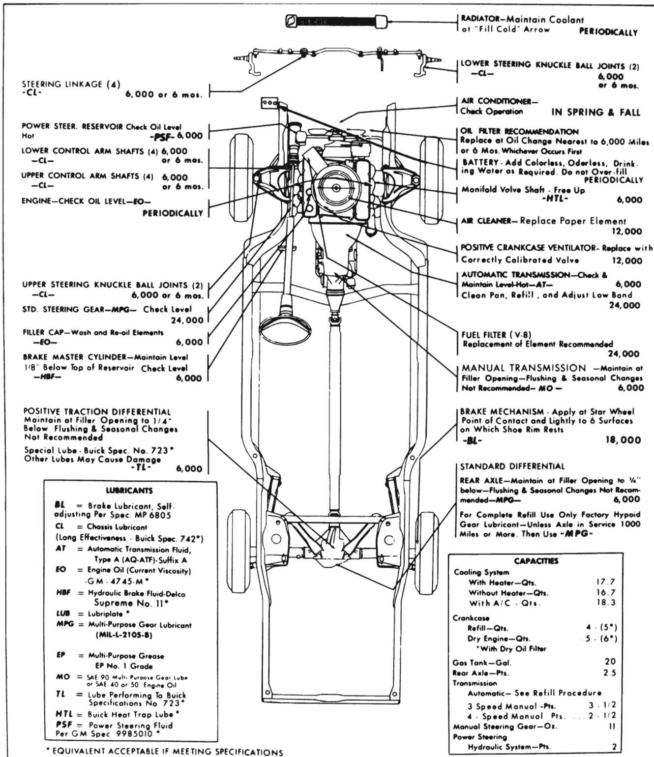
Figure 1-1—1965 Skylark Gran Sport Lubrication Chart
