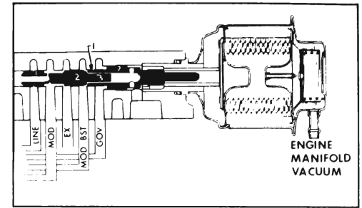
Figure 5-23—Vacuum Modulator and Valve
