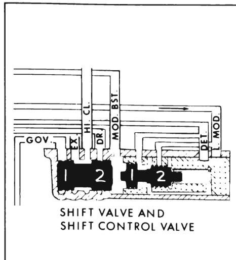
Figure 5-22—Manual Low
