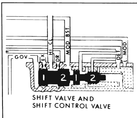
Figure 5-21—Up-Shifted
