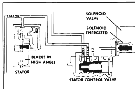
Figure 5-18—Low Angle
