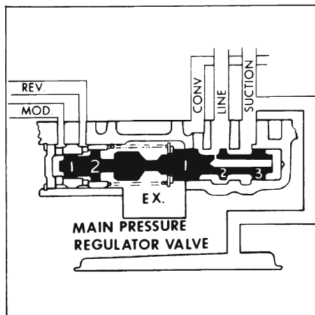
Figure 5-15—Pressure Regulator Valve (Second Stage Regulation)
