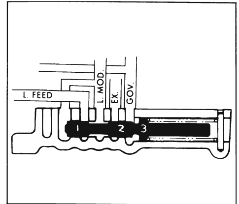
Figure 5-26—Modulator Limit Valve (Second Stage)
