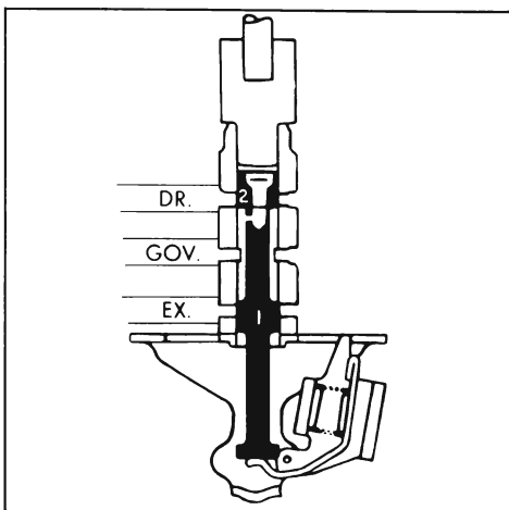
Figure 5-24—Governor Valve
