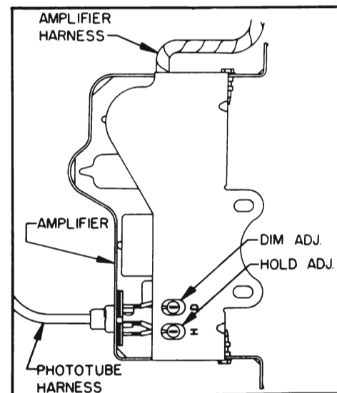
Figure 11-169—Amplifier Adjustments
