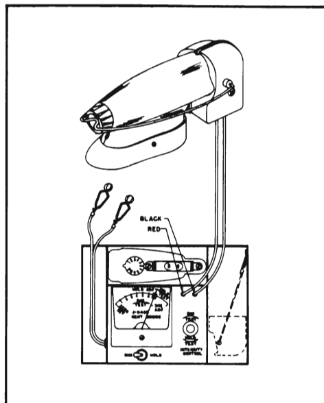
Figure 11-167—Tester J-8465
