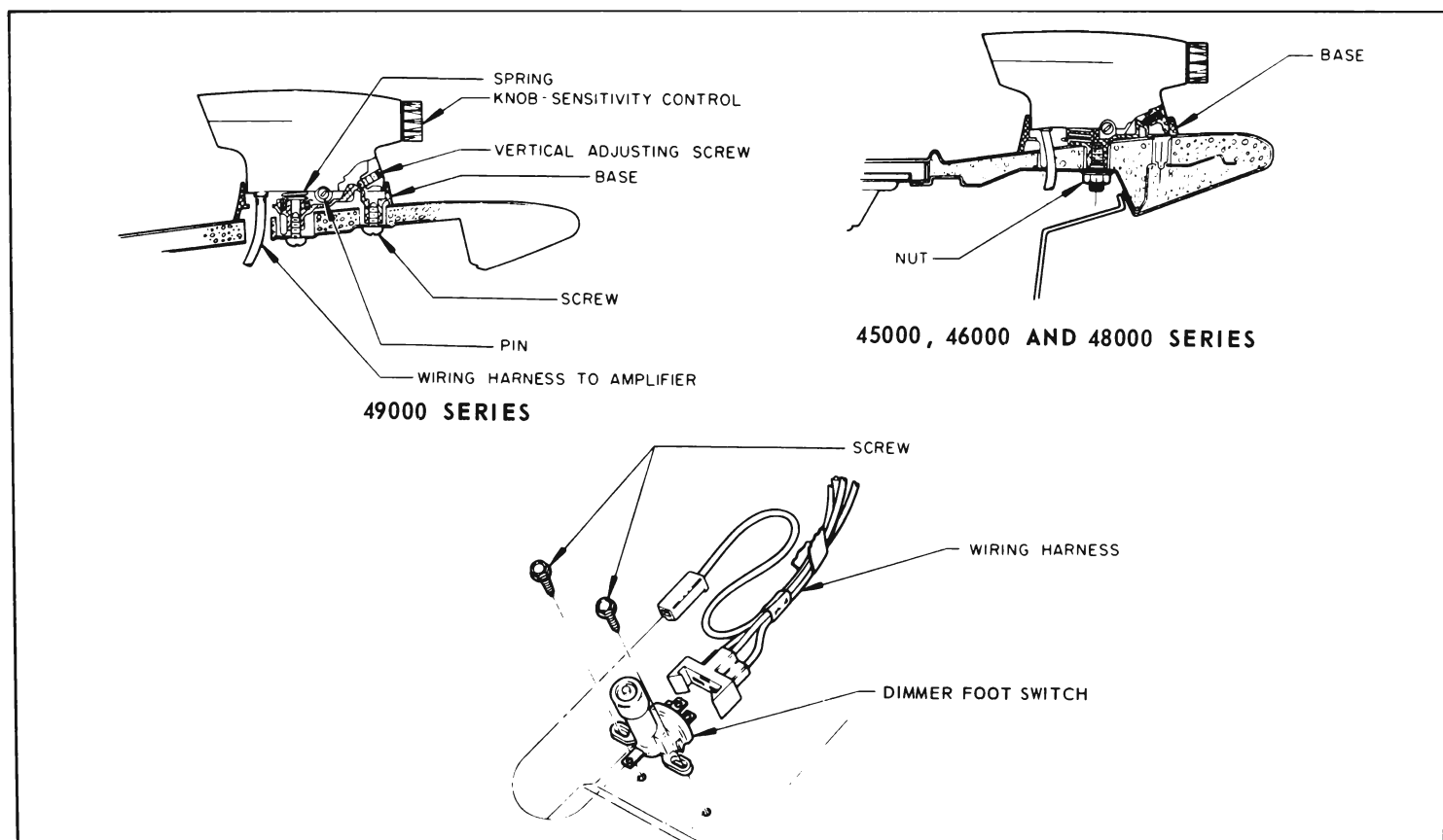
Figure 11-165—Phototube and Dimmer Switch Installation
