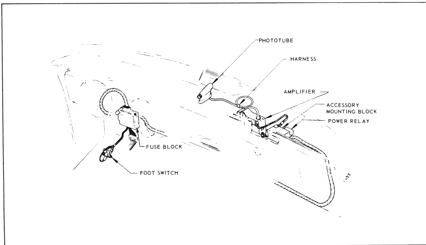
Figure 11-163—Guide-Matic Installation - 45000, 46000 and 48000 Series
