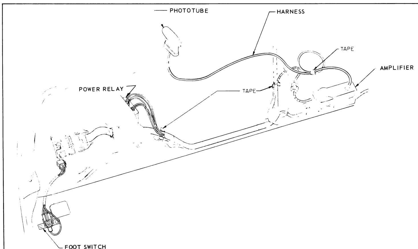
Figure 11-164—Guide-Matic Installation - 49000 Series
