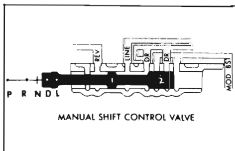
Figure 5-16—Manual Shift Control Valve
