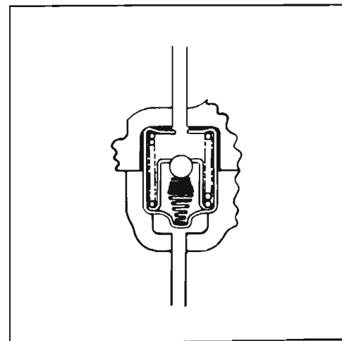
Figure 5-31—Coast Downshift Timing Valve
