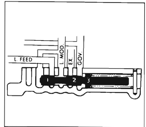
Figure 5-26—Modulator Limit Valve (Second Stage)
