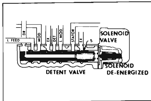
Figure 5-28—Solenoid Valve De-Energized
