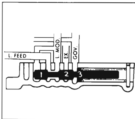
Figure 5-25—Modulator Limit Valve (First Stage)
