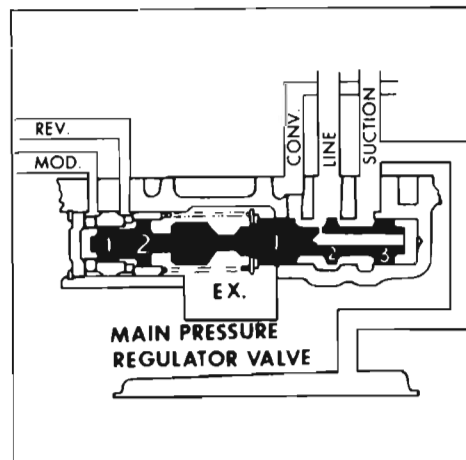
Figure 5-15—Pressure Regulator Valve (Second Stage Regulation)
