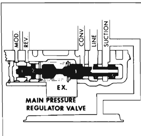
Figure 5-14—Pressure Regulator Valve (First Stage Regulation)
