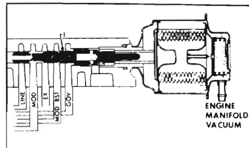
Figure 5-23—Vacuum Modulator and Valve
