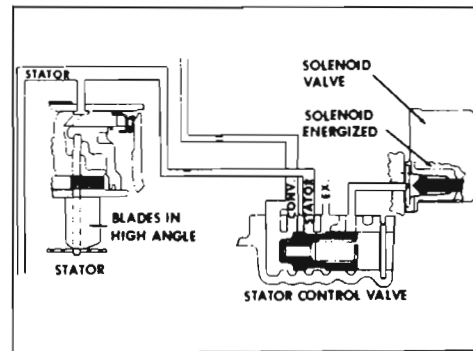
Figure 5-17—Stator Blades in High Angle
