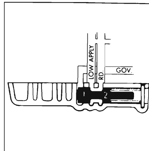
Figure 5-30—High Speed Downshift Timing Valve Regulated
