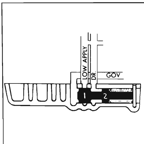
Figure 5-29—High Speed Downshift Timing Valve
