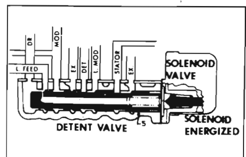
Figure 5-27—Solenoid Valve Energized
