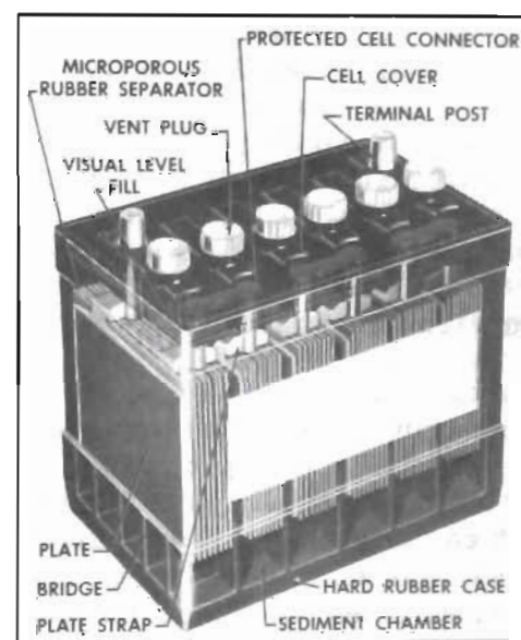
Figure 10-1—Battery
