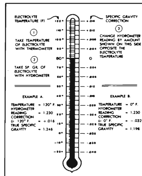
Figure 10-4—Specific Gravity Temperature Correction Scale
