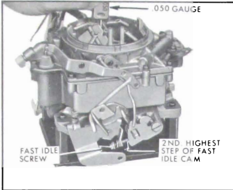
Figure 3-59—Checking Fast Idle Cam Adjustment
