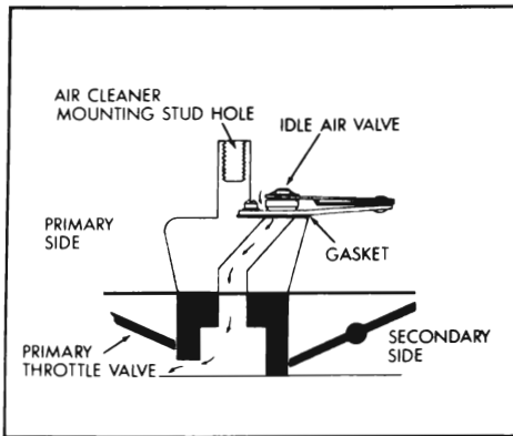
Figure 3-45—Idle Compensator
