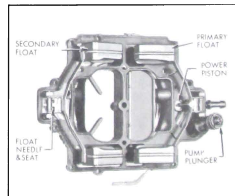
Figure 3-51—Air Horn Parts
