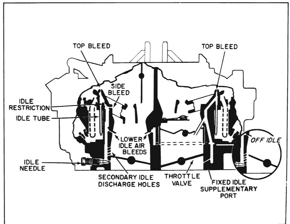
Figure 3-44—Primary and Secondary Idle Systems
