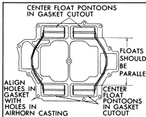
Figure 3-56—Float Alignment
