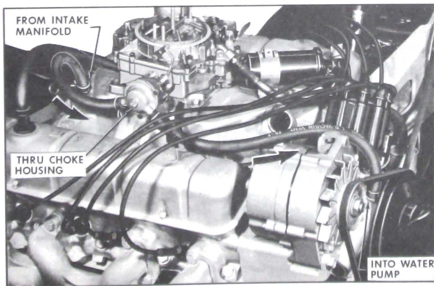
Figure 3-49—Water Heated Choke System-300 Engine
