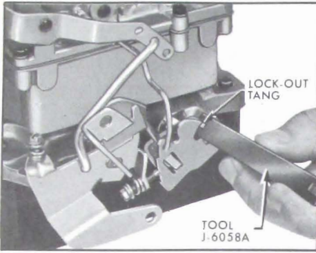
Figure 3-66—Adjusting Secondary Contour
