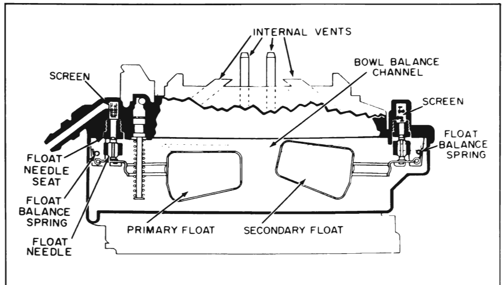
Figure 3-43—Primary and Secondary Float Systems
