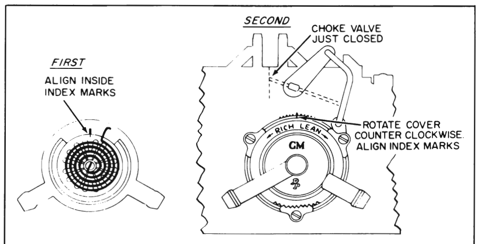
Figure 3-70—Choke Coil Adjustment - 300 Engine
