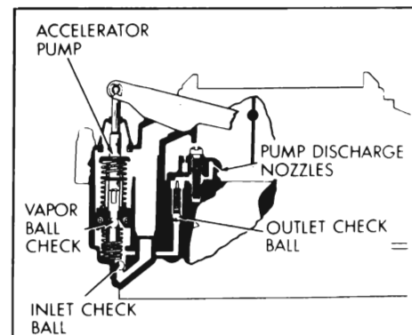
Figure 3-47—Accelerating System
