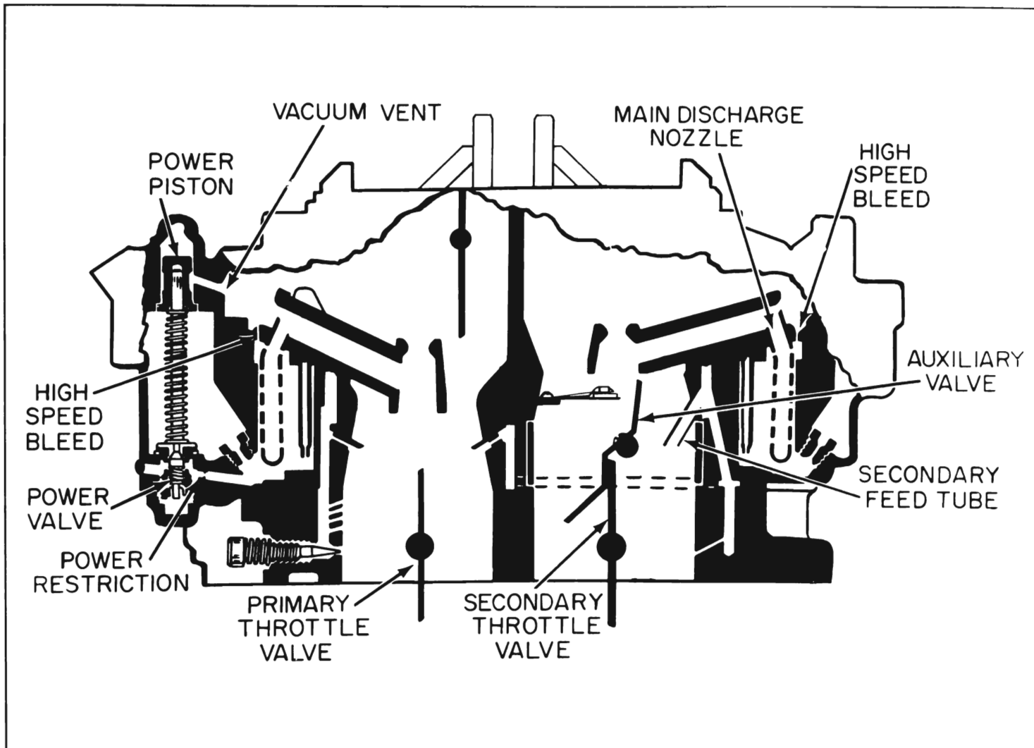
Figure 3-46—Main Metering and Power Systems
