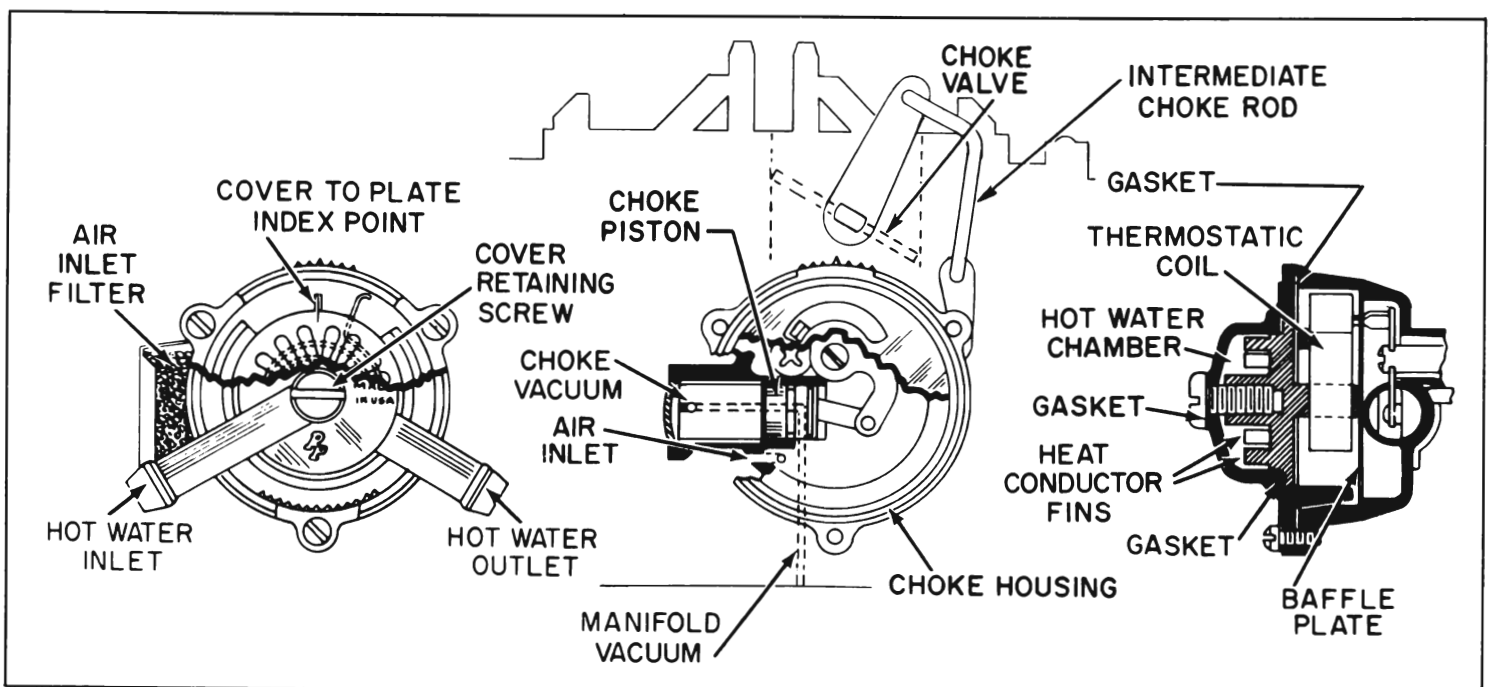
Figure 3-48—Water Heated Choke Housing—300 Engine
