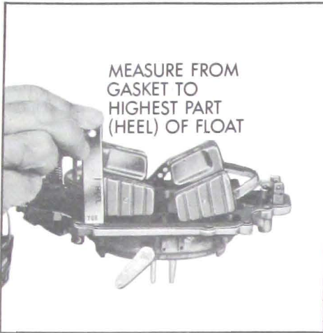
Figure 3-53—Primary Float Heel Adjustment
