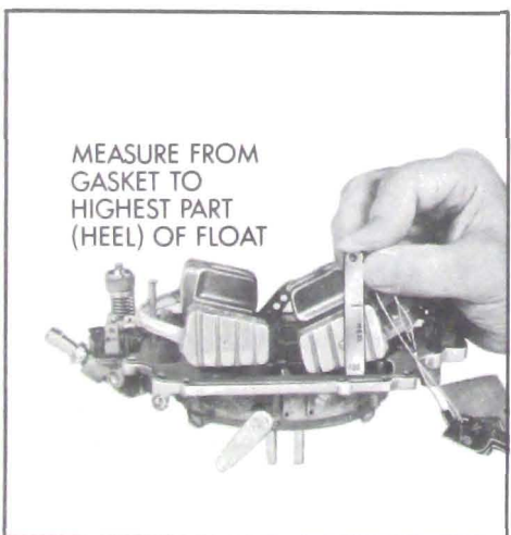
Figure 3-54—Secondary Float Heel Adjustment
