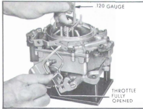
Figure 3-61—Checking Choke Unloader Adjustment
