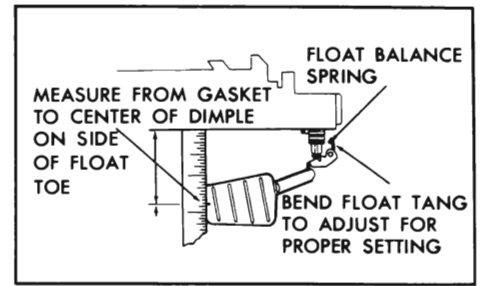
Figure 3-57—Primary Float Drop Adjustment
