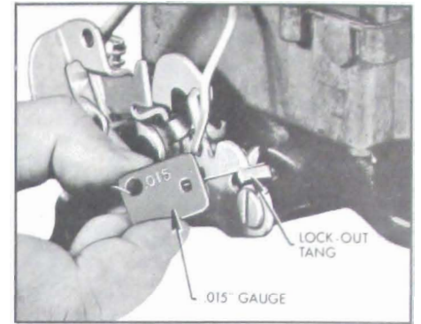
Figure 3-63—Checking Secondary Lock-Out Adjustment
