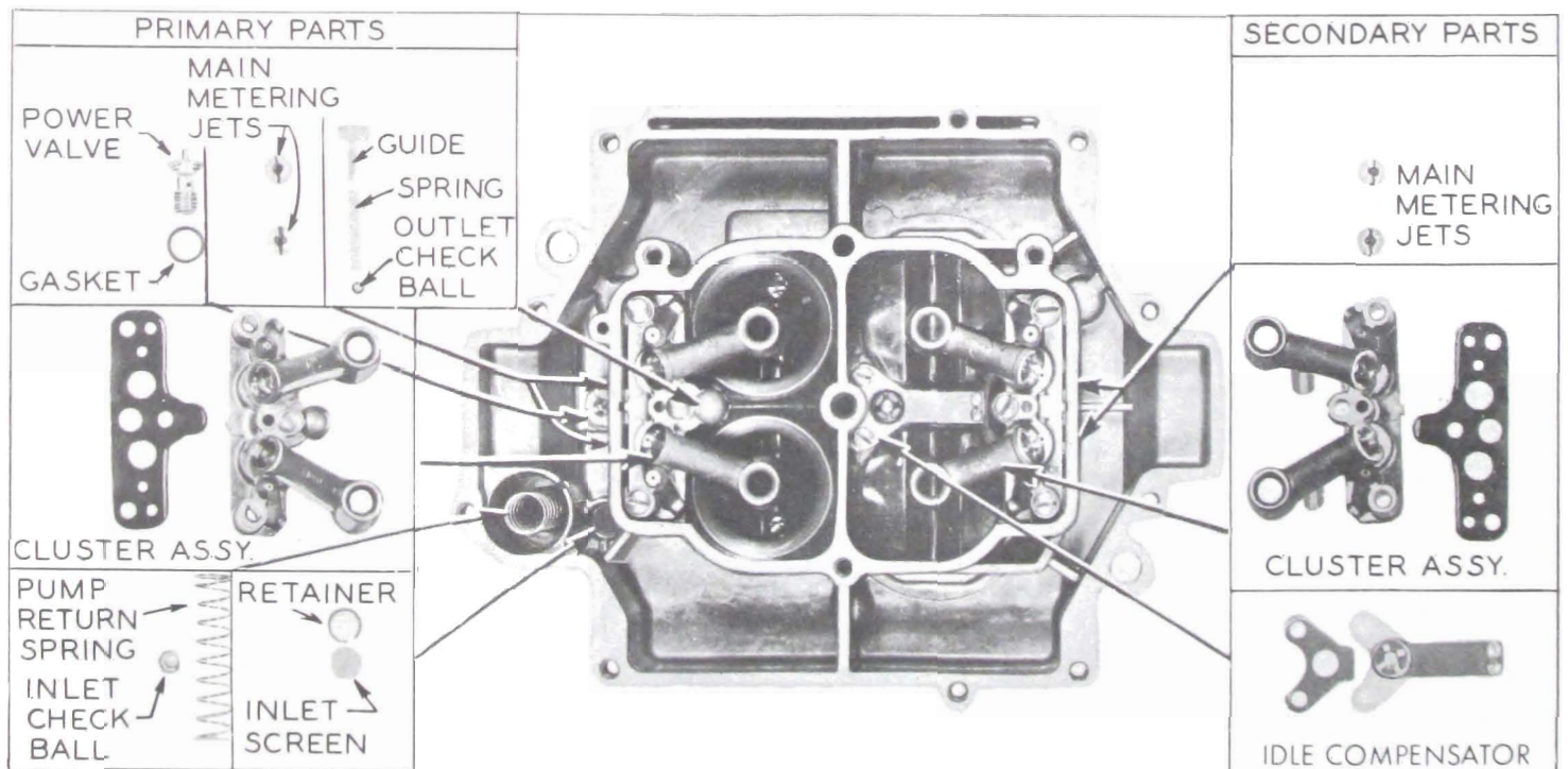
Figure 3-52—Main Body Parts
