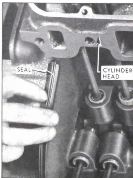
Figure 2-30—Installing Intake Manifold Seals
