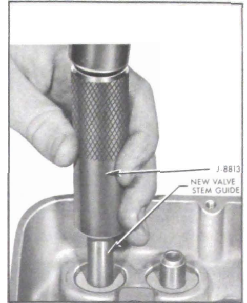
Figure 2-19—Installing New Valve Guide (V-8 only)
