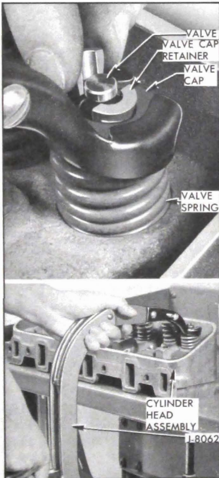
Figure 2-17—Removing and Installing Valve Cap Retainers
