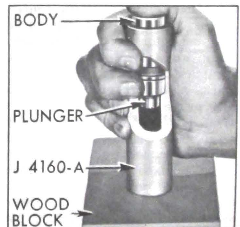
Figure 2-35—Removing Stuck Plunger with J-4160
