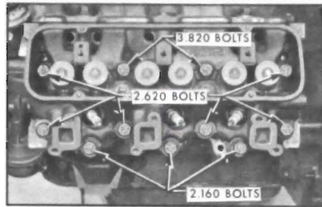
Figure 2-26—V-6 Cylinder Head Bolt Installation
