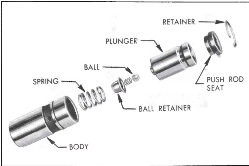
Figure 2-37—Hydraulic Valve Lifter Parts
