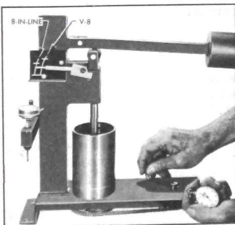
Figure 2-38—Checking Leakdown Rate
