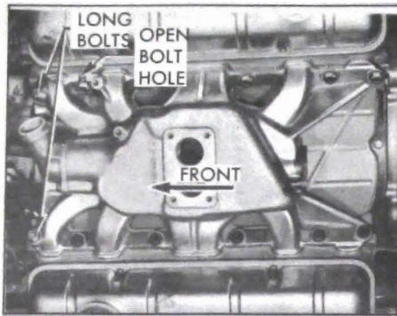
Figure 2-29—V-8 Intake Manifold Installation
