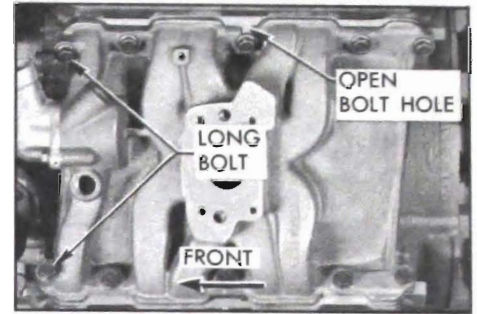
Figure 2-32—V-6 Intake Manifold Installation
