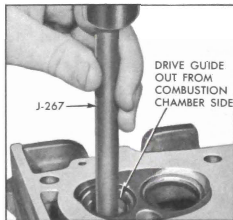
Figure 2-18—Removing Valve Stem Guide (V-8 only)
