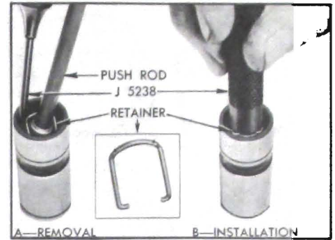
Figure 2-34—Removing and Installing Plunger Retainer
