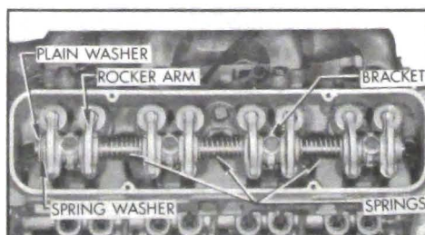
Figure 2-22—Rocker Arm Shaft Assembly (V-8 shown)
