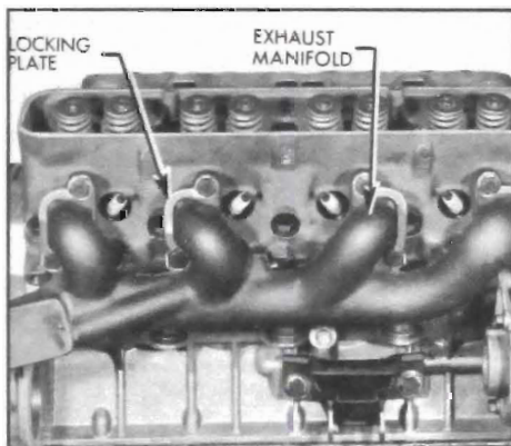
Figure 2-24—Exhaust Manifold Installation (V-8 shown)
