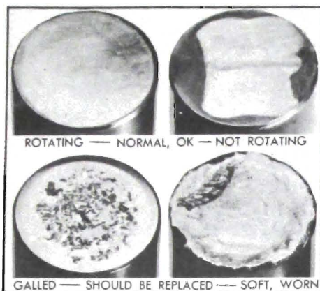
Figure 2-36—Lifter Body Wear Patterns
