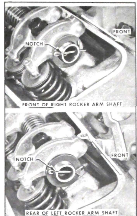
Figure 2-23—Rocker Arm Shaft Installation
