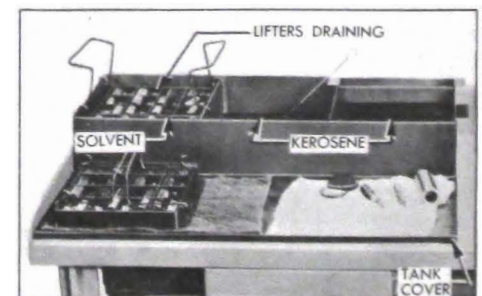
Figure 2-33—Tank J-5821 Set Up for Cleaning Lifter Parts
