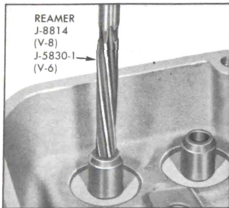
Figure 2-20—Reaming Valve Guide
