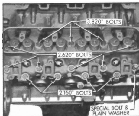
Figure 2-25—V-8 Cylinder Head Bolt Installation
