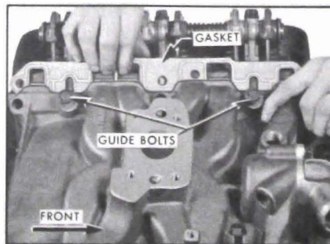
Figure 2-31—Installing V-6 Intake Manifold Gasket
