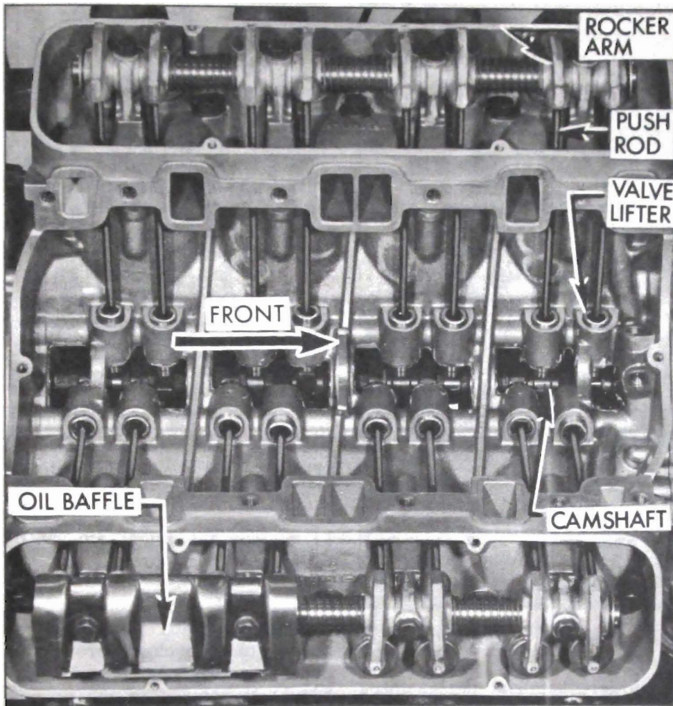
Figure 2-8—V-8 Valve Mechanism
