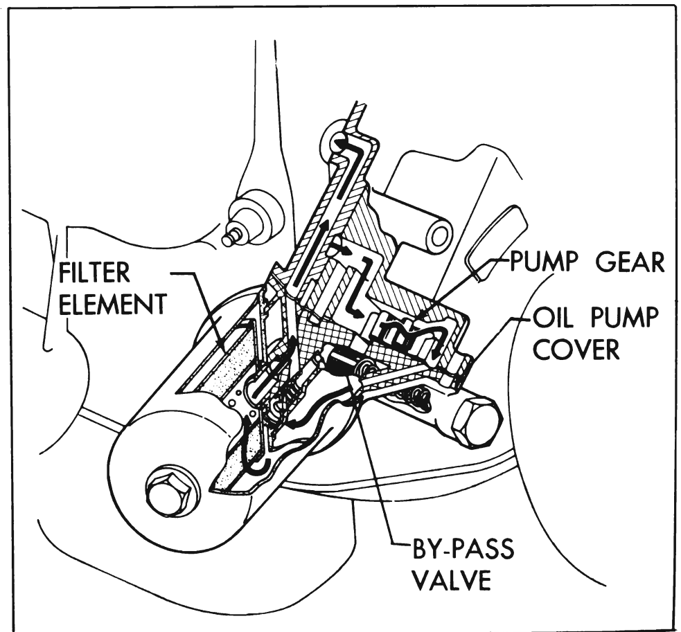
Figure 2-12—Oil Flow Through Filter
