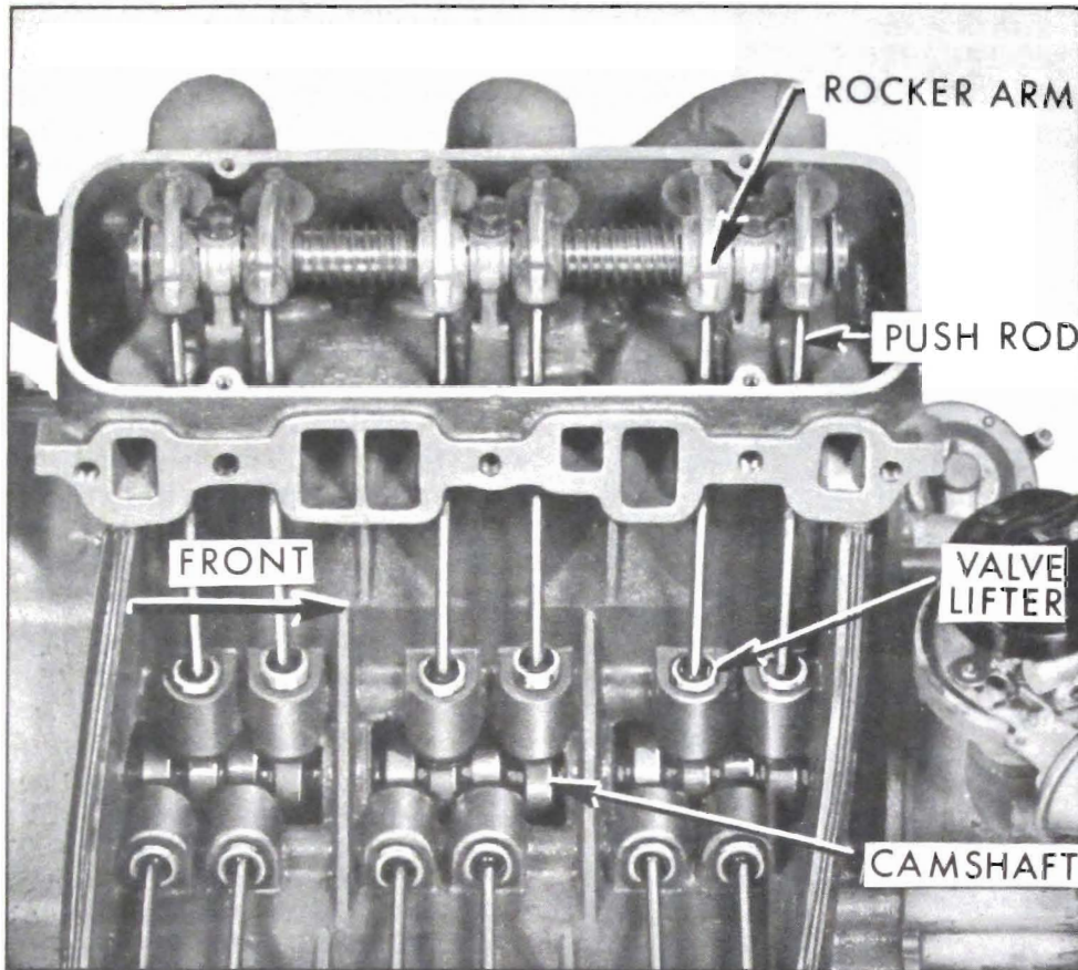
Figure 2-9—V-6 Valve Mechanism
