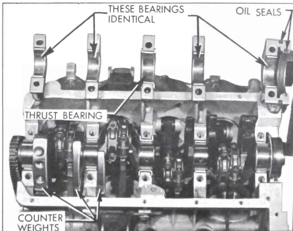
Figure 2-4—V-8 Engine Crankshaft and Bearings
