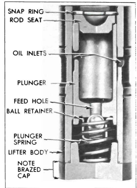
Figure 2-11—Hydraulic Valve Lifter, Sectional View
