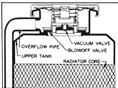
Figure 2-13—Radiator Cap
