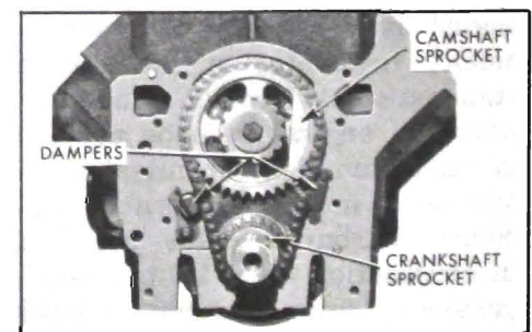
Figure 2-7—V-6 Timing Chain Installation
