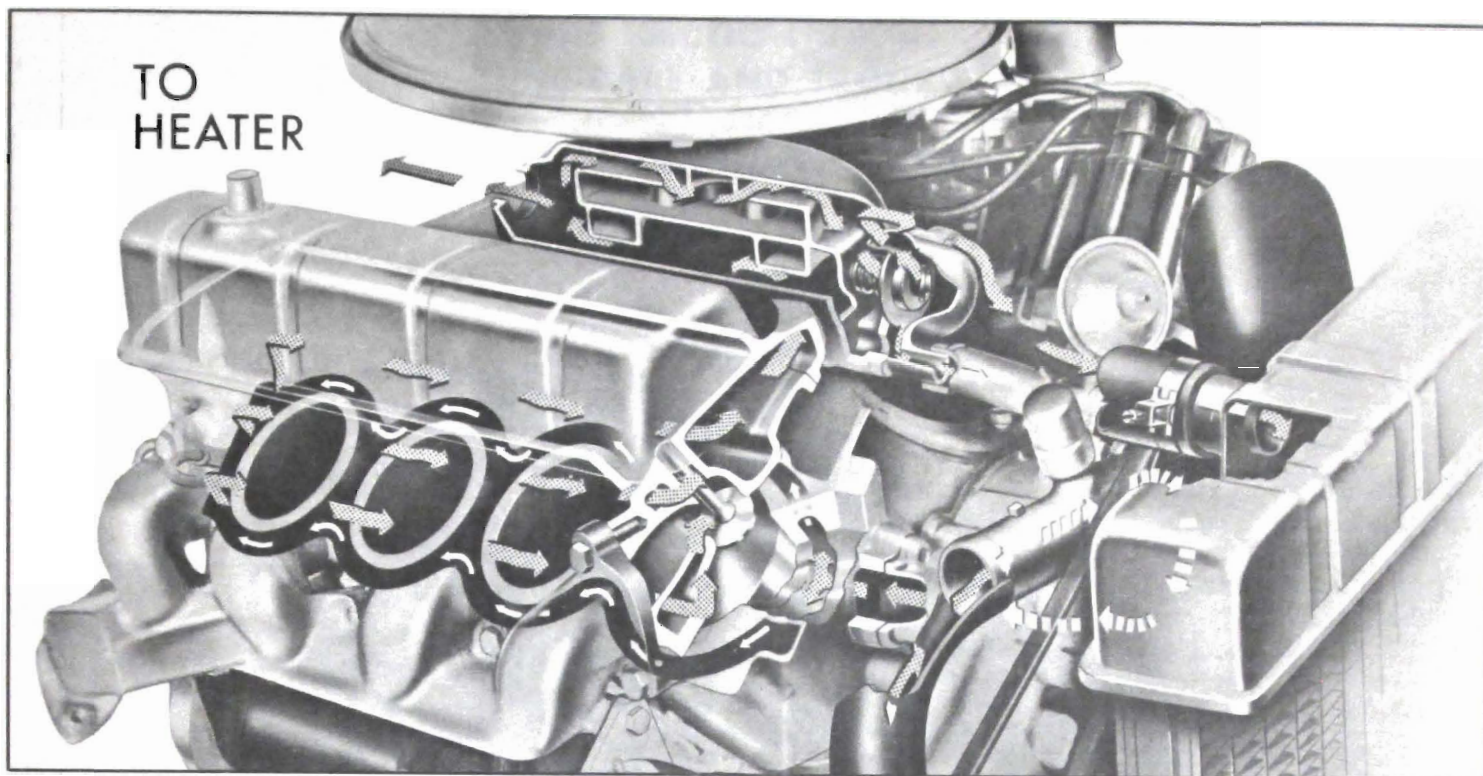
Figure 2-15—V-8 Engine Coolant Flow cylinder bank water jacket. See Figures 2-15 and 2-16.
