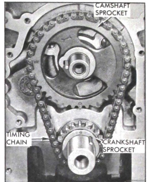
Figure 2-6—V-8 Timing Chain and Sprockets
