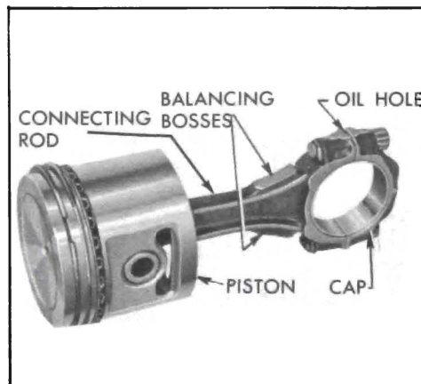
Figure 2-5—Connecting Rod and Piston Assembly
