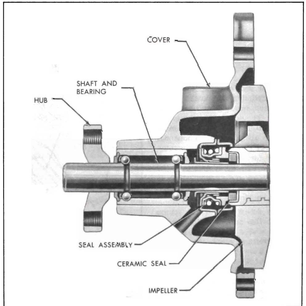
Figure 2-14—Water Pump
