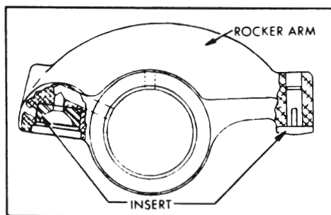
Figure 2-10—Valve Rocker Arm
