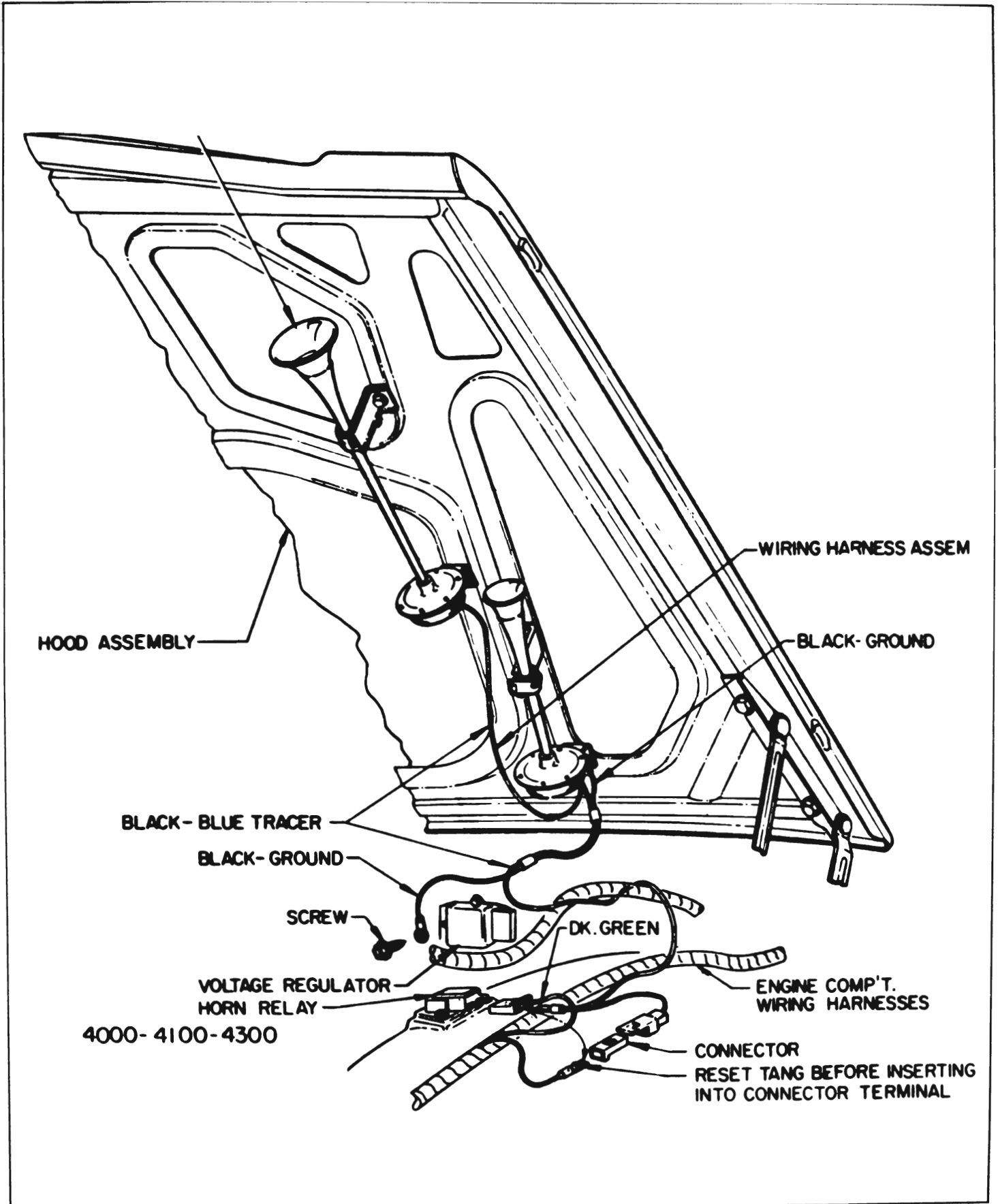
Figure 11-125—Four Note Horn Installation
