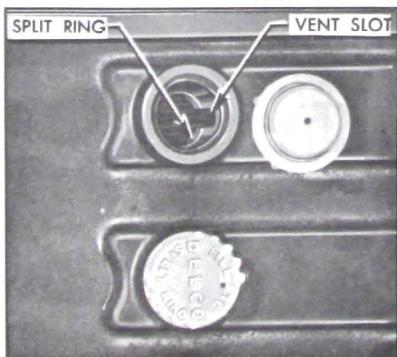
Figure 10-2—Battery Filler Well
