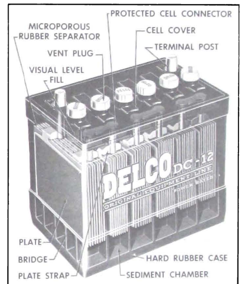
Figure 10-1—Battery
