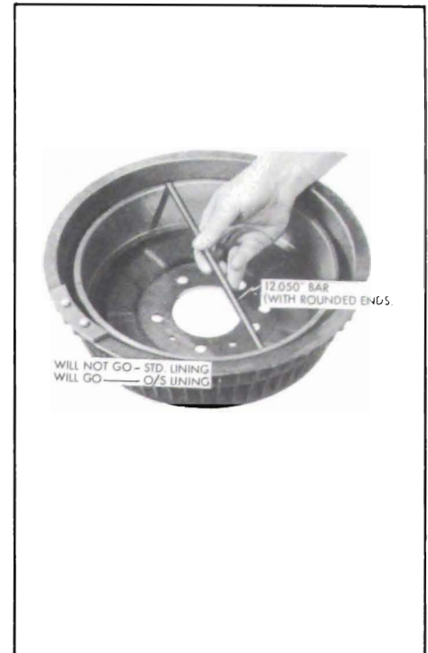
Figure 9-12—Measuring Brake Drum Size
