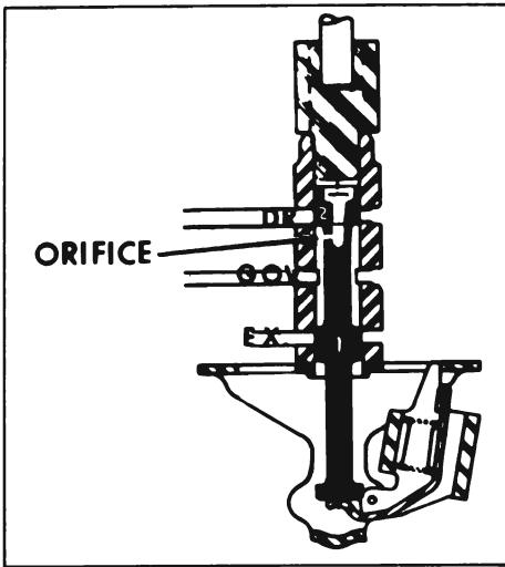
Figure 5-24—Governor Valve
