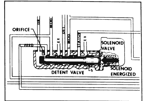
Figure 5-27—Solenoid Valve Energized
